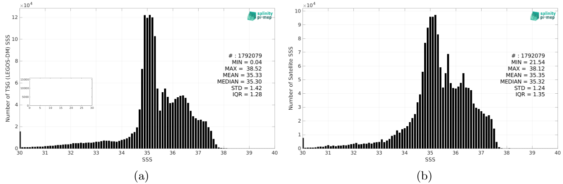
Figure 2: Histograms of SSS from TSG (LEGOS-DM) (a) and CCI SSS L4 Merged-OI v3.2 - 30-day running (ESA) (b) considering all match-up pairs per bins of 0.1 over the Atlantic Ocean Pi-MEP region and for the full satellite product period.
