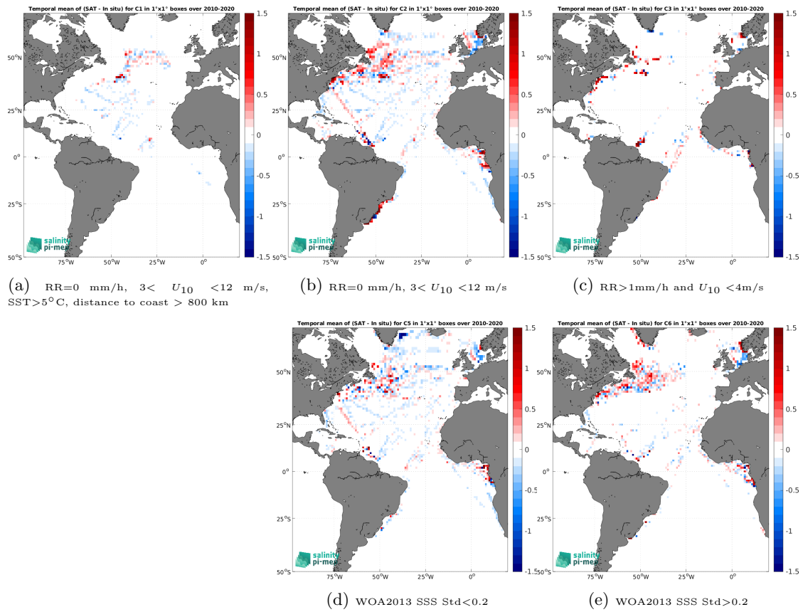
Figure 12: Temporal mean gridded over spatial boxes of size 1^\circ \times 1^\circ of \Delta\text{SSS} (CCI SSS L4 Merged-OI v3.2 - 30-day running (ESA) - TSG (LEGOS-DM)) for 5 different subdatasets corresponding to:RR=0 mm/h, 3 < U_{10} < 12 m/s, SST >5^\circ\text{C} , distance to coast > 800 km (a), RR=0 mm/h, 3 < U_{10} < 12 m/s (b), RR >1 mm/h and U_{10} < 4 m/s (c), WOA2013 SSS Std <0.2 (d), WOA2013 SSS Std >0.2 (e).
