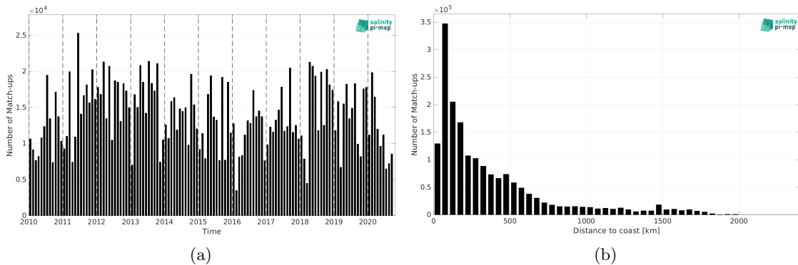
Figure 1: Number of match-ups between TSG (LEGOS-DM) and CCI SSS L4 Merged-OI v3.2 - 30-day running (ESA) SSS as a function of time (a) and as function of the distance to coast (b) over the Atlantic Ocean Pi-MEP region and for the full satellite product period.
