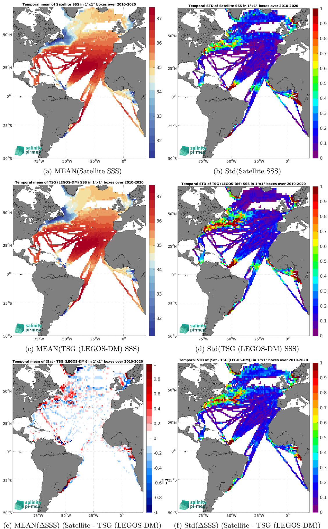
Figure 6: Temporal mean (left) and Std (right) of SSS from CCI SSS L4 Merged-OI v3.2 - 30-day running (ESA) (top), TSG (LEGOS-DM) (middle), and of \Delta SSS (Satellite - TSG (LEGOS-DM)). Only match-up pairs are used to generate these maps.
