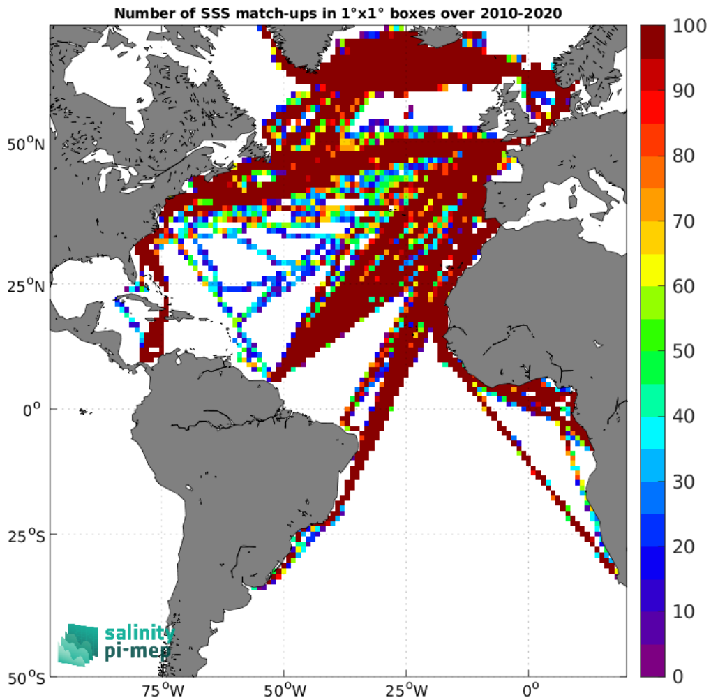
Figure 4: Number of SSS match-ups between TSG (LEGOS-DM) SSS and the CCI SSS L4 Merged-OI v3.2 - 30-day running (ESA) SSS product for the Atlantic Ocean Pi-MEP region over 1^\circ \times 1^\circ boxes and for the full satellite product period.
