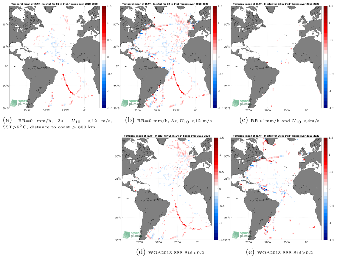
Figure 12: Temporal mean gridded over spatial boxes of size 1^\circ \times 1^\circ of \Delta SSS (CCI SSS L4 Merged-OI v3.2 - 30-day running (ESA) - TSG (GOSUD-Sailing-ship)) for 5 different subdatasets corresponding to:RR=0 mm/h, 3 < U_{10} < 12 m/s, SST>5°C, distance to coast > 800 km (a), RR=0 mm/h, 3 < U_{10} < 12 m/s (b), RR>1mm/h and U_{10} < 4 m/s (c), WOA2013 SSS Std<0.2 (d), WOA2013 SSS Std>0.2 (e).
