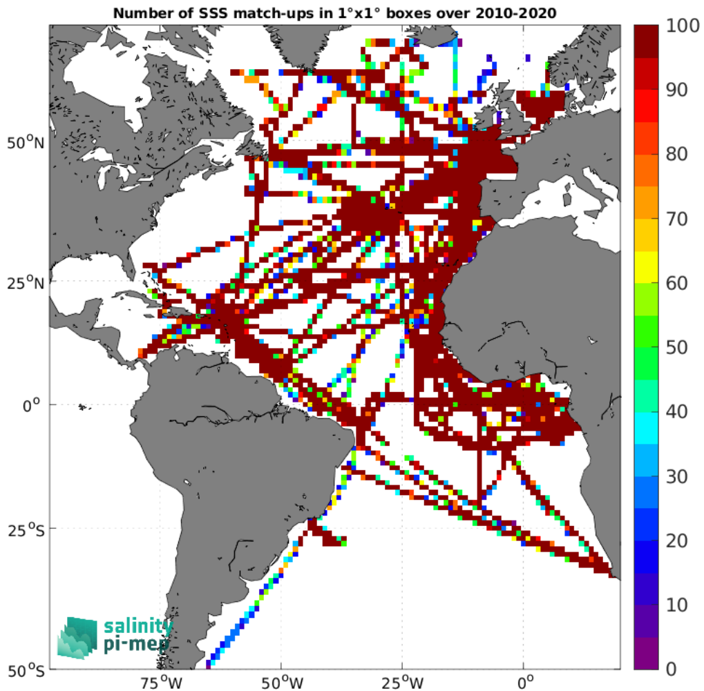
Figure 4: Number of SSS match-ups between TSG (GOSUD-Research-vessel) SSS and the CCI SSS L4 Merged-OI v3.2 - 30-day running (ESA) SSS product for the Atlantic Ocean Pi-MEP region over 1^{\circ} \times 1^{\circ} boxes and for the full satellite product period.
