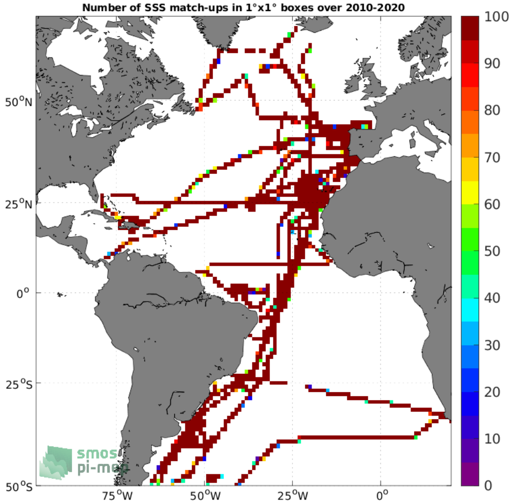
Figure 4: Number of SSS match-ups between TSG (CSIC-UTM) SSS and the CCI SSS L4 Merged-OI v3.2 - 30-day running (ESA) SSS product for the Atlantic Ocean Pi-MEP region over 1^\circ \times 1^\circ boxes and for the full satellite product period.
