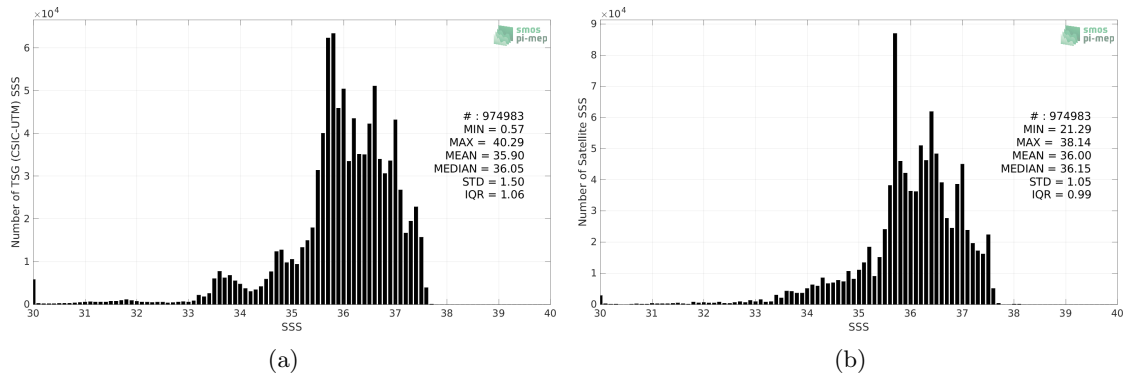
Figure 2: Histograms of SSS from TSG (CSIC-UTM) (a) and CCI SSS L4 Merged-OI v3.2 - 30-day running (ESA) (b) considering all match-up pairs per bins of 0.1 over the Atlantic Ocean Pi-MEP region and for the full satellite product period.
