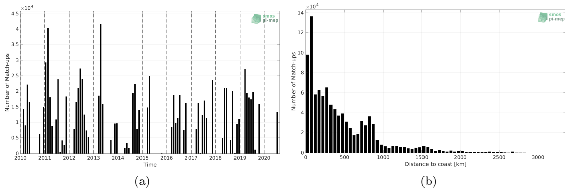
Figure 1: Number of match-ups between TSG (CSIC-UTM) and CCI SSS L4 Merged-OI v3.2 - 30-day running (ESA) SSS as a function of time (a) and as function of the distance to coast (b) over the Atlantic Ocean Pi-MEP region and for the full satellite product period.
