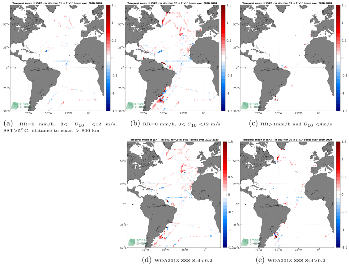
Figure 12: Temporal mean gridded over spatial boxes of size 1^\circ \times 1^\circ of \Delta SSS (CCI SSS L4 Merged-OI v3.2 - 30-day running (ESA) - TSG (CSIC-UTM)) for 5 different subdatasets corresponding to:RR=0 mm/h, 3 < U_{10} < 12 m/s, SST >5^\circ\text{C} , distance to coast > 800 km (a), RR=0 mm/h, 3 < U_{10} < 12 m/s (b), RR >1 mm/h and U_{10} < 4 m/s (c), WOA2013 SSS Std <0.2 (d), WOA2013 SSS Std >0.2 (e).
