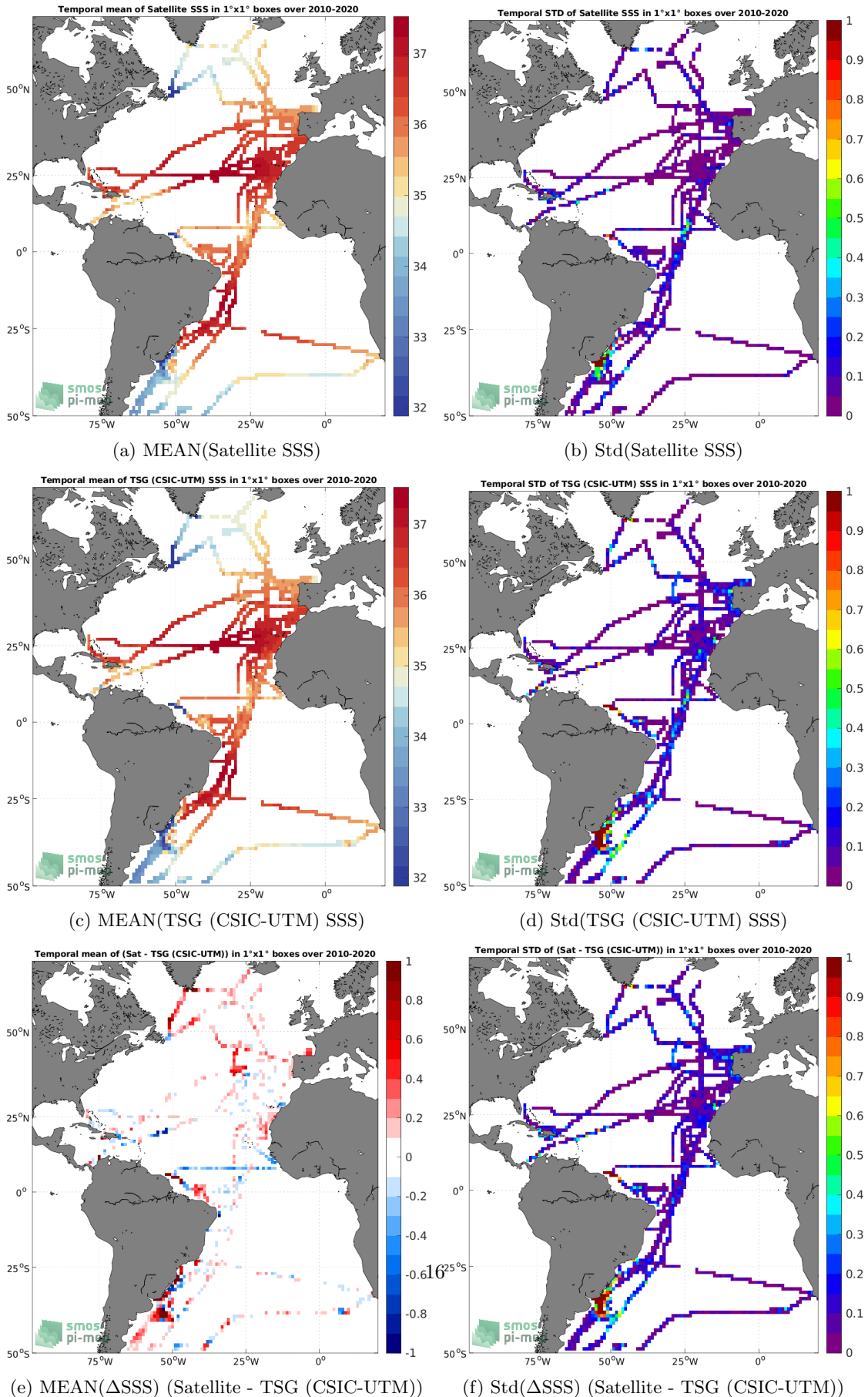
Figure 6: Temporal mean (left) and Std (right) of SSS from CCI SSS L4 Merged-OI v3.2 - 30-day running (ESA) (top), TSG (CSIC-UTM) (middle), and of \Delta SSS (Satellite - TSG (CSIC-UTM)). Only match-up pairs are used to generate these maps.
