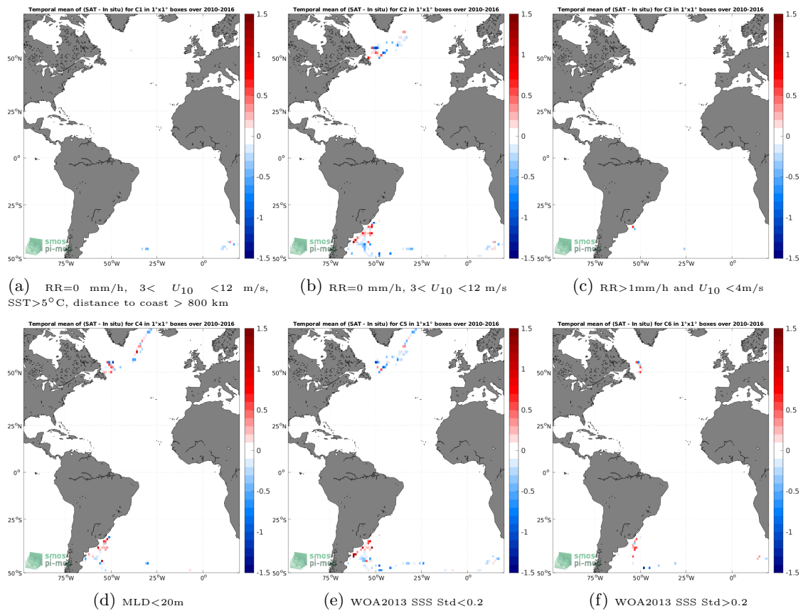
Figure 12: Temporal mean gridded over spatial boxes of size 1^\circ \times 1^\circ of \Delta SSS (CCI SSS L4 Merged-OI v3.2 - 30-day running (ESA) - Marine mammals) for 6 different subdatasets corresponding to:RR=0 mm/h, 3 < U_{10} < 12 m/s, SST>5°C, distance to coast > 800 km (a), RR=0 mm/h, 3 < U_{10} < 12 m/s (b), RR>1mm/h and U_{10} < 4 m/s (c),MLD<20m (d),WOA2013 SSS Std<0.2 (e),WOA2013 SSS Std>0.2 (f).
