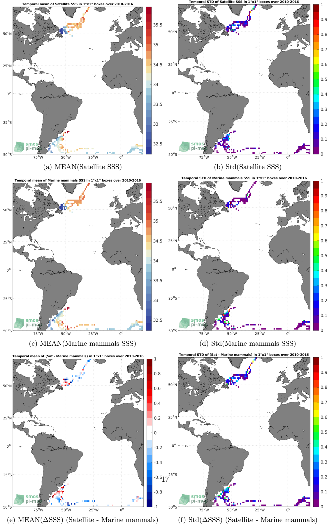
Figure 6: Temporal mean (left) and Std (right) of SSS from CCI SSS L4 Merged-OI v3.2 - 30-day running (ESA) (top), Marine mammals (middle), and of \Delta SSS (Satellite - Marine mammals). Only match-up pairs are used to generate these maps.
