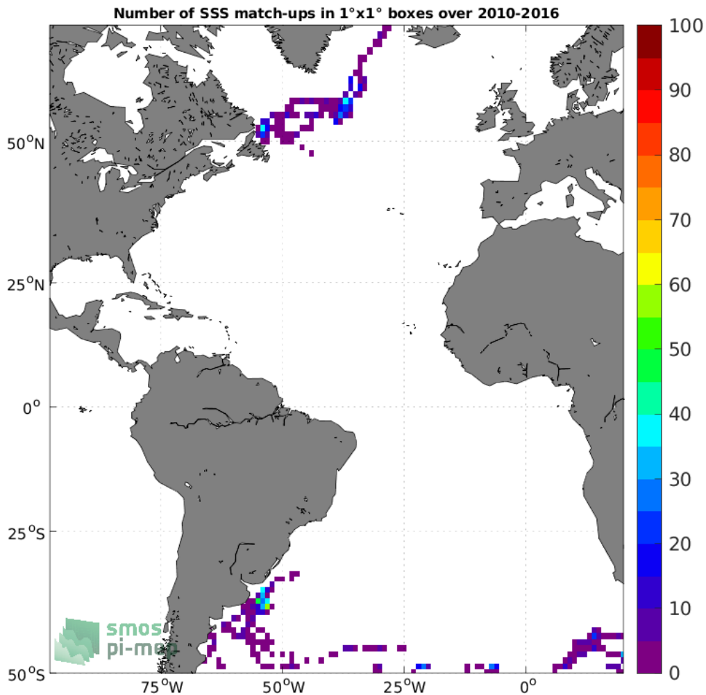
Figure 4: Number of SSS match-ups between Marine mammals SSS and the CCI SSS L4 Merged-OI v3.2 - 30-day running (ESA) SSS product for the Atlantic Ocean Pi-MEP region over 1°x1° boxes and for the full satellite product period.
