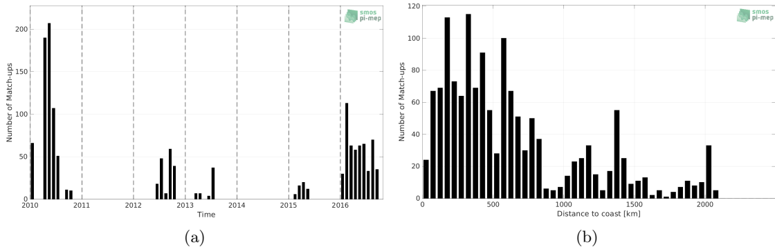
Figure 1: Number of match-ups between Marine mammals and CCI SSS L4 Merged-OI v3.2 - 30-day running (ESA) SSS as a function of time (a) and as function of the distance to coast (b) over the Atlantic Ocean Pi-MEP region and for the full satellite product period.
