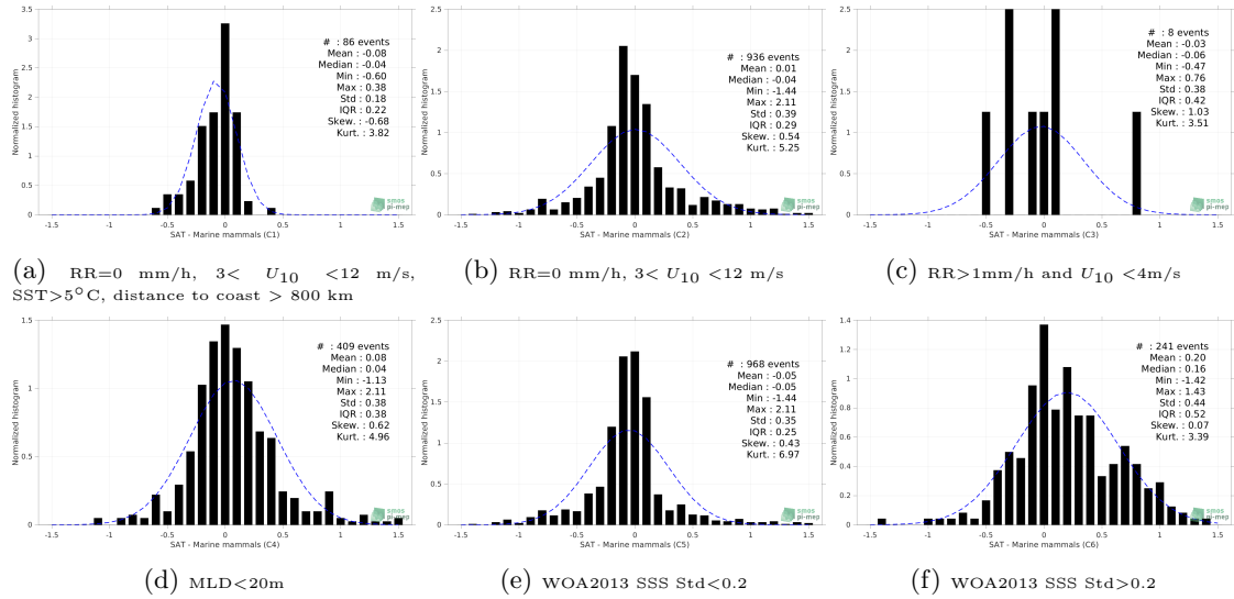
Figure 13: Normalized histogram of \Delta\text{SSS} (CCI SSS L4 Merged-OI v3.2 - 30-day running (ESA) - Marine mammals) for 6 different subdatasets corresponding to: RR=0 mm/h, 3 < U_{10} < 12 m/s, SST>5°C, distance to coast > 800 km (a), RR=0 mm/h, 3 < U_{10} < 12 m/s (b), RR>1mm/h and U_{10} < 4 m/s (c), MLD<20m (d), WOA2013 SSS Std<0.2 (e), WOA2013 SSS Std>0.2 (f).
