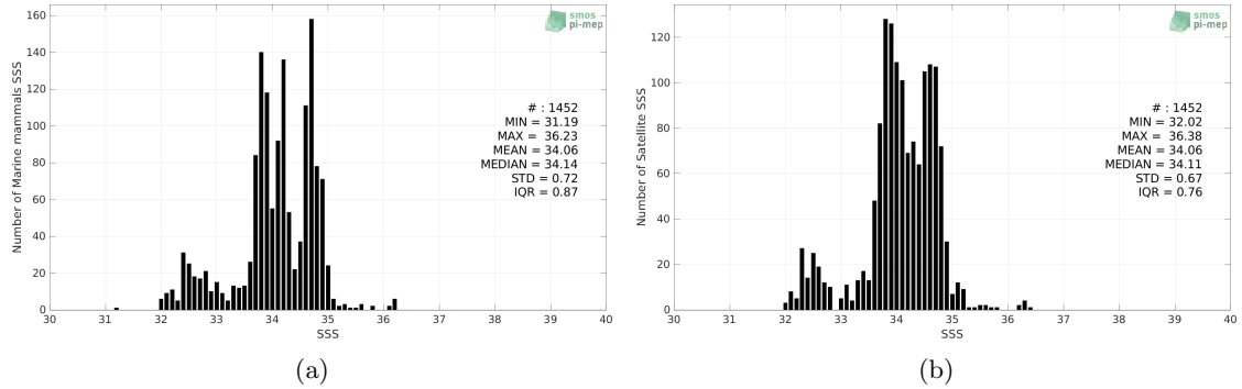
Figure 2: Histograms of SSS from Marine mammals (a) and CCI SSS L4 Merged-OI v3.2 - 30-day running (ESA) (b) considering all match-up pairs per bins of 0.1 over the Atlantic Ocean Pi-MEP region and for the full satellite product period.
