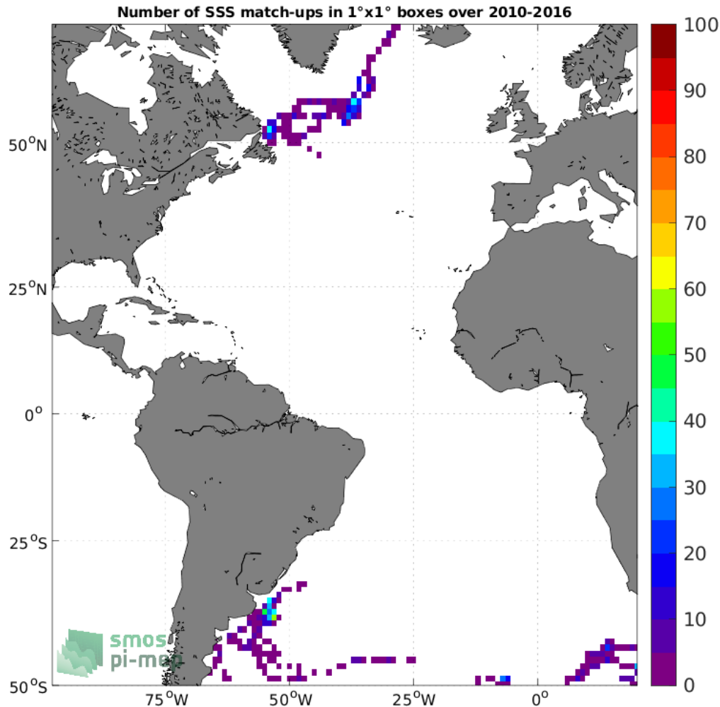
Figure 4: Number of SSS match-ups between Marine mammals SSS and the CCI SSS L4 Merged-OI v3.2 - 30-day running (ESA) SSS product for the Atlantic Ocean Pi-MEP region over 1^\circ \times 1^\circ boxes and for the full satellite product period.
