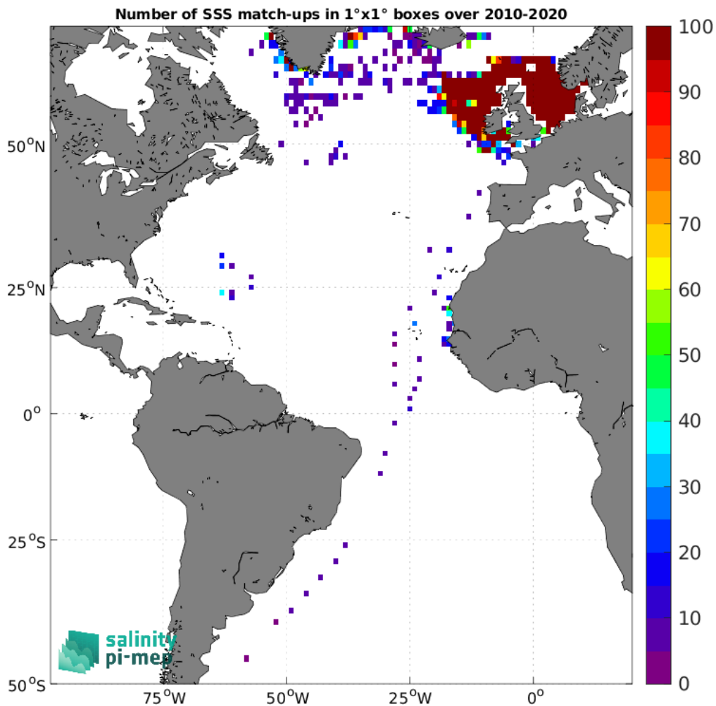
Figure 4: Number of SSS match-ups between ICES SSS and the CCI SSS L4 Merged-OI v3.2 - 30-day running (ESA) SSS product for the Atlantic Ocean Pi-MEP region over 1°x1° boxes and for the full satellite product period.
