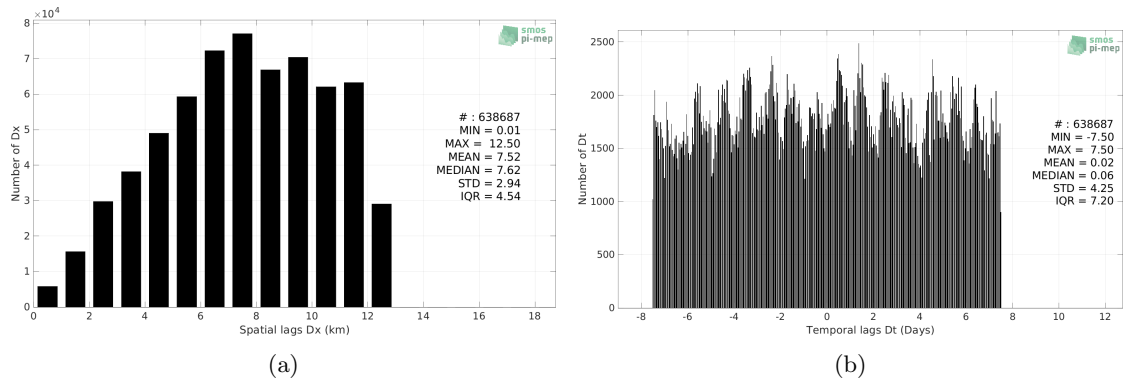
Figure 5: Histograms of the spatial (a) and temporal (b) lags between the location/time of the ICES measurement and the date of the corresponding CCI SSS L4 Merged-OI v3.2 - 30-day running (ESA) SSS pixel.
