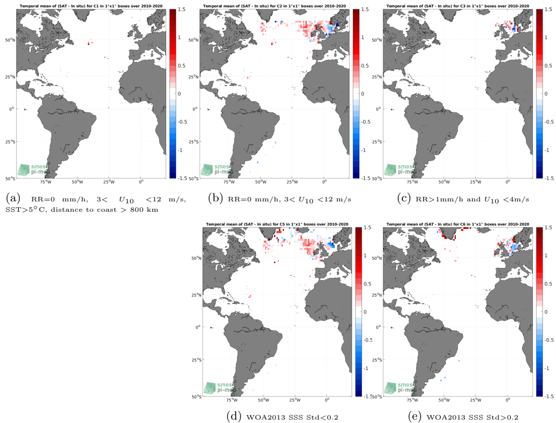
Figure 12: Temporal mean gridded over spatial boxes of size 1^\circ \times 1^\circ of \Delta SSS (CCI SSS L4 Merged-OI v3.2 - 30-day running (ESA) - ICES) for 5 different subdatasets corresponding to:RR=0 mm/h, 3 < U_{10} < 12 m/s, SST >5^\circ\text{C} , distance to coast > 800 km (a), RR=0 mm/h, 3 < U_{10} < 12 m/s (b), RR >1 mm/h and U_{10} < 4 m/s (c), WOA2013 SSS Std <0.2 (d), WOA2013 SSS Std >0.2 (e).
