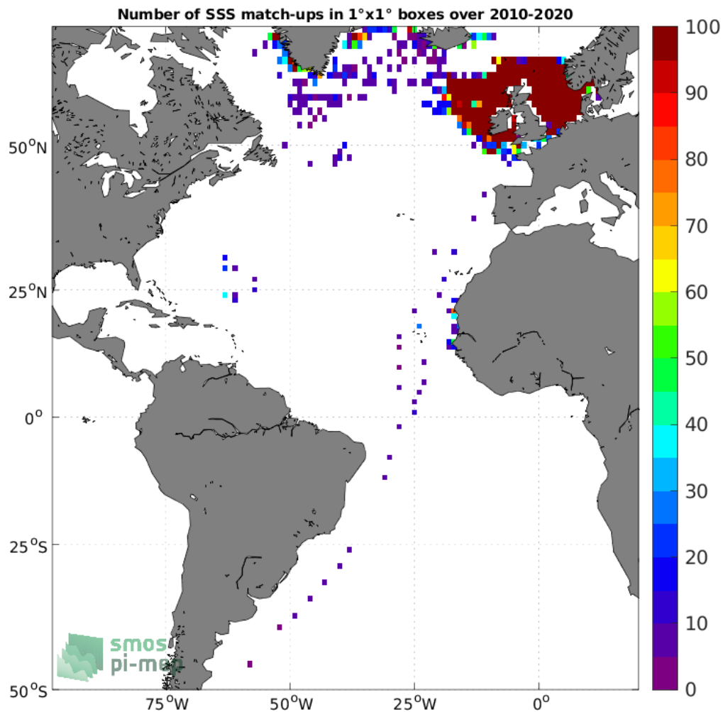
Figure 4: Number of SSS match-ups between ICES SSS and the CCI SSS L4 Merged-OI v3.2 - 30-day running (ESA) SSS product for the Atlantic Ocean Pi-MEP region over 1^\circ \times 1^\circ boxes and for the full satellite product period.
