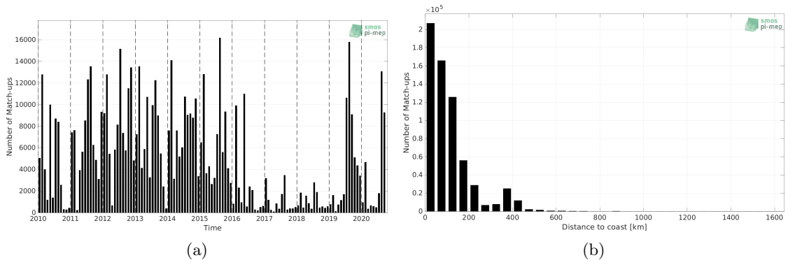
Figure 1: Number of match-ups between ICES and CCI SSS L4 Merged-OI v3.2 - 30-day running (ESA) SSS as a function of time (a) and as function of the distance to coast (b) over the Atlantic Ocean Pi-MEP region and for the full satellite product period.
