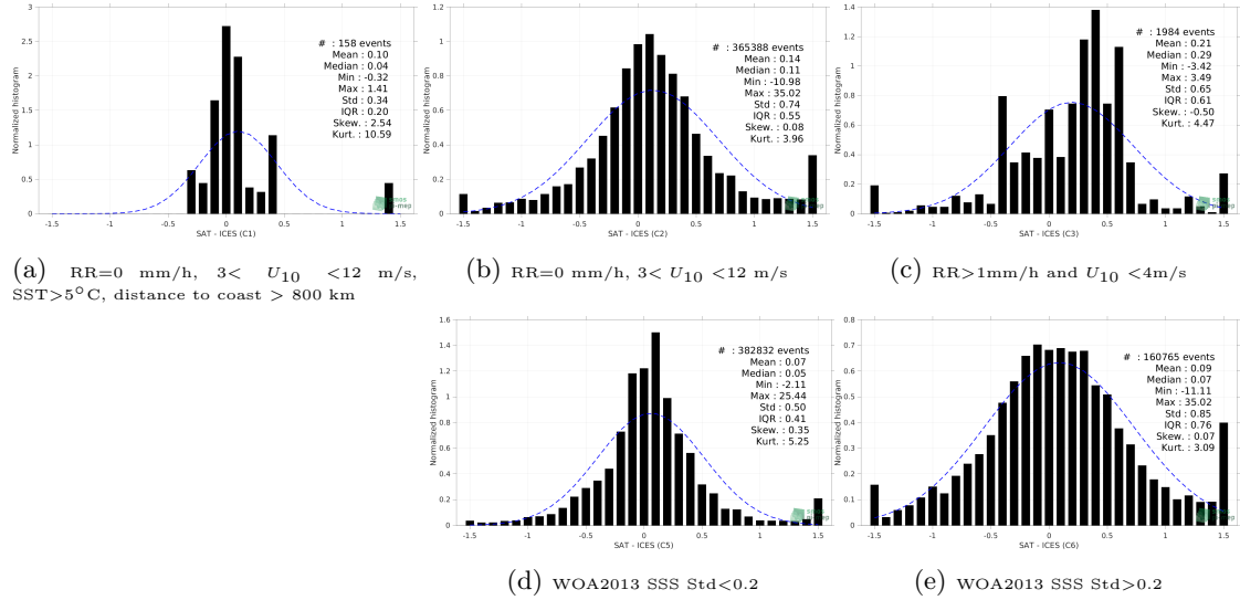
Figure 13: Normalized histogram of \Delta SSS (CCI SSS L4 Merged-OI v3.2 - 30-day running (ESA) - ICES) for 5 different subdatasets corresponding to: RR=0 mm/h, 3 < U_{10} < 12 m/s, SST > 5°C, distance to coast > 800 km (a), RR=0 mm/h, 3 < U_{10} < 12 m/s (b), RR > 1mm/h and U_{10} < 4 m/s (c), WOA2013 SSS Std < 0.2 (d), WOA2013 SSS Std > 0.2 (e).
