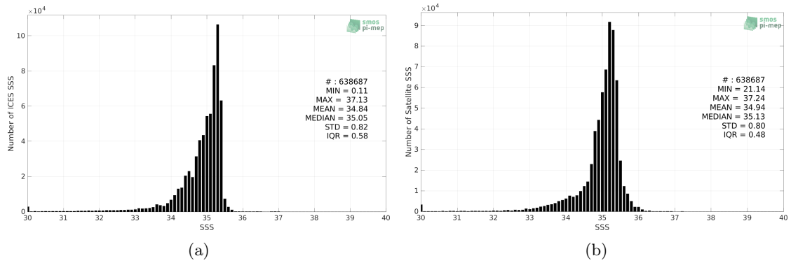
Figure 2: Histograms of SSS from ICES (a) and CCI SSS L4 Merged-OI v3.2 - 30-day running (ESA) (b) considering all match-up pairs per bins of 0.1 over the Atlantic Ocean Pi-MEP region and for the full satellite product period.
