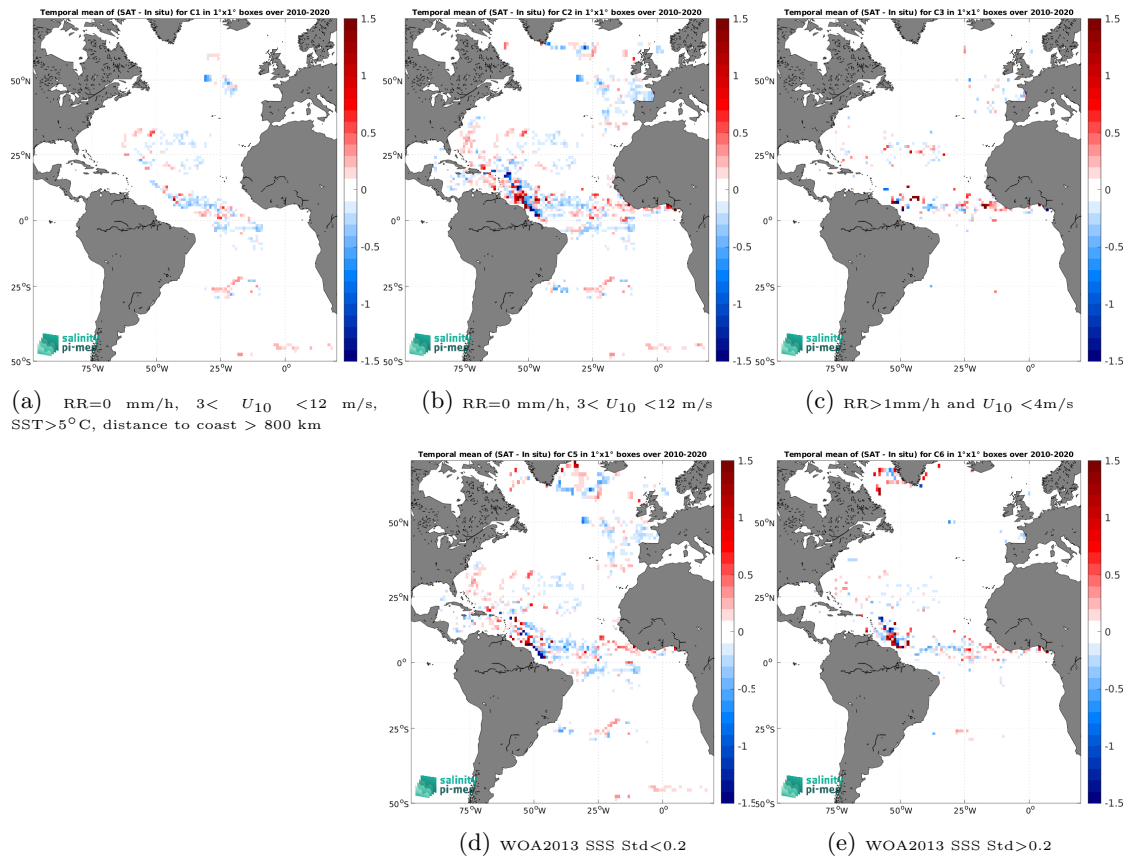
Figure 11: Temporal mean gridded over spatial boxes of size 1^\circ \times 1^\circ of \Delta\text{SSS} (CCI SSS L4 Merged-OI v3.2 - 30-day running (ESA) - Surface drifters) for 5 different subdatasets corresponding to:RR=0 mm/h, 3 < U_{10} < 12 m/s, SST >5^\circ\text{C} , distance to coast > 800 km (a), RR=0 mm/h, 3 < U_{10} < 12 m/s (b), RR >1 mm/h and U_{10} < 4 m/s (c), WOA2013 SSS Std <0.2 (d), WOA2013 SSS Std >0.2 (e).
