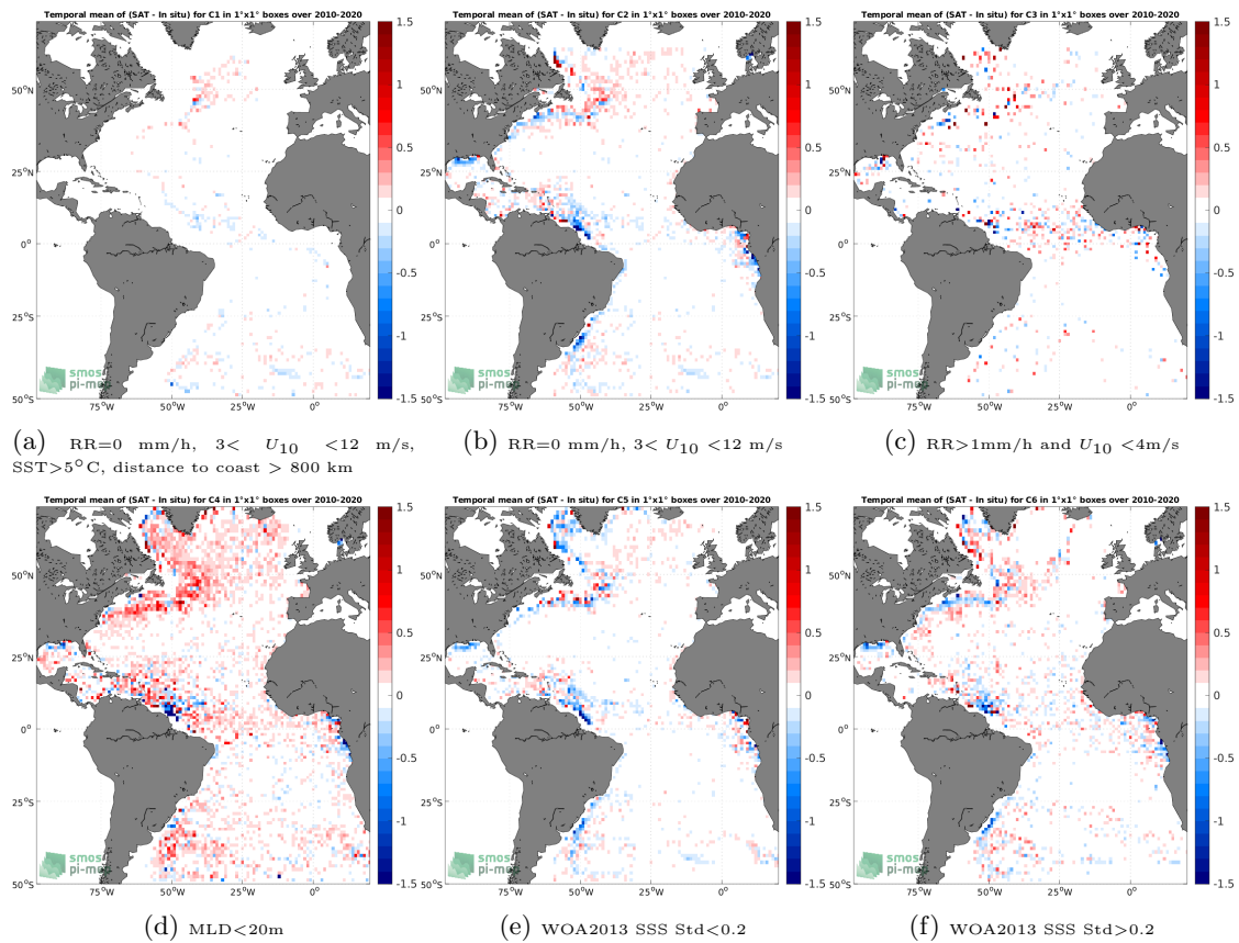
Figure 12: Temporal mean gridded over spatial boxes of size 1^\circ \times 1^\circ of \Delta SSS (CCI SSS L4 Merged-OI v3.2 - 30-day running (ESA) - Argo) for 6 different subdatasets corresponding to:RR=0 mm/h, 3 < U_{10} < 12 m/s, SST >5^\circ C, distance to coast > 800 km (a), RR=0 mm/h, 3 < U_{10} < 12 m/s (b), RR >1 mm/h and U_{10} < 4 m/s (c),MLD <20 m (d),WOA2013 SSS Std <0.2 (e),WOA2013 SSS Std >0.2 (f).
