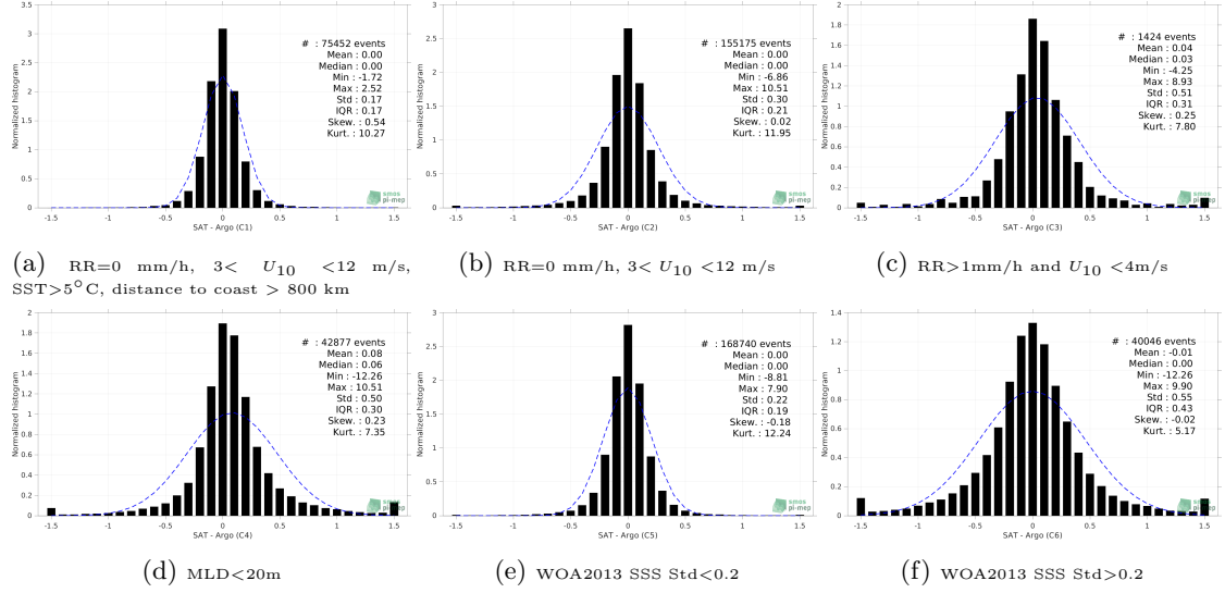
Figure 13: Normalized histogram of \Delta SSS (CCI SSS L4 Merged-OI v3.2 - 30-day running (ESA) - Argo) for 6 different subdatasets corresponding to: RR=0 mm/h, 3 < U_{10} < 12 m/s, SST > 5°C, distance to coast > 800 km (a), RR=0 mm/h, 3 < U_{10} < 12 m/s (b), RR > 1mm/h and U_{10} < 4 m/s (c), MLD < 20m (d), WOA2013 SSS Std < 0.2 (e), WOA2013 SSS Std > 0.2 (f).
