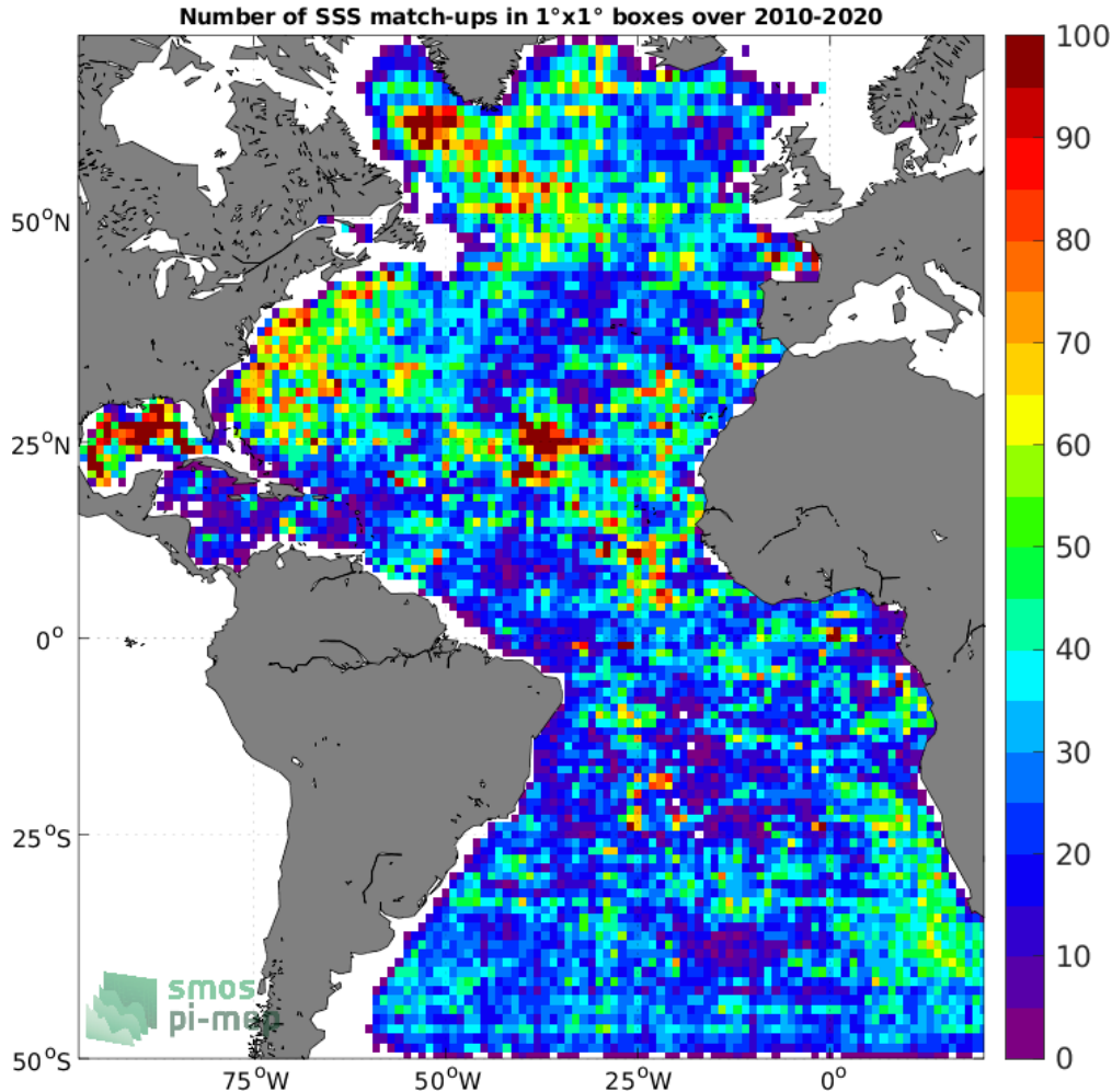
Figure 4: Number of SSS match-ups between Argo SSS and the CCI SSS L4 Merged-OI v3.2 - 30-day running (ESA) SSS product for the Atlantic Ocean Pi-MEP region over 1^\circ \times 1^\circ boxes and for the full satellite product period.
