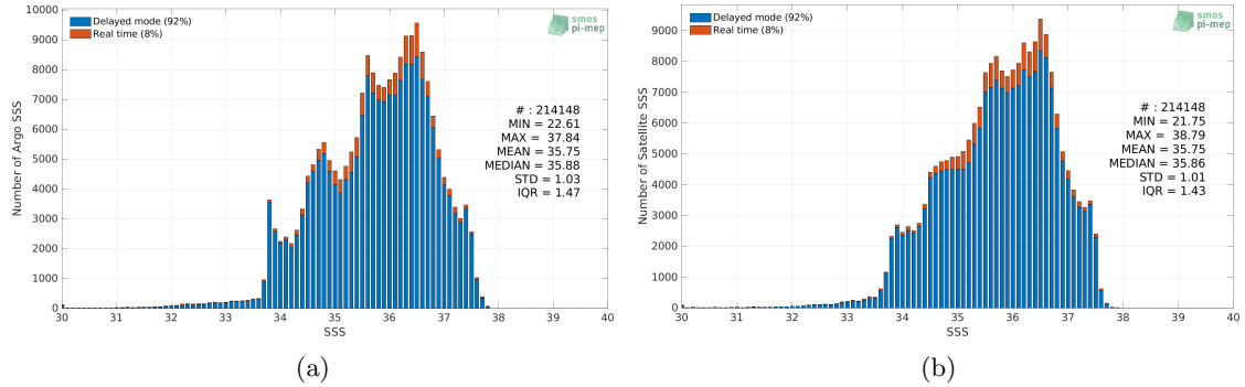
Figure 2: Histograms of SSS from Argo (a) and CCI SSS L4 Merged-OI v3.2 - 30-day running (ESA) (b) considering all match-up pairs per bins of 0.1 over the Atlantic Ocean Pi-MEP region and for the full satellite product period.
