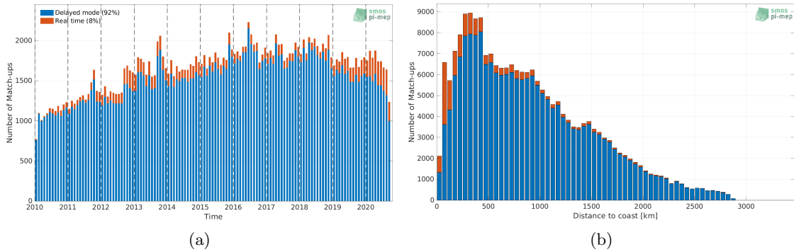
Figure 1: Number of match-ups between Argo and CCI SSS L4 Merged-OI v3.2 - 30-day running (ESA) SSS as a function of time (a) and as function of the distance to coast (b) over the Atlantic Ocean Pi-MEP region and for the full satellite product period.
