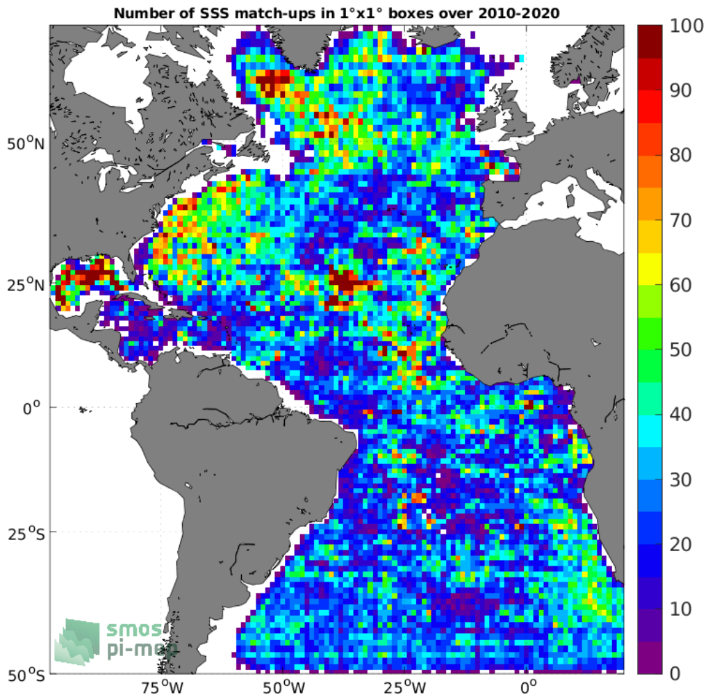
Figure 4: Number of SSS match-ups between Argo SSS and the CCI SSS L4 Merged-OI v3.2 - 30-day running (ESA) SSS product for the Atlantic Ocean Pi-MEP region over 1°x1° boxes and for the full satellite product period.
