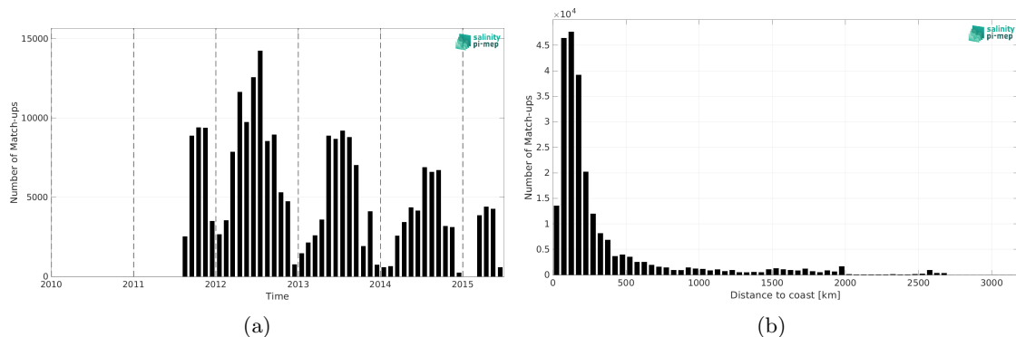
Figure 2: Number of match-ups between TSG (SAMOS) and Aquarius SSS L4 OI v5 - Weekly (IPRC) SSS as a function of time (a) and as function of the distance to coast (b) over the Atlantic Ocean Pi-MEP region and for the full satellite product period.
