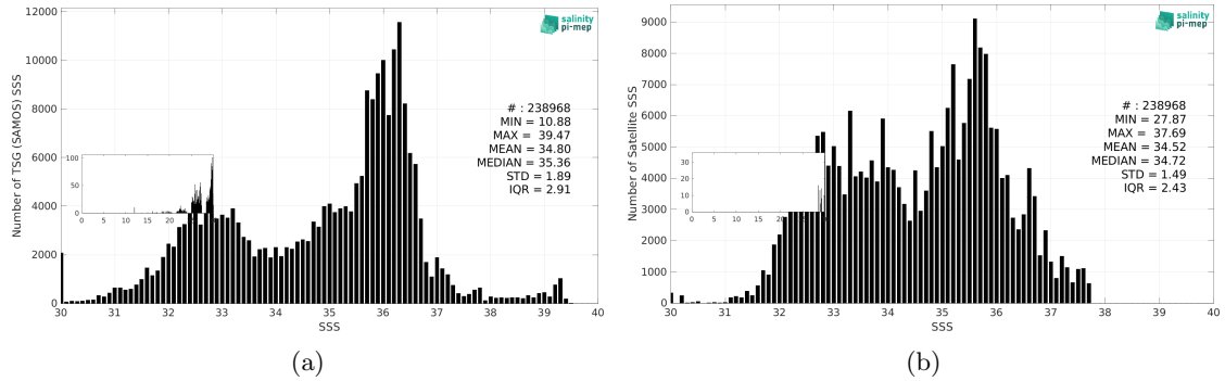
Figure 3: Histograms of SSS from TSG (SAMOS) (a) and Aquarius SSS L4 OI v5 - Weekly (IPRC) (b) considering all match-up pairs per bins of 0.1 over the Atlantic Ocean Pi-MEP region and for the full satellite product period.
