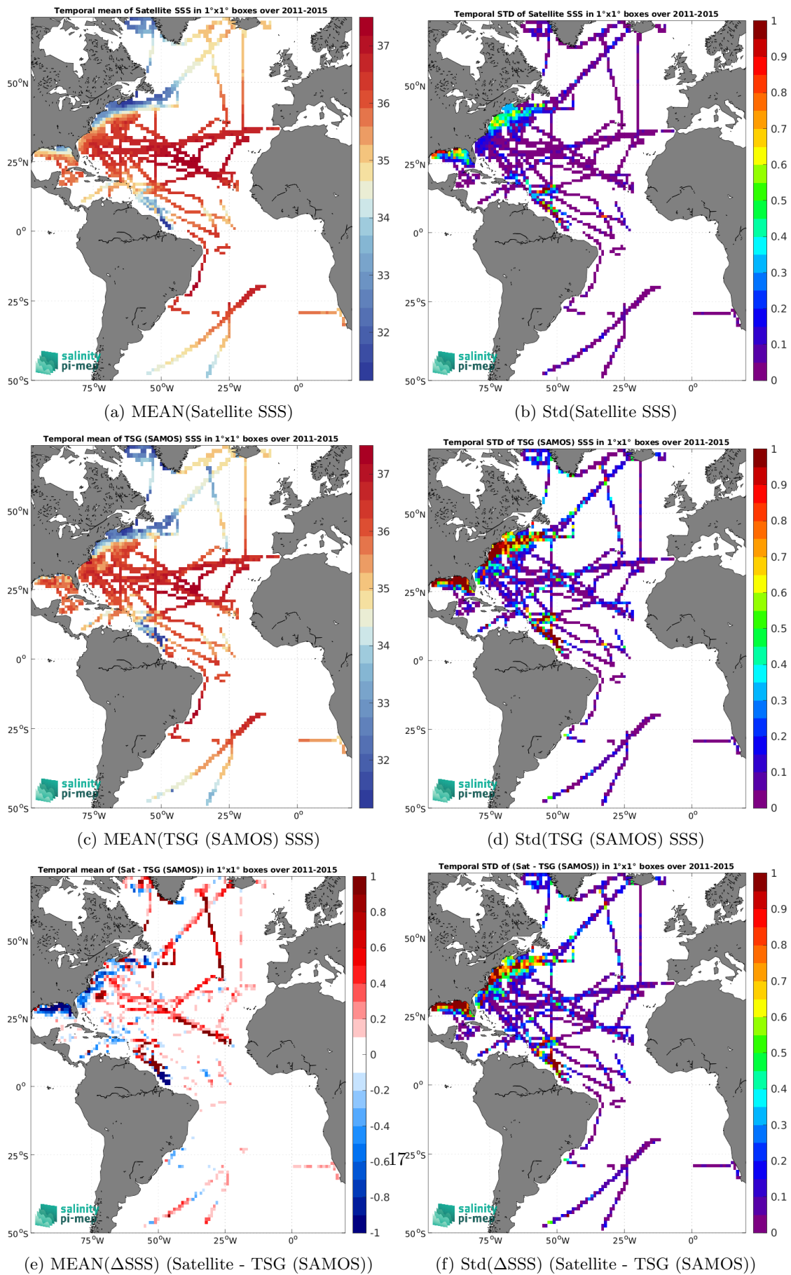
Figure 7: Temporal mean (left) and Std (right) of SSS from Aquarius SSS L4 OI v5 - Weekly (IPRC) (top), TSG (SAMOS) (middle), and of \Delta SSS (Satellite - TSG (SAMOS)). Only match-up pairs are used to generate these maps.
