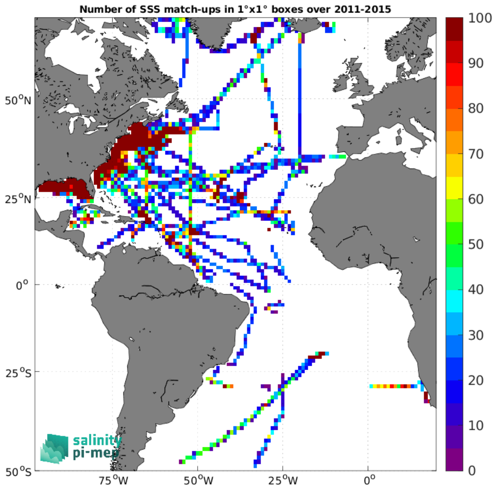
Figure 5: Number of SSS match-ups between TSG (SAMOS) SSS and the Aquarius SSS L4 OI v5 - Weekly (IPRC) SSS product for the Atlantic Ocean Pi-MEP region over 1^\circ \times 1^\circ boxes and for the full satellite product period.
