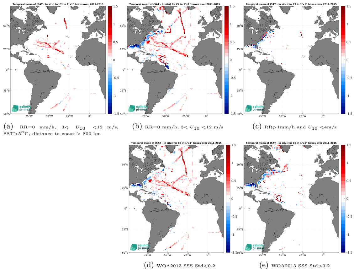
Figure 14: Temporal mean gridded over spatial boxes of size 1^\circ \times 1^\circ of \Delta SSS (Aquarius SSS L4 OI v5 - Weekly (IPRC) - TSG (SAMOS)) for 5 different subdatasets corresponding to:RR=0 mm/h, 3 < U_{10} < 12 m/s, SST >5^\circ\text{C} , distance to coast > 800 km (a), RR=0 mm/h, 3 < U_{10} < 12 m/s (b), RR >1 mm/h and U_{10} < 4 m/s (c), WOA2013 SSS Std <0.2 (d), WOA2013 SSS Std >0.2 (e).
