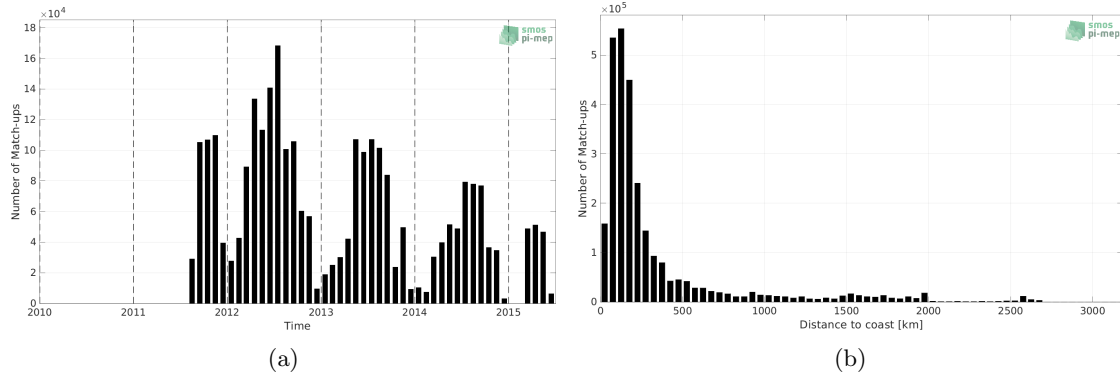
Figure 1: Number of match-ups between TSG (SAMOS) and Aquarius SSS L4 OI v5 - Weekly (IPRC) SSS as a function of time (a) and as function of the distance to coast (b) over the Atlantic Ocean Pi-MEP region and for the full satellite product period.
