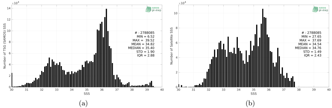
Figure 2: Histograms of SSS from TSG (SAMOS) (a) and Aquarius SSS L4 OI v5 - Weekly (IPRC) (b) considering all match-up pairs per bins of 0.1 over the Atlantic Ocean Pi-MEP region and for the full satellite product period.
