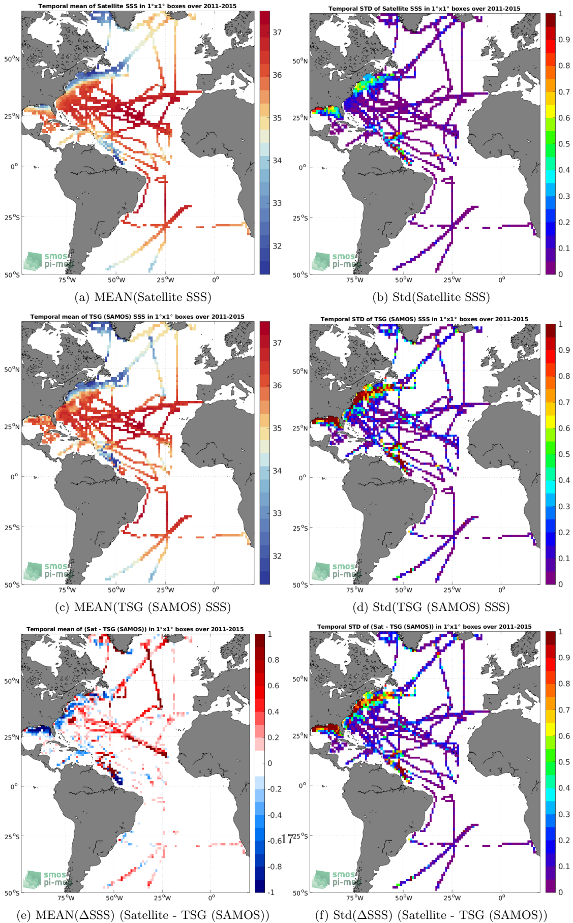
Figure 6: Temporal mean (left) and Std (right) of SSS from Aquarius SSS L4 OI v5 - Weekly (IPRC) (top), TSG (SAMOS) (middle), and of \Delta SSS (Satellite - TSG (SAMOS)). Only match-up pairs are used to generate these maps.
