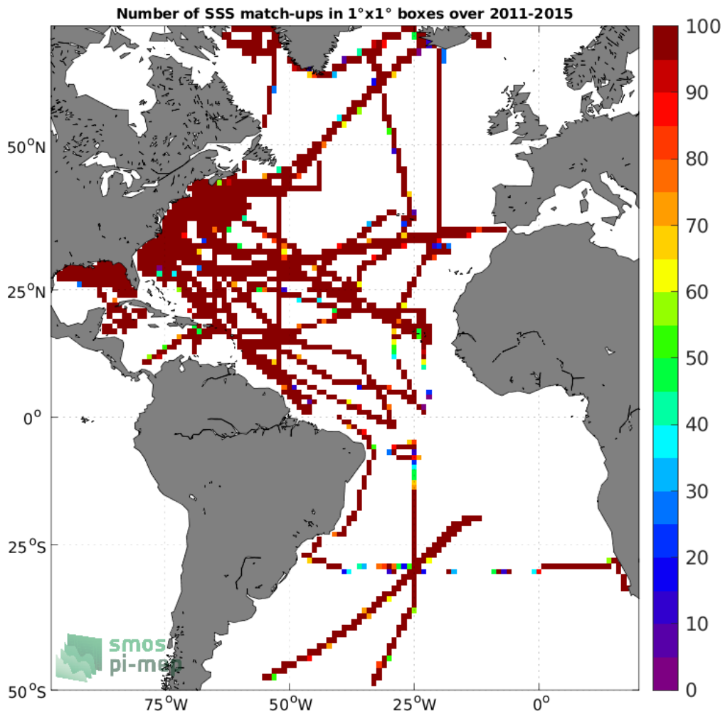
Figure 4: Number of SSS match-ups between TSG (SAMOS) SSS and the Aquarius SSS L4 OI v5 - Weekly (IPRC) SSS product for the Atlantic Ocean Pi-MEP region over 1°x1° boxes and for the full satellite product period.
