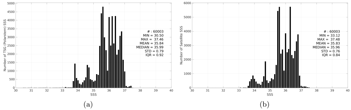
Figure 3: Histograms of SSS from TSG (Polarstern) (a) and Aquarius SSS L4 OI v5 - Weekly (IPRC) (b) considering all match-up pairs per bins of 0.1 over the Atlantic Ocean Pi-MEP region and for the full satellite product period.
