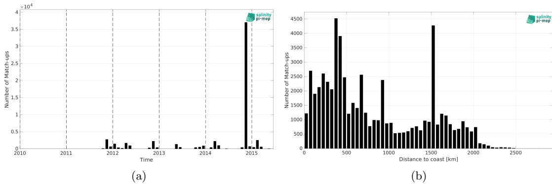
Figure 2: Number of match-ups between TSG (Polarstern) and Aquarius SSS L4 OI v5 - Weekly (IPRC) SSS as a function of time (a) and as function of the distance to coast (b) over the Atlantic Ocean Pi-MEP region and for the full satellite product period.
