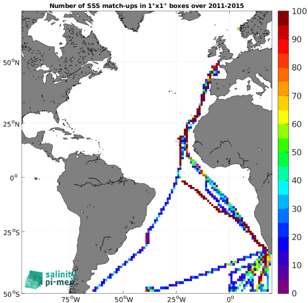
Figure 5: Number of SSS match-ups between TSG (Polarstern) SSS and the Aquarius SSS L4 OI v5 - Weekly (IPRC) SSS product for the Atlantic Ocean Pi-MEP region over 1^\circ \times 1^\circ boxes and for the full satellite product period.
