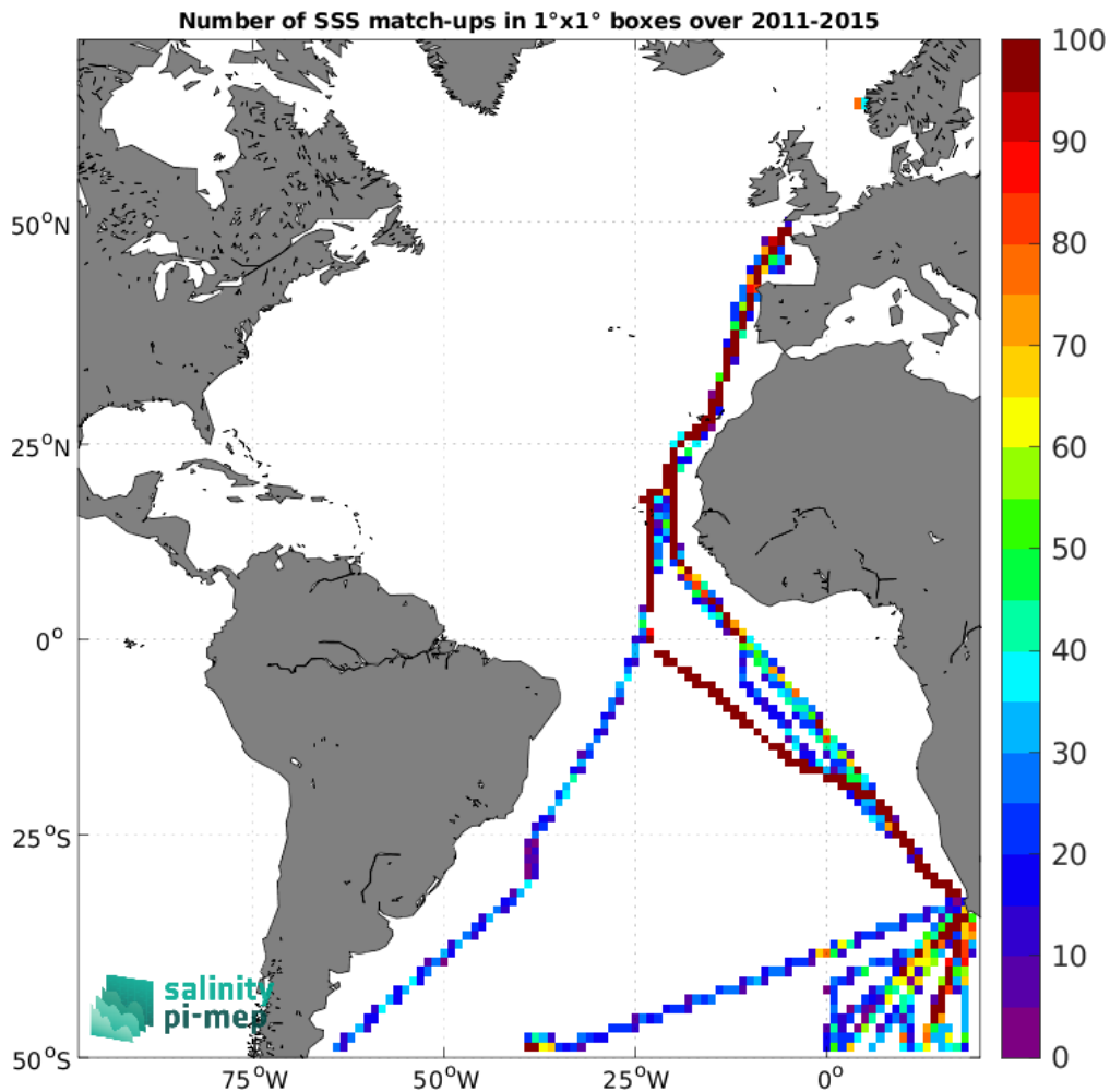
Figure 4: Number of SSS match-ups between TSG (Polarstern) SSS and the Aquarius SSS L4 OI v5 - Weekly (IPRC) SSS product for the Atlantic Ocean Pi-MEP region over 1^{\circ} \times 1^{\circ} boxes and for the full satellite product period.
