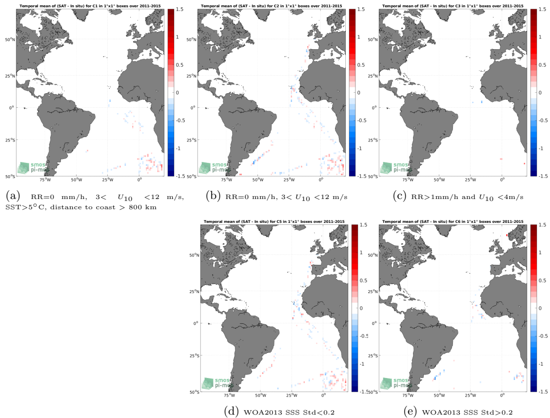
Figure 12: Temporal mean gridded over spatial boxes of size 1^\circ \times 1^\circ of \Delta SSS (Aquarius SSS L4 OI v5 - Weekly (IPRC) - TSG (Polarstern)) for 5 different subdatasets corresponding to:RR=0 mm/h, 3 < U_{10} < 12 m/s, SST >5^\circ\text{C} , distance to coast > 800 km (a), RR=0 mm/h, 3 < U_{10} < 12 m/s (b), RR >1 mm/h and U_{10} < 4 m/s (c), WOA2013 SSS Std <0.2 (d), WOA2013 SSS Std >0.2 (e).
