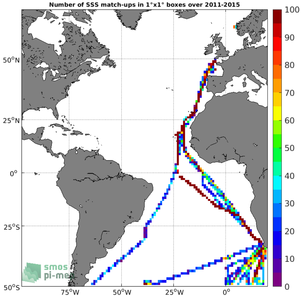
Figure 4: Number of SSS match-ups between TSG (Polarstern) SSS and the Aquarius SSS L4 OI v5 - Weekly (IPRC) SSS product for the Atlantic Ocean Pi-MEP region over 1^\circ \times 1^\circ boxes and for the full satellite product period.
