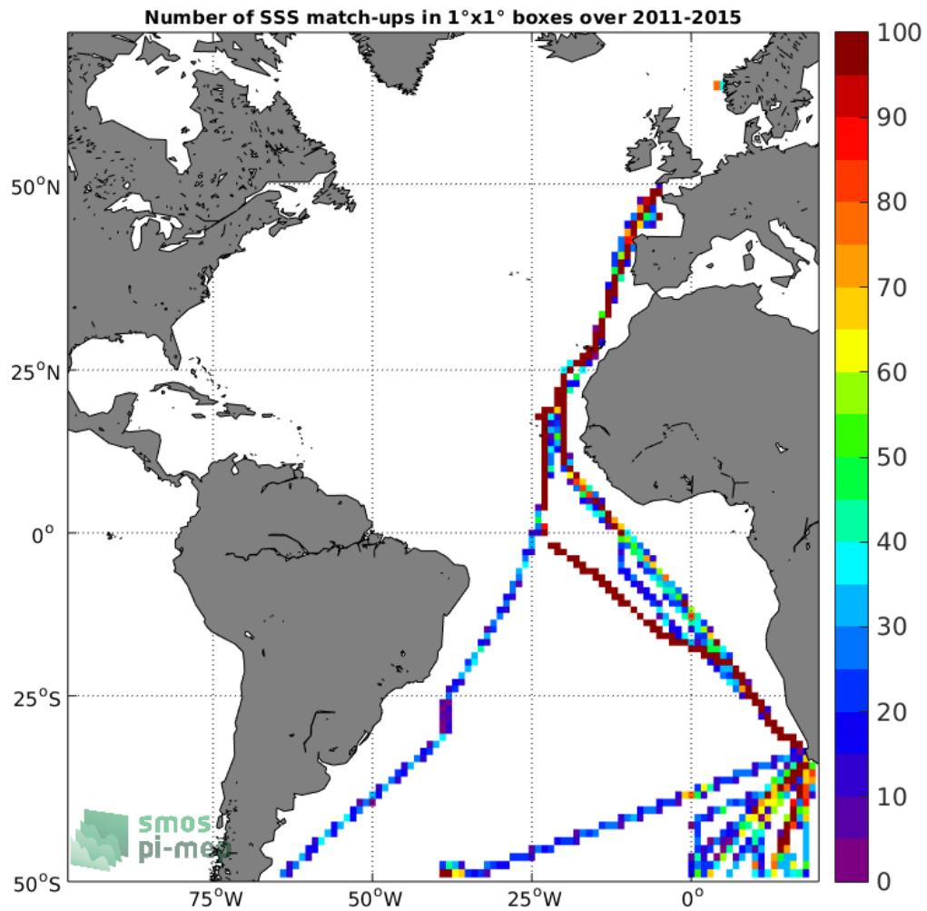
Figure 4: Number of SSS match-ups between TSG-POLARSTERN SSS and the Aquarius-L4-IPRC-V5-WEEKLY SSS product for the Atlantic Ocean Pi-MEP region over 1°x1° boxes and for the full satellite product period.
