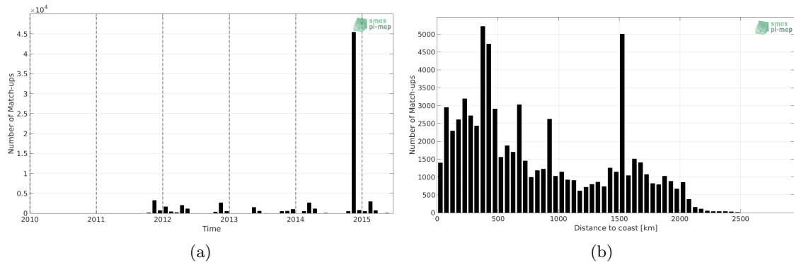
Figure 1: Number of match-ups between TSG-POLARSTERN and Aquarius-L4-IPRC-V5-WEEKLY SSS as a function of time (a) and as function of the distance to coast (b) over the Atlantic Ocean Pi-MEP region and for the full satellite product period.
