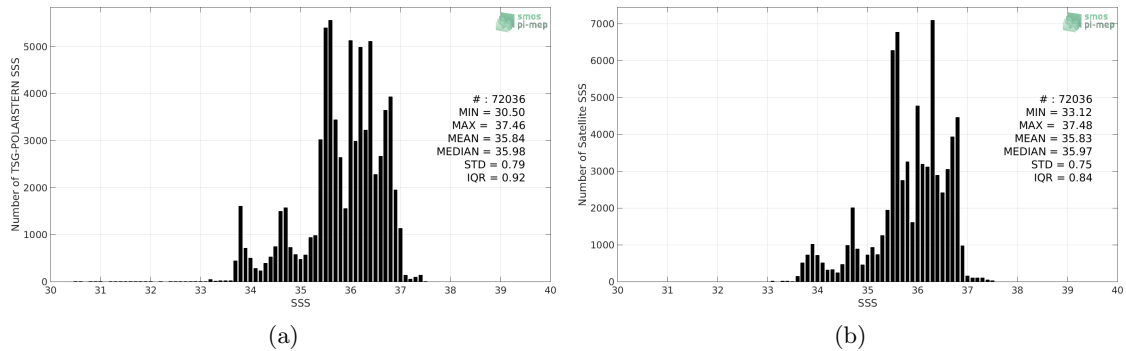
Figure 2: Histograms of SSS from TSG-POLARSTERN (a) and Aquarius-L4-IPRC-V5-WEEKLY (b) considering all match-up pairs per bins of 0.1 over the Atlantic Ocean Pi-MEP region and for the full satellite product period.
