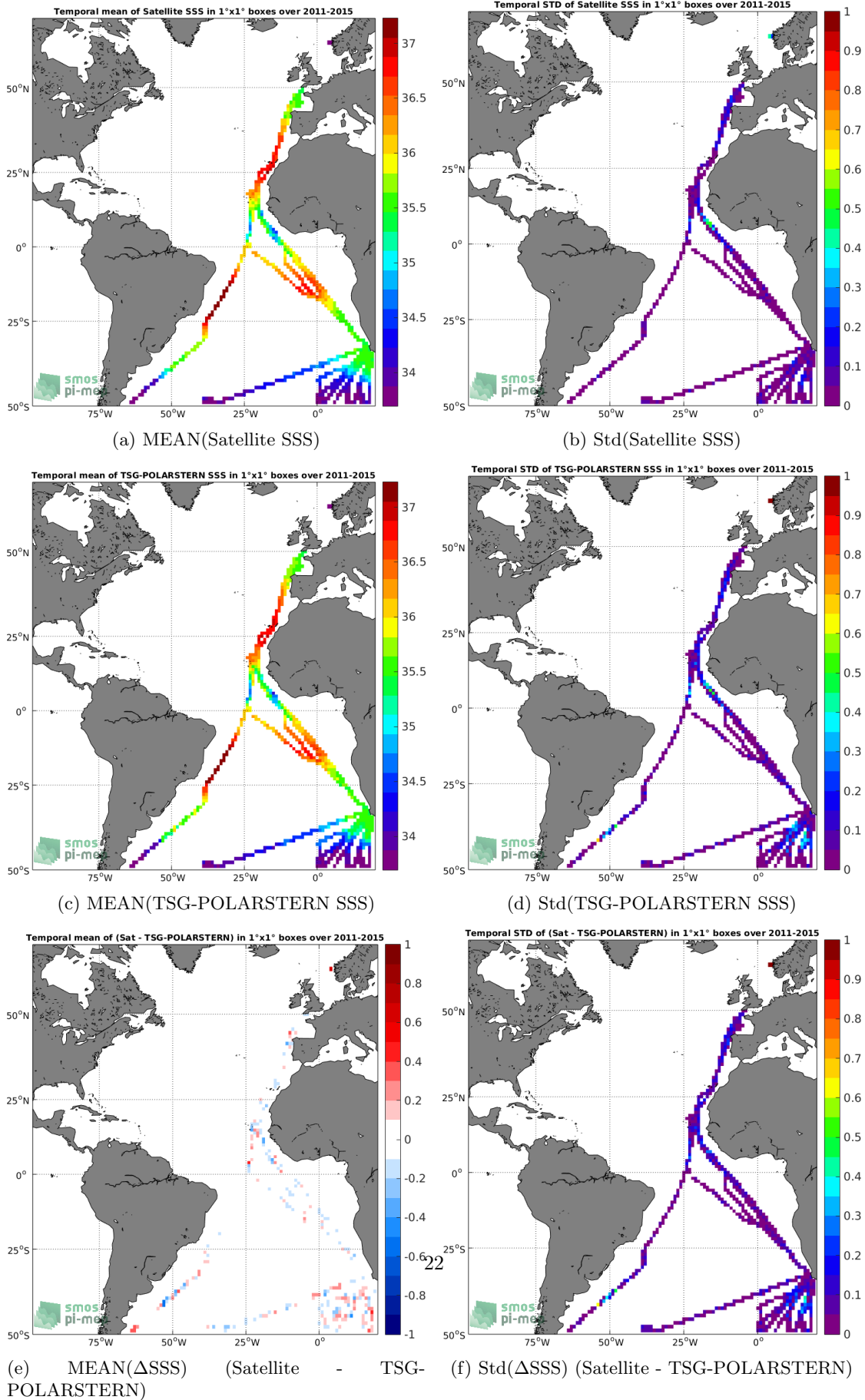
Figure 6: Temporal mean (left) and Std (right) of SSS from Aquarius-L4-IPRC-V5-WEEKLY (top), TSG-POLARSTERN (middle), and of \Delta SSS (Satellite - TSG-POLARSTERN). Only match-up pairs are used to generate these maps.
