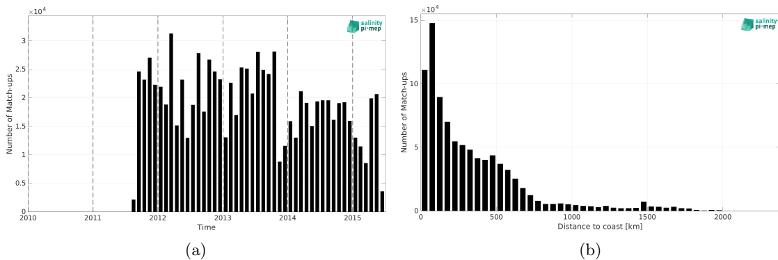
Figure 2: Number of match-ups between TSG (LEGOS-DM) and Aquarius SSS L4 OI v5 - Weekly (IPRC) SSS as a function of time (a) and as function of the distance to coast (b) over the Atlantic Ocean Pi-MEP region and for the full satellite product period.
