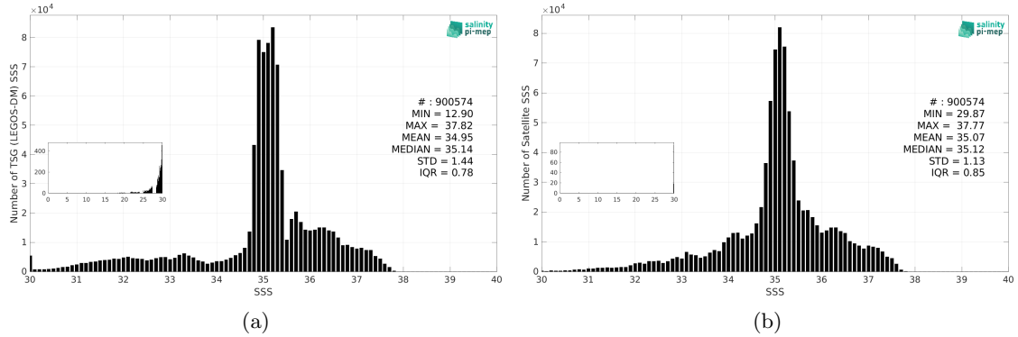
Figure 3: Histograms of SSS from TSG (LEGOS-DM) (a) and Aquarius SSS L4 OI v5 - Weekly (IPRC) (b) considering all match-up pairs per bins of 0.1 over the Atlantic Ocean Pi-MEP region and for the full satellite product period.
