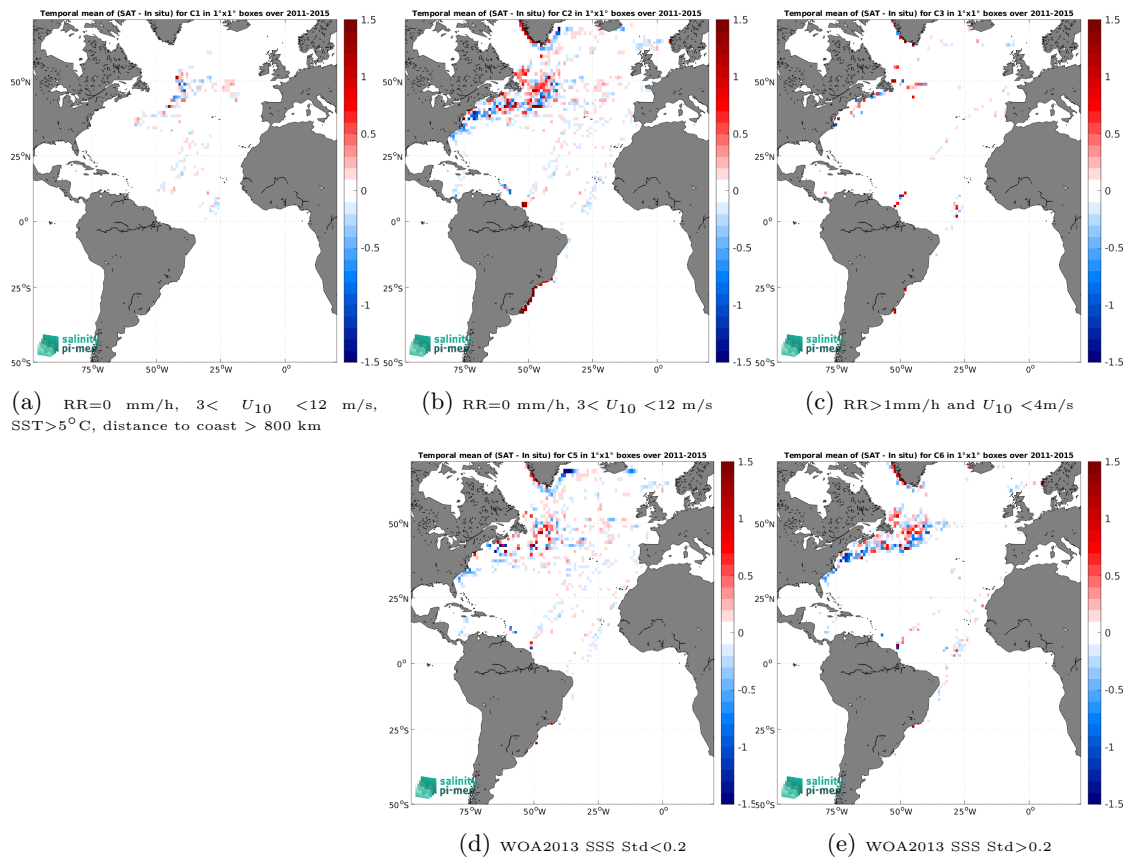
Figure 14: Temporal mean gridded over spatial boxes of size 1^\circ \times 1^\circ of \Delta\text{SSS} (Aquarius SSS L4 OI v5 - Weekly (IPRC) - TSG (LEGOS-DM)) for 5 different subdatasets corresponding to:RR=0 mm/h, 3 < U_{10} < 12 m/s, SST>5°C, distance to coast > 800 km (a), RR=0 mm/h, 3 < U_{10} < 12 m/s (b), RR>1mm/h and U_{10} < 4 m/s (c), WOA2013 SSS Std<0.2 (d), WOA2013 SSS Std>0.2 (e).
