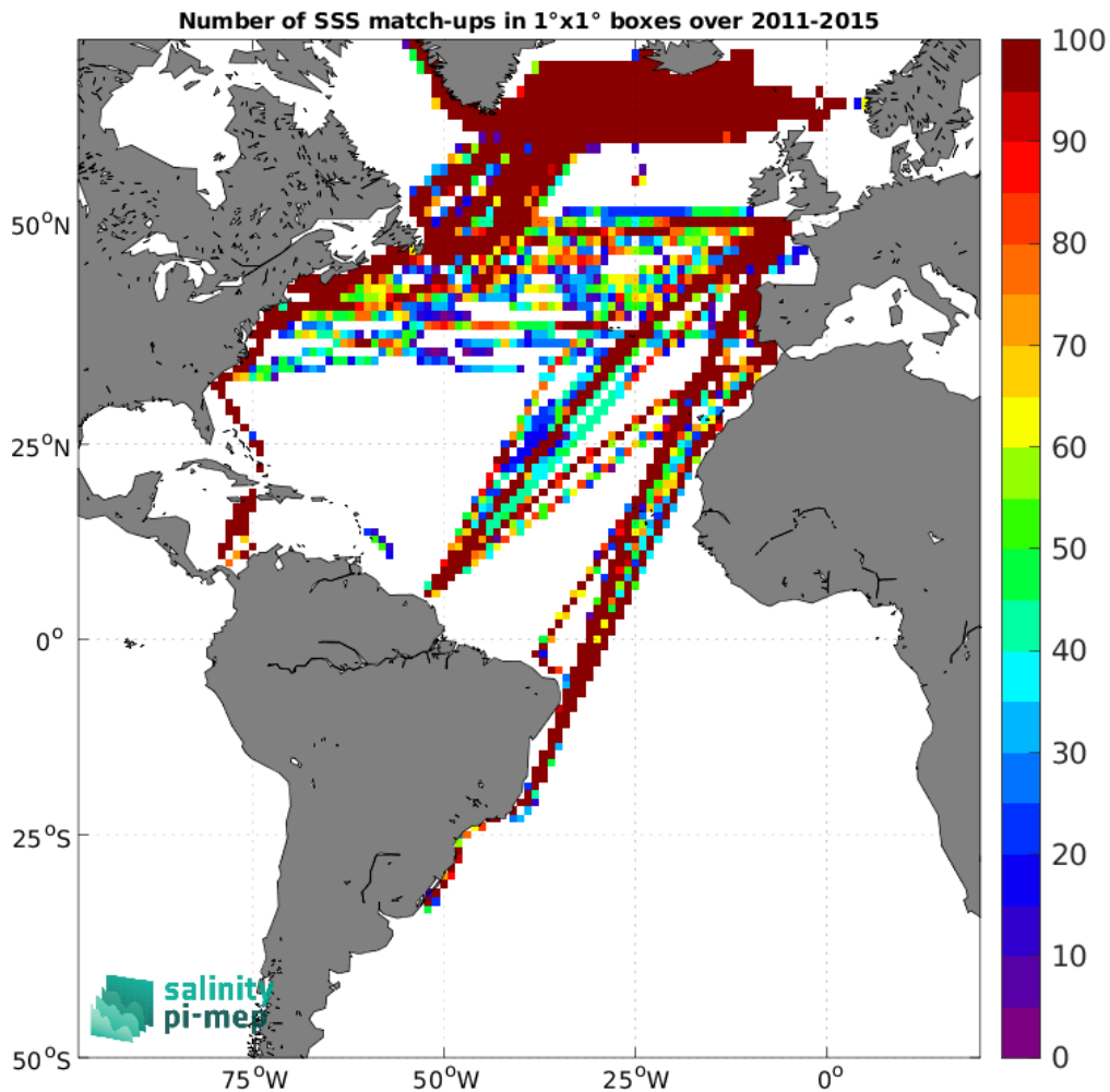
Figure 5: Number of SSS match-ups between TSG (LEGOS-DM) SSS and the Aquarius SSS L4 OI v5 - Weekly (IPRC) SSS product for the Atlantic Ocean Pi-MEP region over 1^\circ \times 1^\circ boxes and for the full satellite product period.
