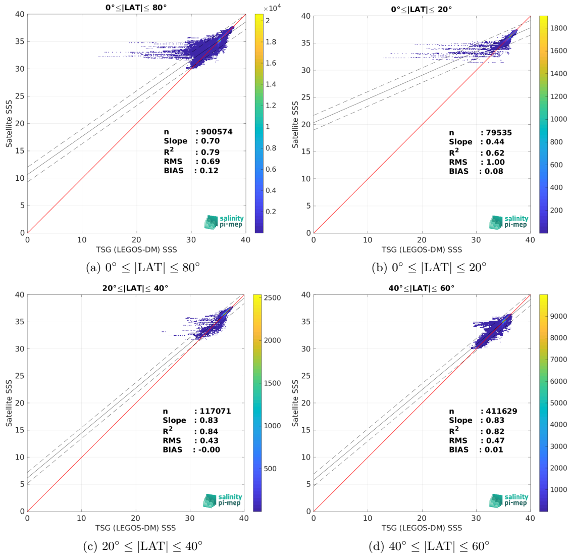
Figure 10: Contour maps of the concentration of Aquarius SSS L4 OI v5 - Weekly (IPRC) SSS (y-axis) versus TSG (LEGOS-DM) SSS (x-axis) at match-up pairs for different latitude bands. For each plot, the red line shows x=y . The black thin and dashed lines indicate a linear fit through the data cloud and the \pm 95\% confidence levels, respectively. The number match-up pairs n , the slope and R^2 coefficient of the linear fit, the root mean square (RMS) and the mean bias between satellite and in situ data are indicated for each latitude band in each plots.
