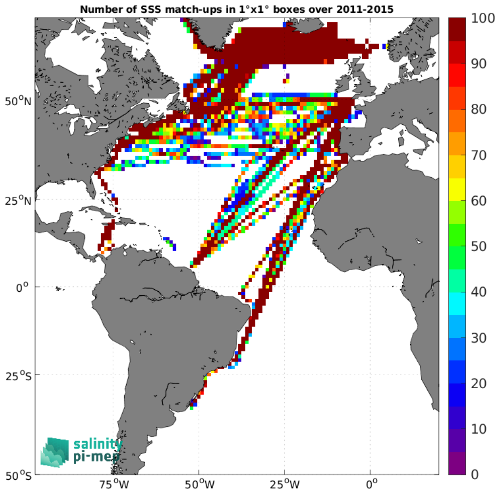
Figure 5: Number of SSS match-ups between TSG (LEGOS-DM) SSS and the Aquarius SSS L4 OI v5 - Weekly (IPRC) SSS product for the Atlantic Ocean Pi-MEP region over 1^{\circ} \times 1^{\circ} boxes and for the full satellite product period.
