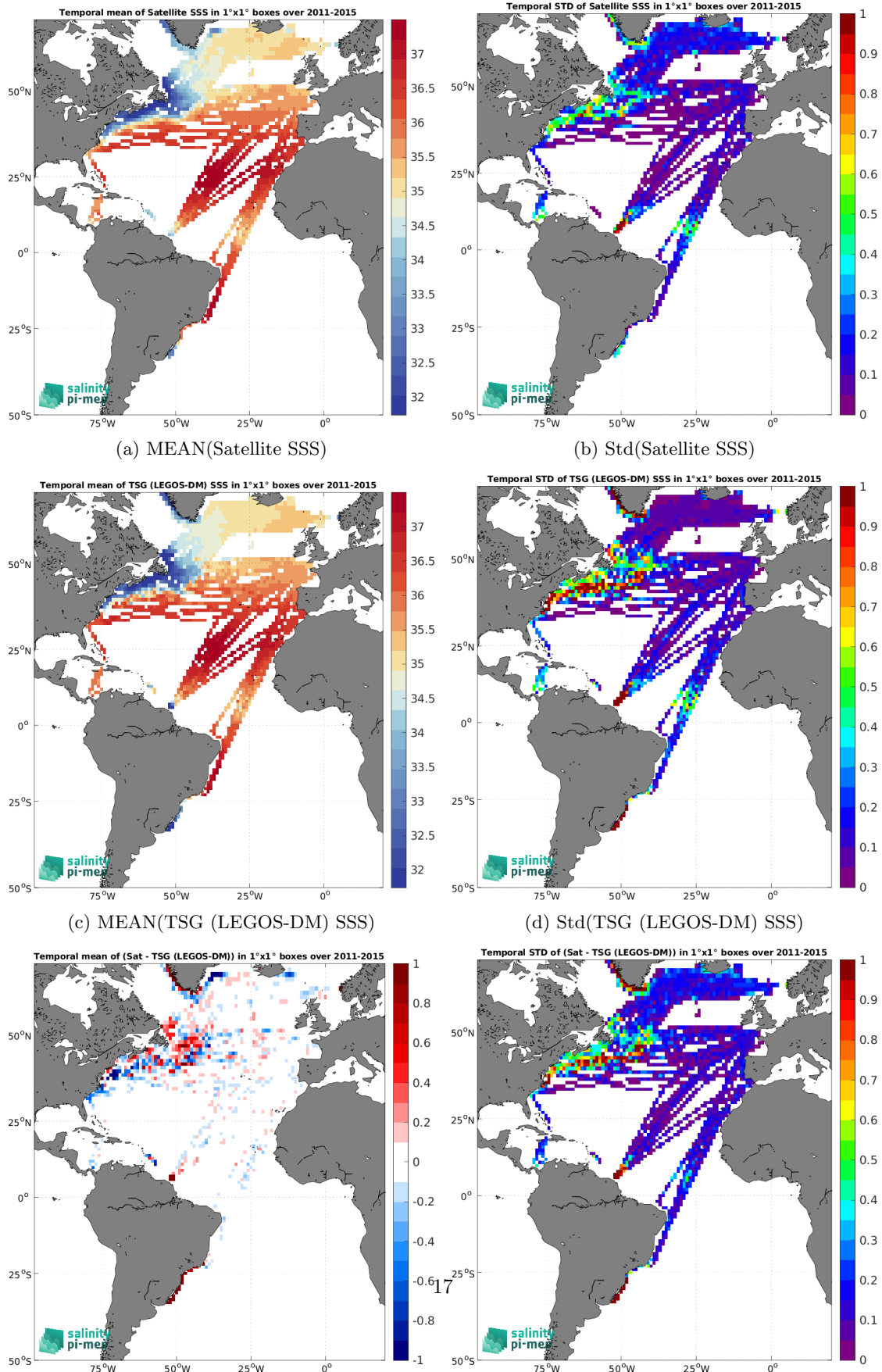
(e) MEAN( \Delta\text{SSS} ) (Satellite - TSG (LEGOS-DM)) (f) Std( \Delta\text{SSS} ) (Satellite - TSG (LEGOS-DM)) Figure 7: Temporal mean (left) and Std (right) of SSS from Aquarius SSS L4 OI v5 - Weekly (IPRC) (top), TSG (LEGOS-DM) (middle), and of \Delta\text{SSS} (Satellite - TSG (LEGOS-DM)). Only match-up pairs are used to generate these maps.
