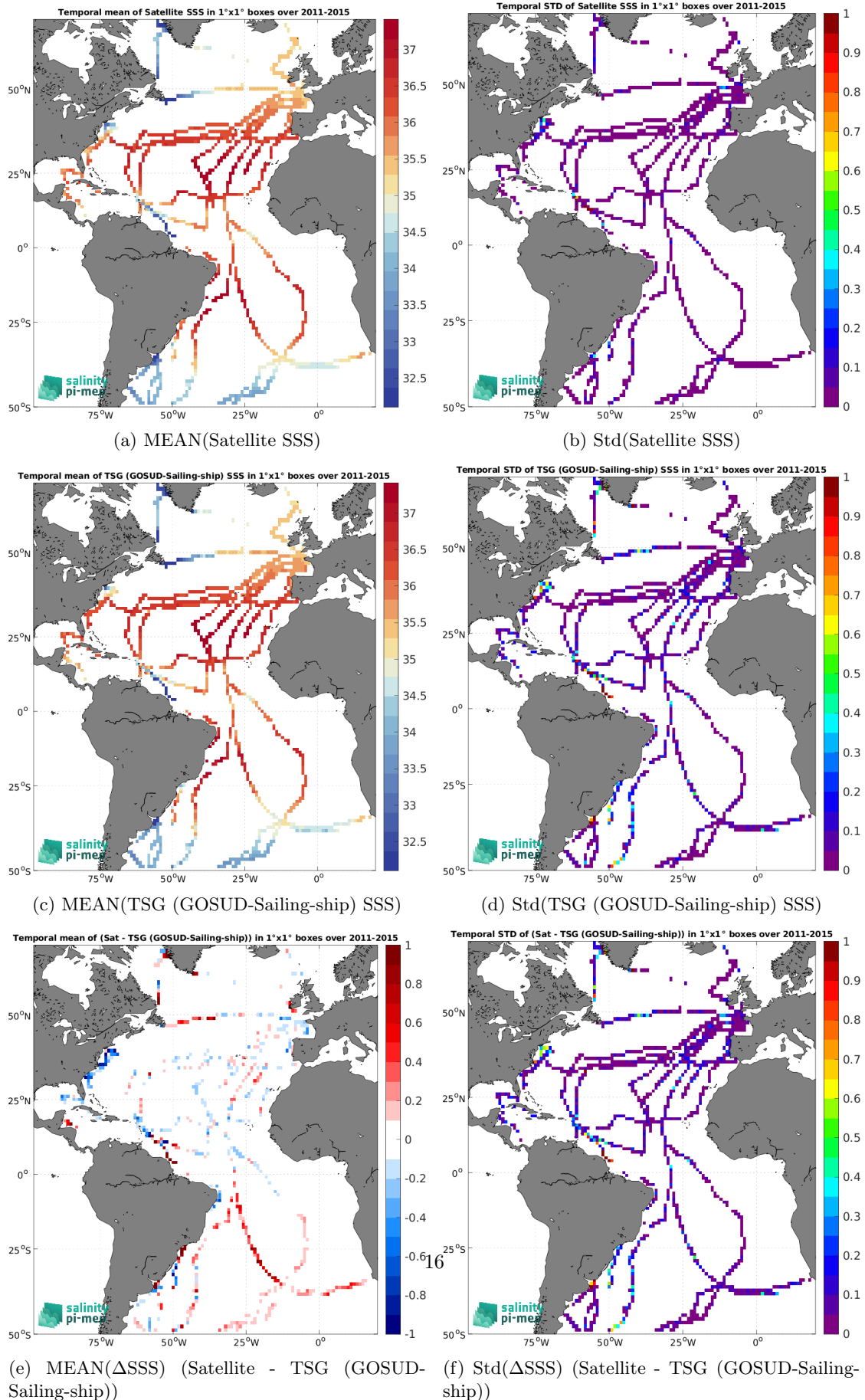
Figure 7: Temporal mean (left) and Std (right) of SSS from Aquarius SSS L4 OI v5 - Weekly (IPRC) (top), TSG (GOSUD-Sailing-ship) (middle), and of \Delta SSS (Satellite - TSG (GOSUD-Sailing-ship)). Only match-up pairs are used to generate these maps.
