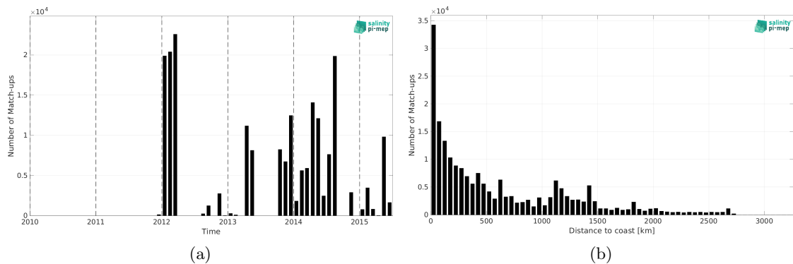
Figure 2: Number of match-ups between TSG (GOSUD-Sailing-ship) and Aquarius SSS L4 OI v5 - Weekly (IPRC) SSS as a function of time (a) and as function of the distance to coast (b) over the Atlantic Ocean Pi-MEP region and for the full satellite product period.
