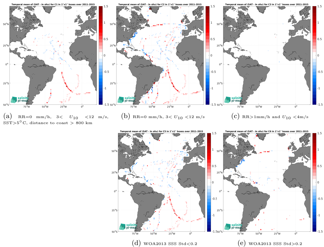
Figure 14: Temporal mean gridded over spatial boxes of size 1^\circ \times 1^\circ of \Delta\text{SSS} (Aquarius SSS L4 OI v5 - Weekly (IPRC) - TSG (GOSUD-Sailing-ship)) for 5 different subdatasets corresponding to:RR=0 mm/h, 3 < U_{10} < 12 m/s, SST>5°C, distance to coast > 800 km (a), RR=0 mm/h, 3 < U_{10} < 12 m/s (b), RR>1mm/h and U_{10} < 4 m/s (c), WOA2013 SSS Std<0.2 (d), WOA2013 SSS Std>0.2 (e).
