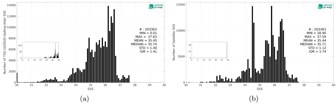
Figure 3: Histograms of SSS from TSG (GOSUD-Sailing-ship) (a) and Aquarius SSS L4 OI v5 - Weekly (IPRC) (b) considering all match-up pairs per bins of 0.1 over the Atlantic Ocean Pi-MEP region and for the full satellite product period.
