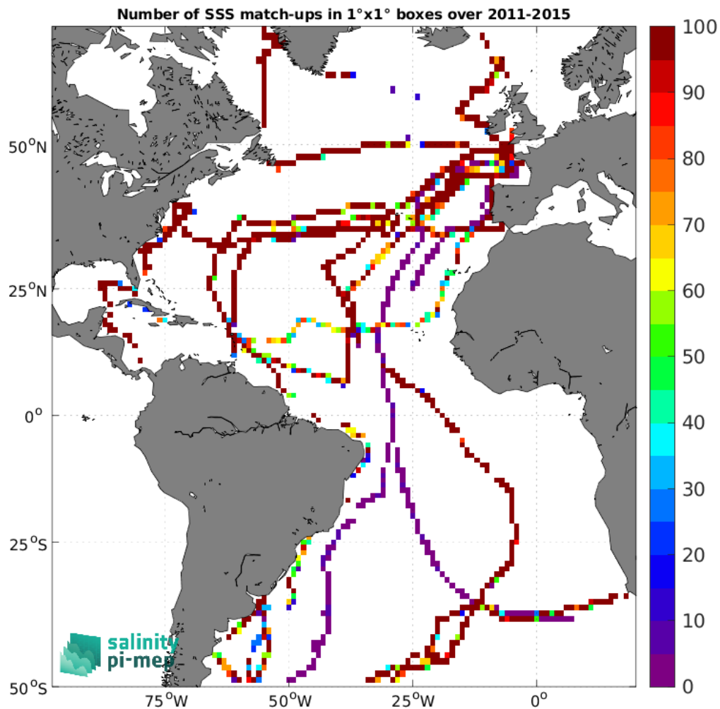
Figure 5: Number of SSS match-ups between TSG (GOSUD-Sailing-ship) SSS and the Aquarius SSS L4 OI v5 - Weekly (IPRC) SSS product for the Atlantic Ocean Pi-MEP region over 1°x1° boxes and for the full satellite product period.
