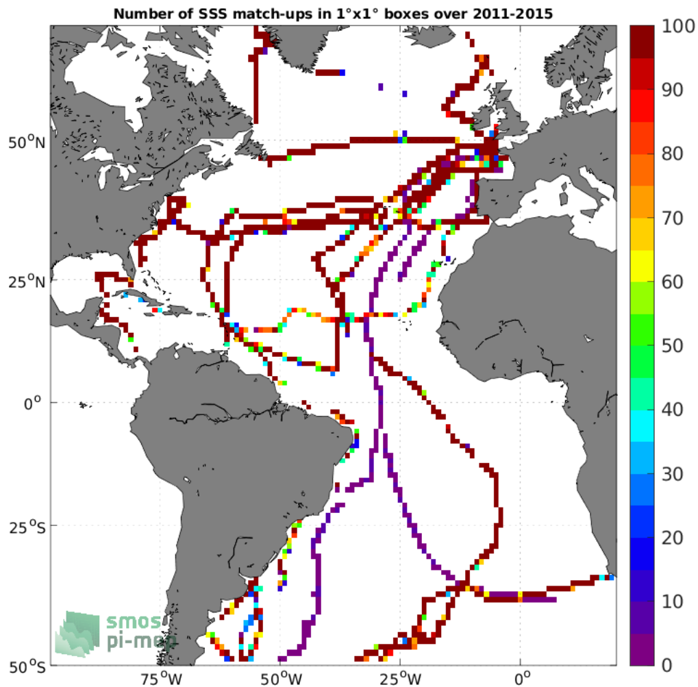
Figure 4: Number of SSS match-ups between TSG (GOSUD-Sailing-ship) SSS and the Aquarius SSS L4 OI v5 - Weekly (IPRC) SSS product for the Atlantic Ocean Pi-MEP region over 1°x1° boxes and for the full satellite product period.
