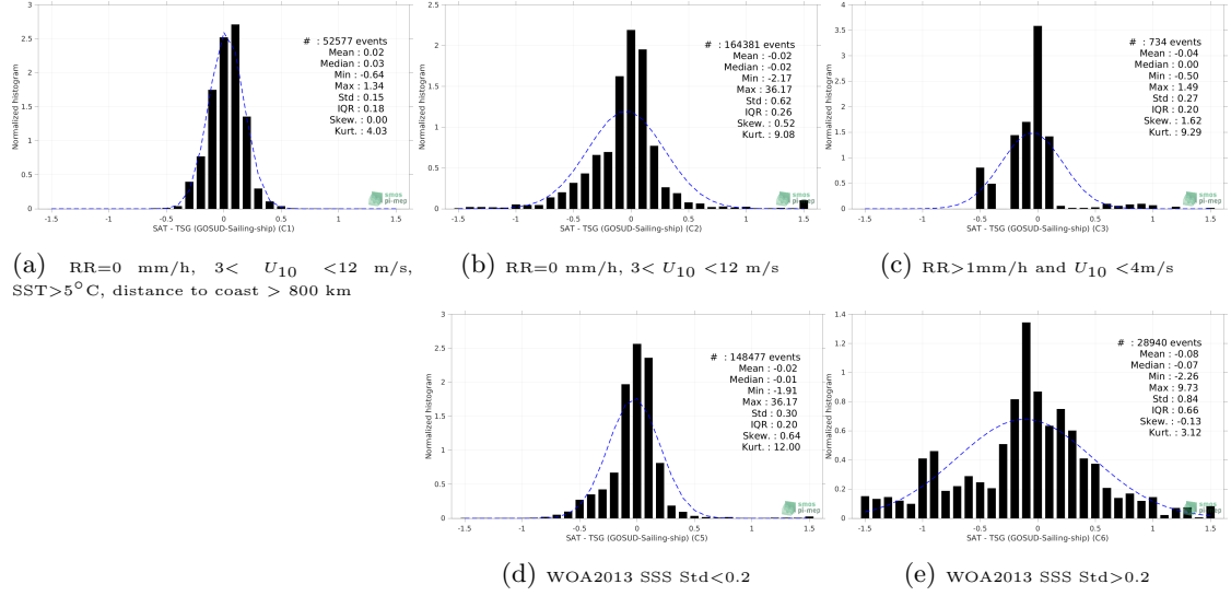
Figure 13: Normalized histogram of \Delta\text{SSS} (Aquarius SSS L4 OI v5 - Weekly (IPRC) - TSG (GOSUD-Sailing-ship)) for 5 different subdatasets corresponding to: RR=0 mm/h, 3 < U_{10} < 12 m/s, SST>5°C, distance to coast > 800 km (a), RR=0 mm/h, 3 < U_{10} < 12 m/s (b), RR>1mm/h and U_{10} < 4 m/s (c), WOA2013 SSS Std<0.2 (d), WOA2013 SSS Std>0.2 (e).
