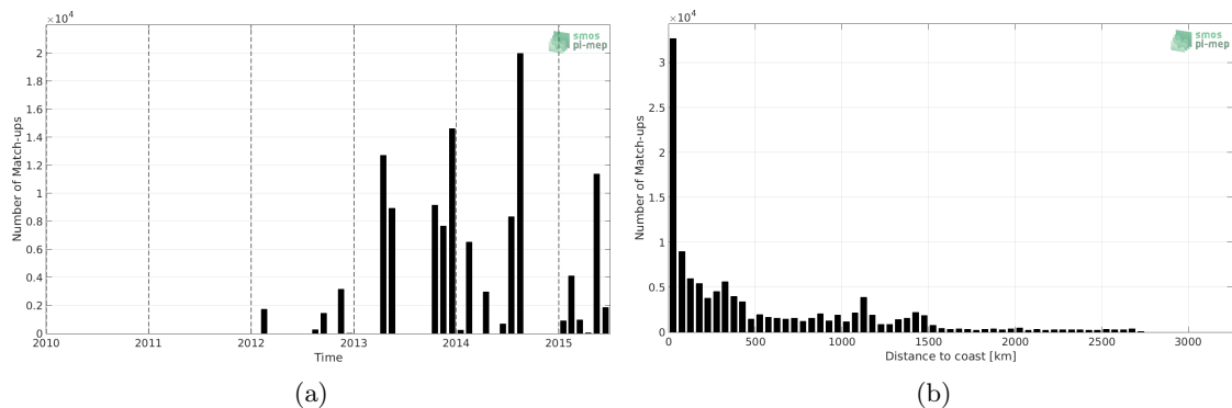
Figure 1: Number of match-ups between TSG-GOSUD-Sailing-ship and Aquarius-L4-IPRC-V5-WEEKLY SSS as a function of time (a) and as function of the distance to coast (b) over the Atlantic Ocean Pi-MEP region and for the full satellite product period.
