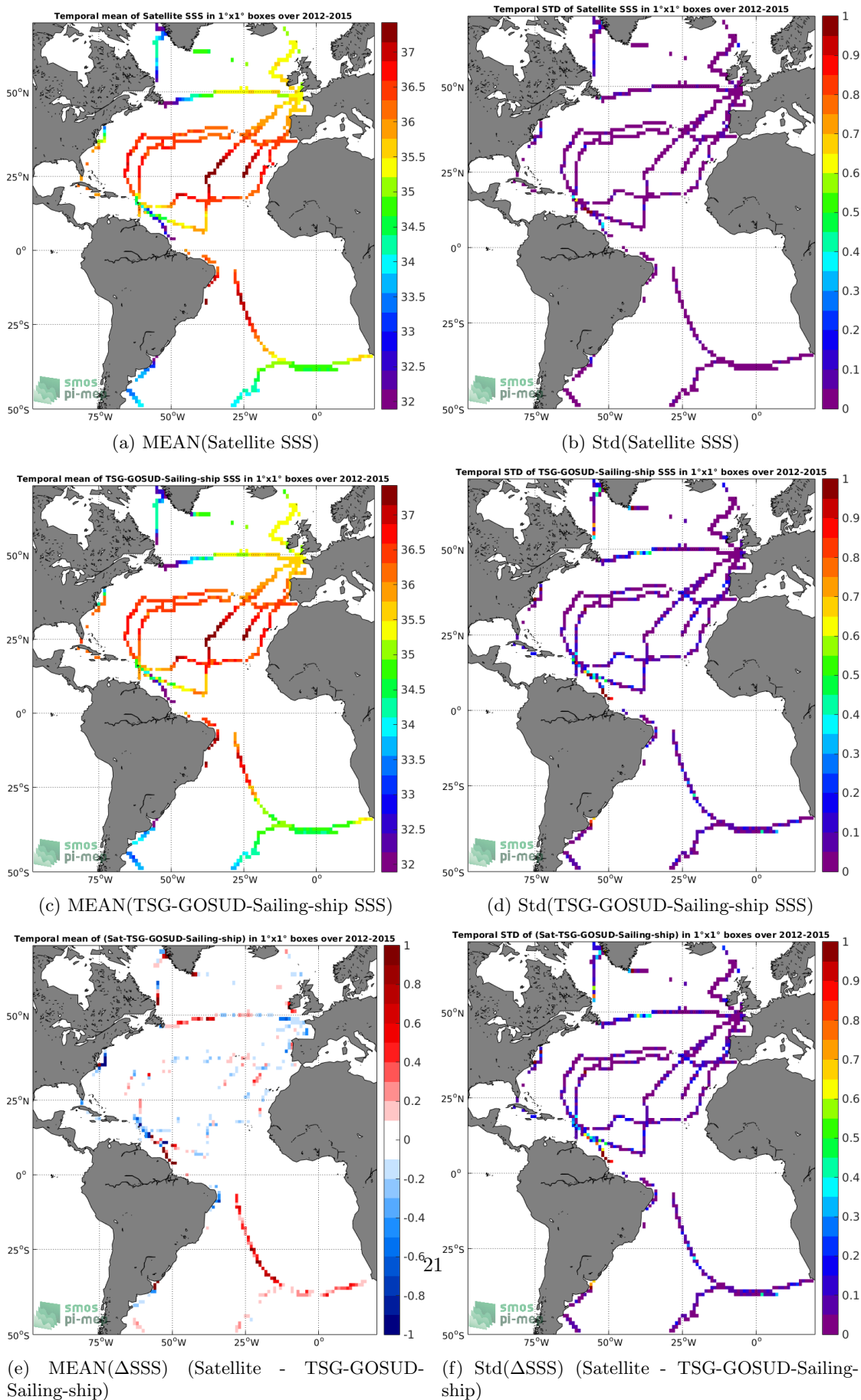
Figure 6: Temporal mean (left) and Std (right) of SSS from Aquarius-L4-IPRC-V5-WEEKLY (top), TSG-GOSUD-Sailing-ship (middle), and of \Delta SSS (Satellite - TSG-GOSUD-Sailing-ship). Only match-up pairs are used to generate these maps.
