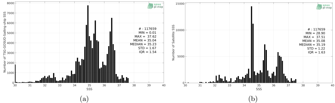
Figure 2: Histograms of SSS from TSG-GOSUD-Sailing-ship (a) and Aquarius-L4-IPRC-V5-WEEKLY (b) considering all match-up pairs per bins of 0.1 over the Atlantic Ocean Pi-MEP region and for the full satellite product period.
