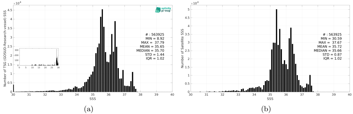
Figure 3: Histograms of SSS from TSG (GOSUD-Research-vessel) (a) and Aquarius SSS L4 OI v5 - Weekly (IPRC) (b) considering all match-up pairs per bins of 0.1 over the Atlantic Ocean Pi-MEP region and for the full satellite product period.
