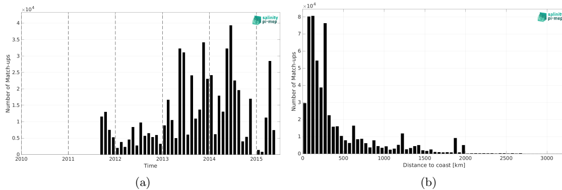
Figure 2: Number of match-ups between TSG (GOSUD-Research-vessel) and Aquarius SSS L4 OI v5 - Weekly (IPRC) SSS as a function of time (a) and as function of the distance to coast (b) over the Atlantic Ocean Pi-MEP region and for the full satellite product period.
