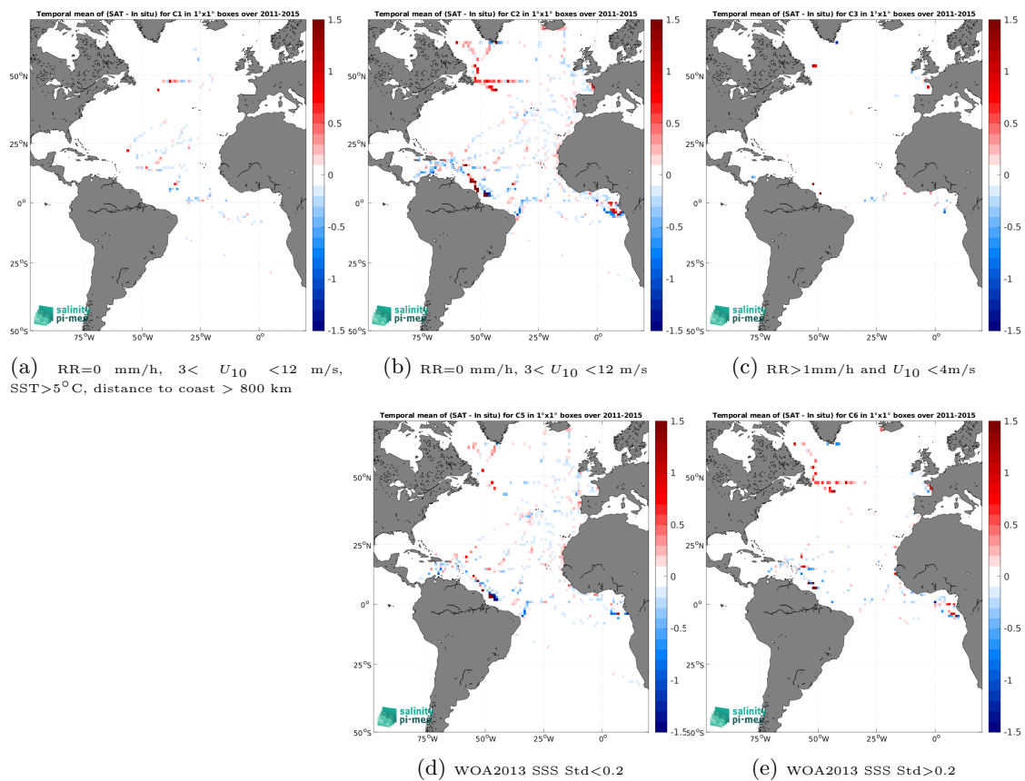
Figure 14: Temporal mean gridded over spatial boxes of size 1^\circ \times 1^\circ of \Delta\text{SSS} (Aquarius SSS L4 OI v5 - Weekly (IPRC) - TSG (GOSUD-Research-vessel)) for 5 different subdatasets corresponding to:RR=0 mm/h, 3 < U_{10} < 12 m/s, SST>5°C, distance to coast > 800 km (a), RR=0 mm/h, 3 < U_{10} < 12 m/s (b), RR>1mm/h and U_{10} < 4 m/s (c), WOA2013 SSS Std<0.2 (d), WOA2013 SSS Std>0.2 (e).
