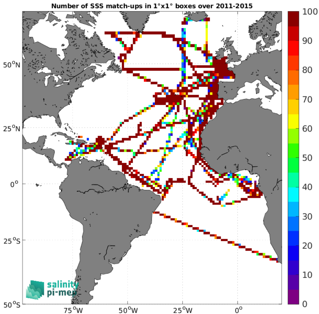
Figure 5: Number of SSS match-ups between TSG (GOSUD-Research-vessel) SSS and the Aquarius SSS L4 OI v5 - Weekly (IPRC) SSS product for the Atlantic Ocean Pi-MEP region over 1^\circ \times 1^\circ boxes and for the full satellite product period.
