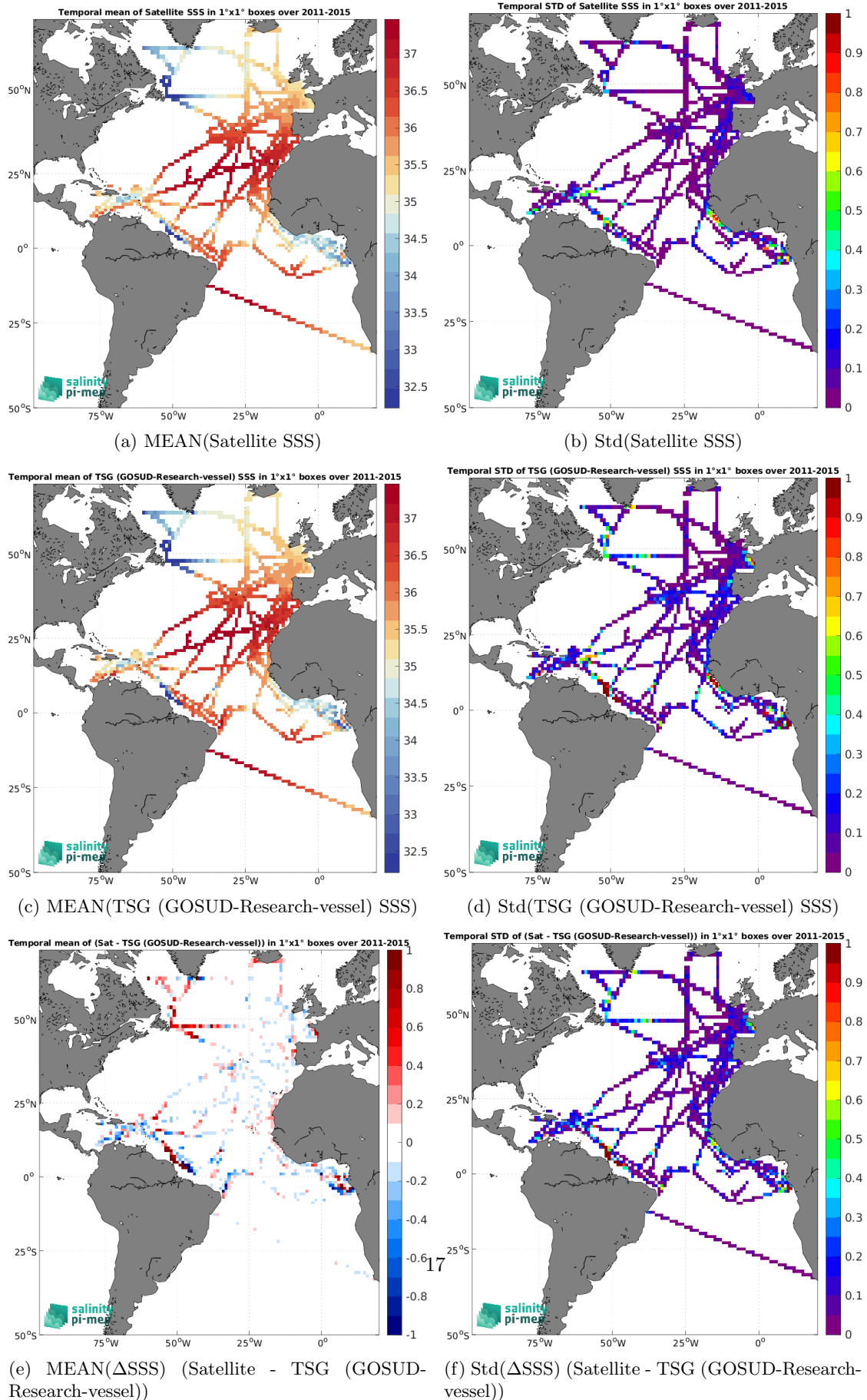
Figure 7: Temporal mean (left) and Std (right) of SSS from Aquarius SSS L4 OI v5 - Weekly (IPRC) (top), TSG (GOSUD-Research-vessel) (middle), and of \Delta SSS (Satellite - TSG (GOSUD-Research-vessel)). Only match-up pairs are used to generate these maps.
