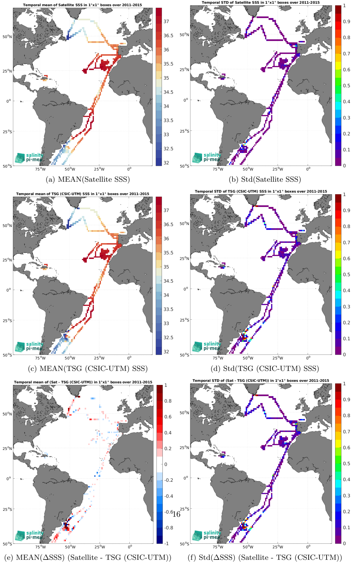
Figure 7: Temporal mean (left) and Std (right) of SSS from Aquarius SSS L4 OI v5 - Weekly (IPRC) (top), TSG (CSIC-UTM) (middle), and of \Delta SSS (Satellite - TSG (CSIC-UTM)). Only match-up pairs are used to generate these maps.
