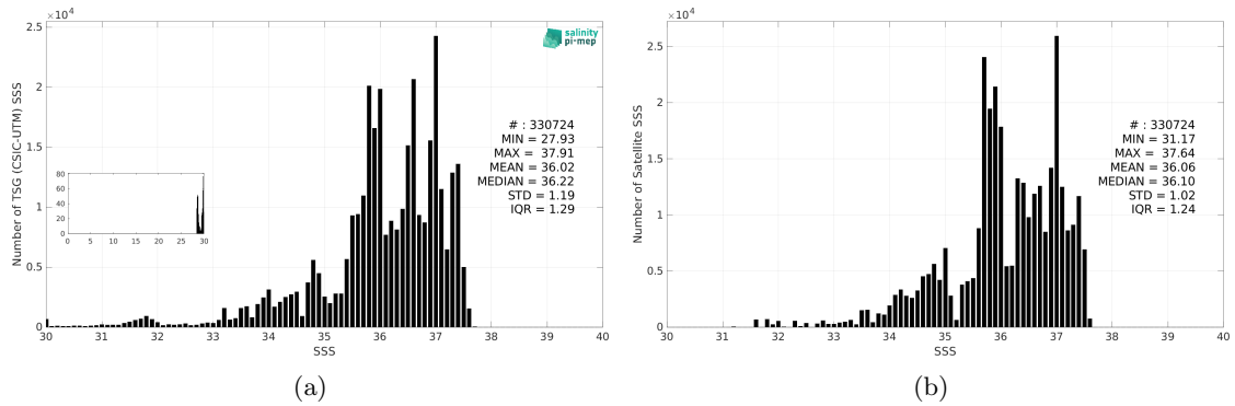
Figure 3: Histograms of SSS from TSG (CSIC-UTM) (a) and Aquarius SSS L4 OI v5 - Weekly (IPRC) (b) considering all match-up pairs per bins of 0.1 over the Atlantic Ocean Pi-MEP region and for the full satellite product period.
