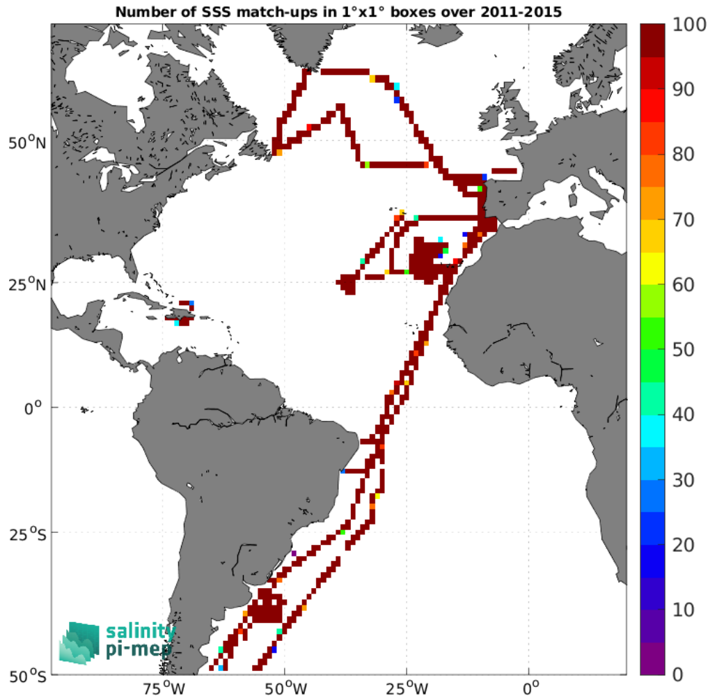
Figure 5: Number of SSS match-ups between TSG (CSIC-UTM) SSS and the Aquarius SSS L4 OI v5 - Weekly (IPRC) SSS product for the Atlantic Ocean Pi-MEP region over 1^\circ \times 1^\circ boxes and for the full satellite product period.
