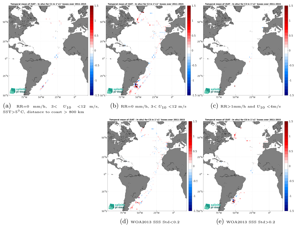
Figure 14: Temporal mean gridded over spatial boxes of size 1^\circ \times 1^\circ of \Delta SSS (Aquarius SSS L4 OI v5 - Weekly (IPRC) - TSG (CSIC-UTM)) for 5 different subdatasets corresponding to:RR=0 mm/h, 3 < U_{10} < 12 m/s, SST >5^\circ\text{C} , distance to coast > 800 km (a), RR=0 mm/h, 3 < U_{10} < 12 m/s (b), RR >1 mm/h and U_{10} < 4 m/s (c), WOA2013 SSS Std <0.2 (d), WOA2013 SSS Std >0.2 (e).
