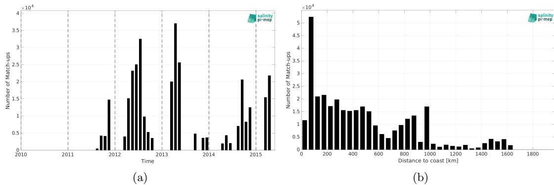
Figure 2: Number of match-ups between TSG (CSIC-UTM) and Aquarius SSS L4 OI v5 - Weekly (IPRC) SSS as a function of time (a) and as function of the distance to coast (b) over the Atlantic Ocean Pi-MEP region and for the full satellite product period.
