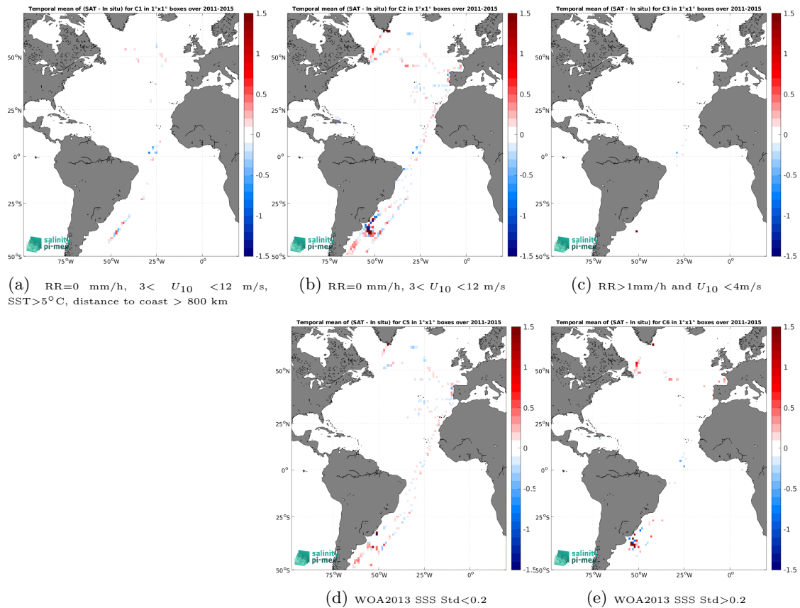
Figure 12: Temporal mean gridded over spatial boxes of size 1^\circ \times 1^\circ of \Delta\text{SSS} (Aquarius SSS L4 OI v5 - Weekly (IPRC) - TSG (CSIC-UTM)) for 5 different subdatasets corresponding to:RR=0 mm/h, 3 < U_{10} < 12 m/s, SST >5^\circ\text{C} , distance to coast > 800 km (a), RR=0 mm/h, 3 < U_{10} < 12 m/s (b), RR >1 mm/h and U_{10} < 4 m/s (c), WOA2013 SSS Std <0.2 (d), WOA2013 SSS Std >0.2 (e).
