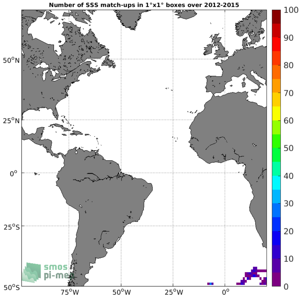
Figure 4: Number of SSS match-ups between Marine mammals SSS and the Aquarius SSS L4 OI v5 - Weekly (IPRC) SSS product for the Atlantic Ocean Pi-MEP region over 1^\circ \times 1^\circ boxes and for the full satellite product period.
