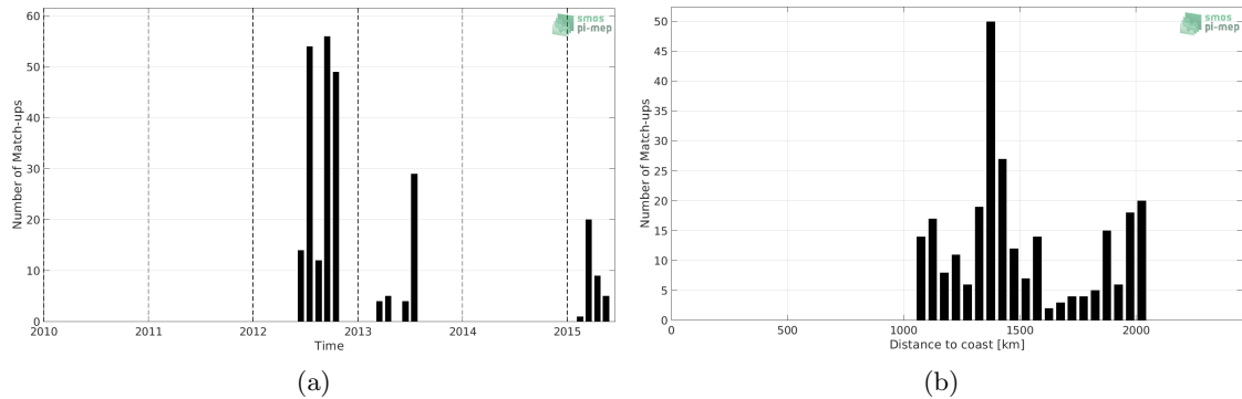
Figure 1: Number of match-ups between Sea mammals and Aquarius SSS L4 OI v5 - Weekly (IPRC) SSS as a function of time (a) and as function of the distance to coast (b) over the Atlantic Ocean Pi-MEP region and for the full satellite product period.
