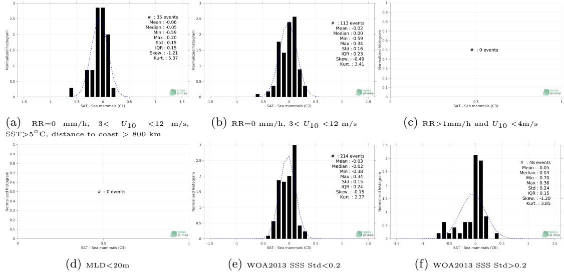
Figure 13: Normalized histogram of \Delta SSS (Aquarius SSS L4 OI v5 - Weekly (IPRC) - Sea mammals) for 6 different subdatasets corresponding to: RR=0 mm/h, 3 < U_{10} < 12 m/s, SST > 5^\circ C , distance to coast > 800 km (a), RR=0 mm/h, 3 < U_{10} < 12 m/s (b), RR > 1 mm/h and U_{10} < 4 m/s (c), MLD < 20 m (d), WOA2013 SSS Std < 0.2 (e), WOA2013 SSS Std > 0.2 (f).
