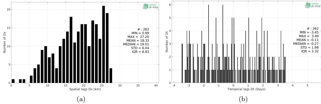
Figure 5: Histograms of the spatial (a) and temporal (b) lags between the location/time of the Sea mammals measurement and the date of the corresponding Aquarius SSS L4 OI v5 - Weekly (IPRC) SSS pixel.
