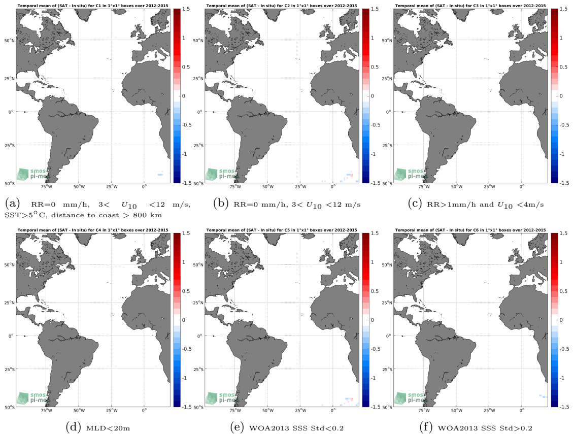
Figure 12: Temporal mean gridded over spatial boxes of size 1°x1° of \Delta SSS (Aquarius-L4-IPRC-V5-WEEKLY - Sea mammals) for 6 different subdatasets corresponding to:RR=0 mm/h, 3 < U_{10} < 12 m/s, SST>5°C, distance to coast > 800 km (a), RR=0 mm/h, 3 < U_{10} < 12 m/s (b), RR>1mm/h and U_{10} < 4 m/s (c),MLD<20m (d),WOA2013 SSS Std<0.2 (e),WOA2013 SSS Std>0.2 (f).
