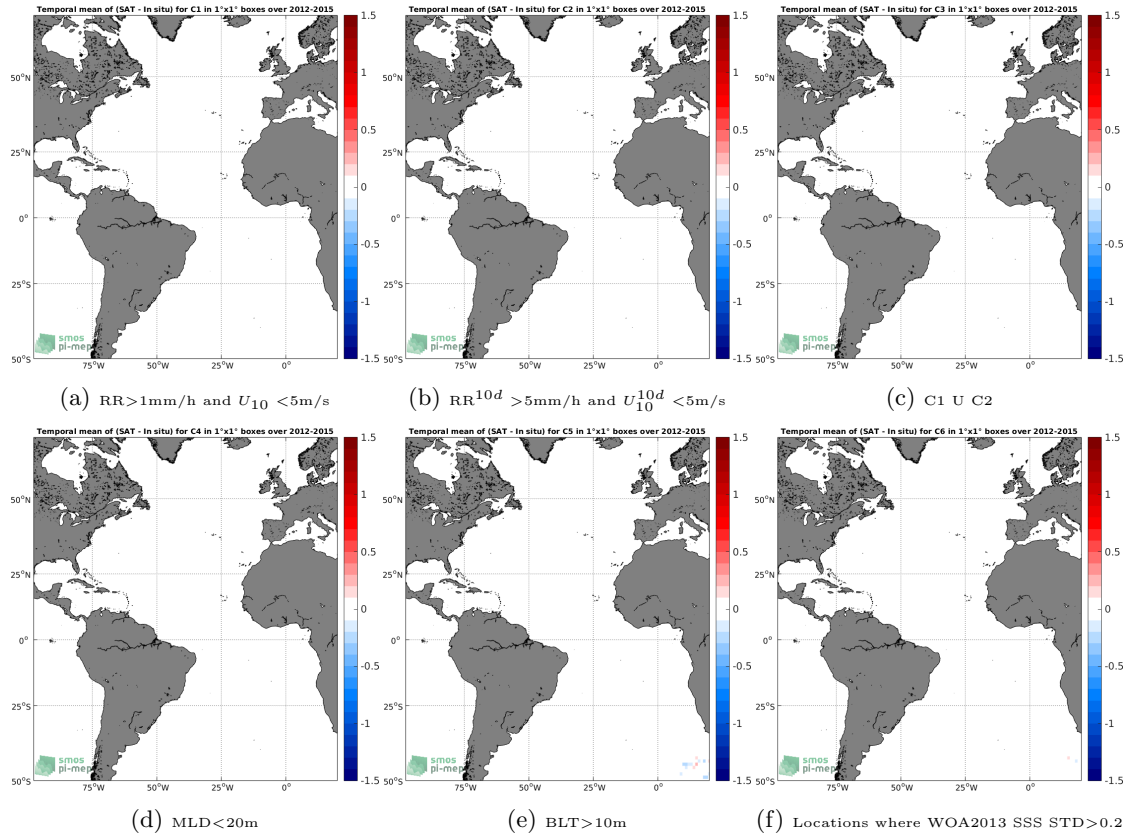
Figure 12: Temporal mean gridded over spatial boxes of size 1^\circ \times 1^\circ of \Delta\text{SSS} (Aquarius-L4-IPRC-V5-WEEKLY - Sea mammals) for 6 different subdatasets corresponding to: \text{RR} > 1\text{mm/h} and U_{10} < 5\text{m/s} (a), \text{RR}^{10d} > 5\text{mm/h} and U_{10}^{10d} < 5\text{m/s} (b), C1 U C2 (c), \text{MLD} < 20\text{m} (d), \text{BLT} > 10\text{m} (e), Locations where WOA2013 SSS STD > 0.2 (f).
