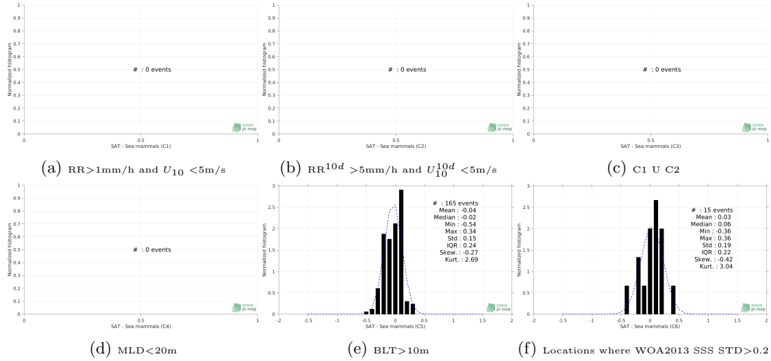
Figure 13: Normalized histogram of \Delta\text{SSS} (Aquarius-L4-IPRC-V5-WEEKLY - Sea mammals) for 6 different subdatasets corresponding to: RR>1mm/h and U_{10} < 5\text{m/s} (a), RR 10d >5mm/h and U_{10}^{10d} < 5\text{m/s} (b), C1 U C2 (c),MLD<20m (d),BLT>10m (e),Locations where WOA2013 SSS STD>0.2 (f).
