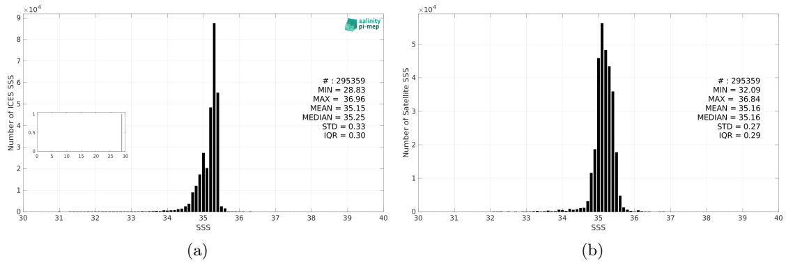
Figure 3: Histograms of SSS from ICES (a) and Aquarius SSS L4 OI v5 - Weekly (IPRC) (b) considering all match-up pairs per bins of 0.1 over the Atlantic Ocean Pi-MEP region and for the full satellite product period.
