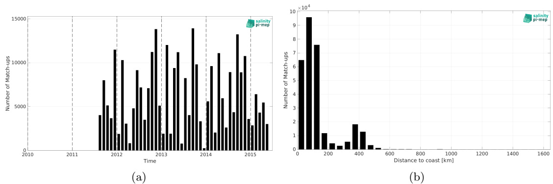
Figure 2: Number of match-ups between ICES and Aquarius SSS L4 OI v5 - Weekly (IPRC) SSS as a function of time (a) and as function of the distance to coast (b) over the Atlantic Ocean Pi-MEP region and for the full satellite product period.
