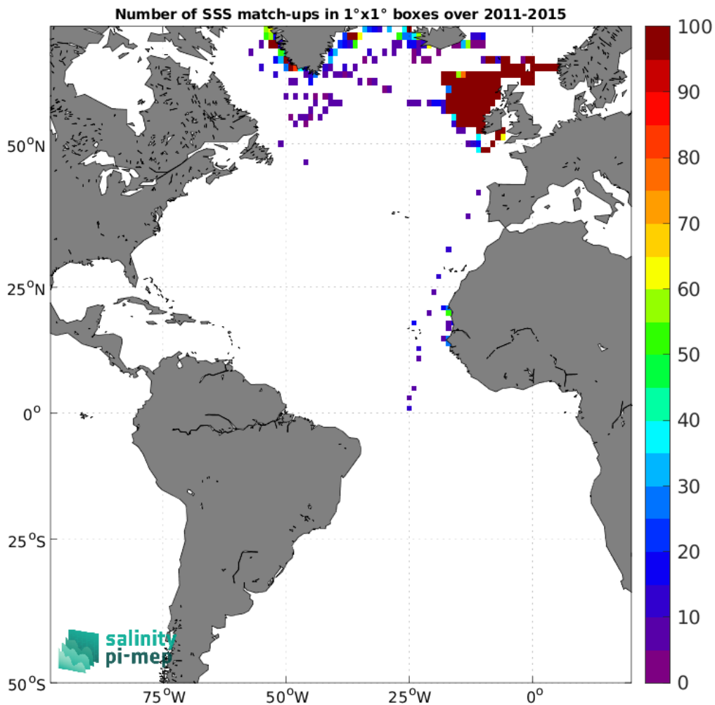
Figure 5: Number of SSS match-ups between ICES SSS and the Aquarius SSS L4 OI v5 - Weekly (IPRC) SSS product for the Atlantic Ocean Pi-MEP region over 1°x1° boxes and for the full satellite product period.
