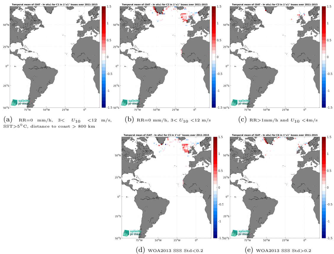
Figure 14: Temporal mean gridded over spatial boxes of size 1^\circ \times 1^\circ of \Delta\text{SSS} (Aquarius SSS L4 OI v5 - Weekly (IPRC) - ICES) for 5 different subdatasets corresponding to:RR=0 mm/h, 3 < U_{10} < 12 m/s, SST>5°C, distance to coast > 800 km (a), RR=0 mm/h, 3 < U_{10} < 12 m/s (b), RR>1mm/h and U_{10} < 4 m/s (c), WOA2013 SSS Std<0.2 (d), WOA2013 SSS Std>0.2 (e).
