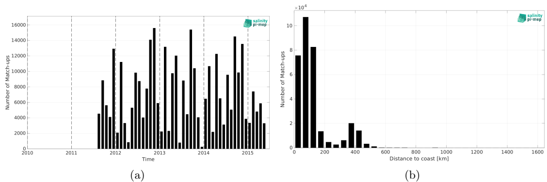
Figure 1: Number of match-ups between ICES and Aquarius SSS L4 OI v5 - Weekly (IPRC) SSS as a function of time (a) and as function of the distance to coast (b) over the Atlantic Ocean Pi-MEP region and for the full satellite product period.
