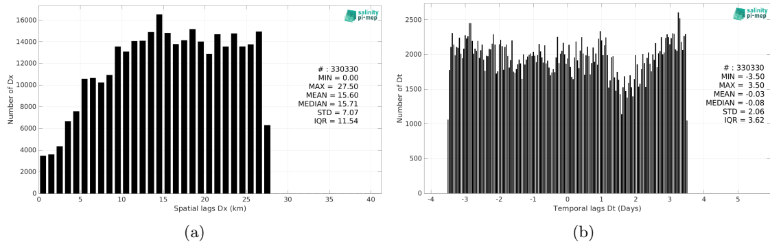
Figure 5: Histograms of the spatial (a) and temporal (b) lags between the location/time of the ICES measurement and the date of the corresponding Aquarius SSS L4 OI v5 - Weekly (IPRC) SSS pixel.
