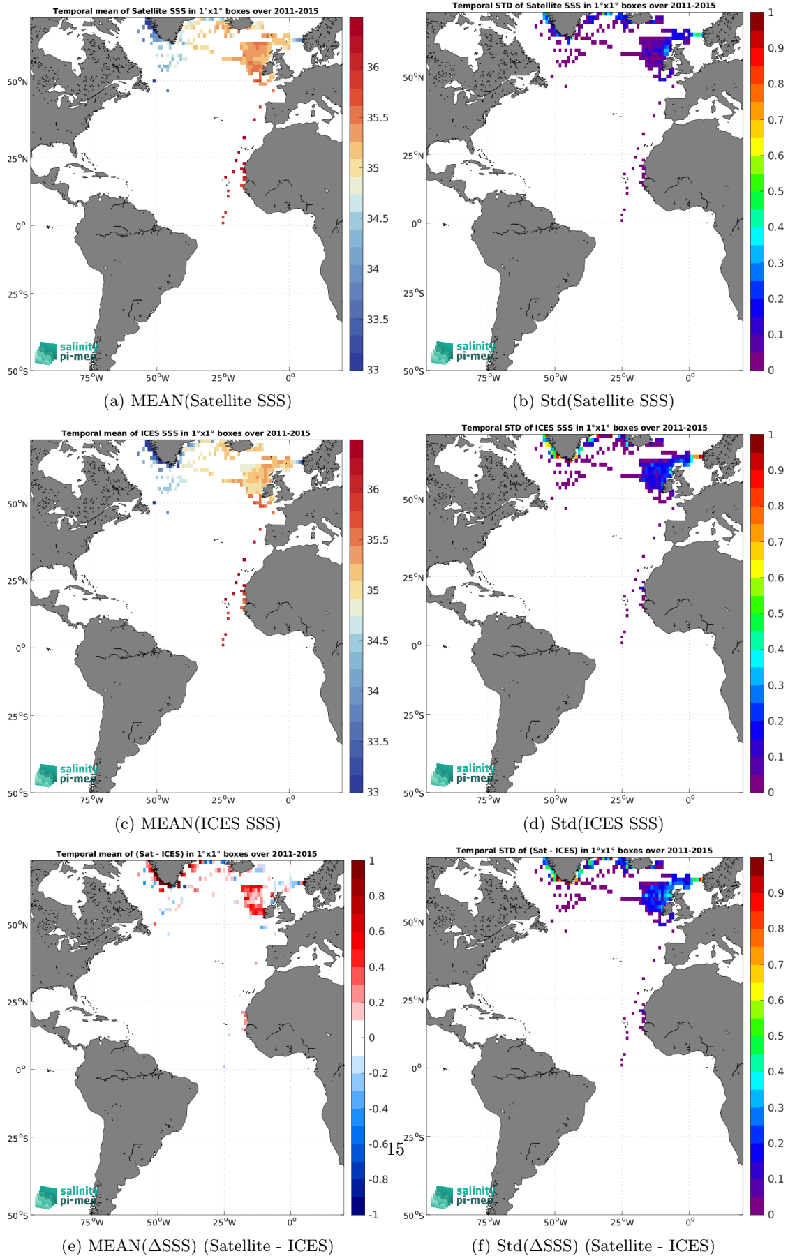
Figure 6: Temporal mean (left) and Std (right) of SSS from Aquarius SSS L4 OI v5 - Weekly (IPRC) (top), ICES (middle), and of \Delta SSS (Satellite - ICES). Only match-up pairs are used to generate these maps.
