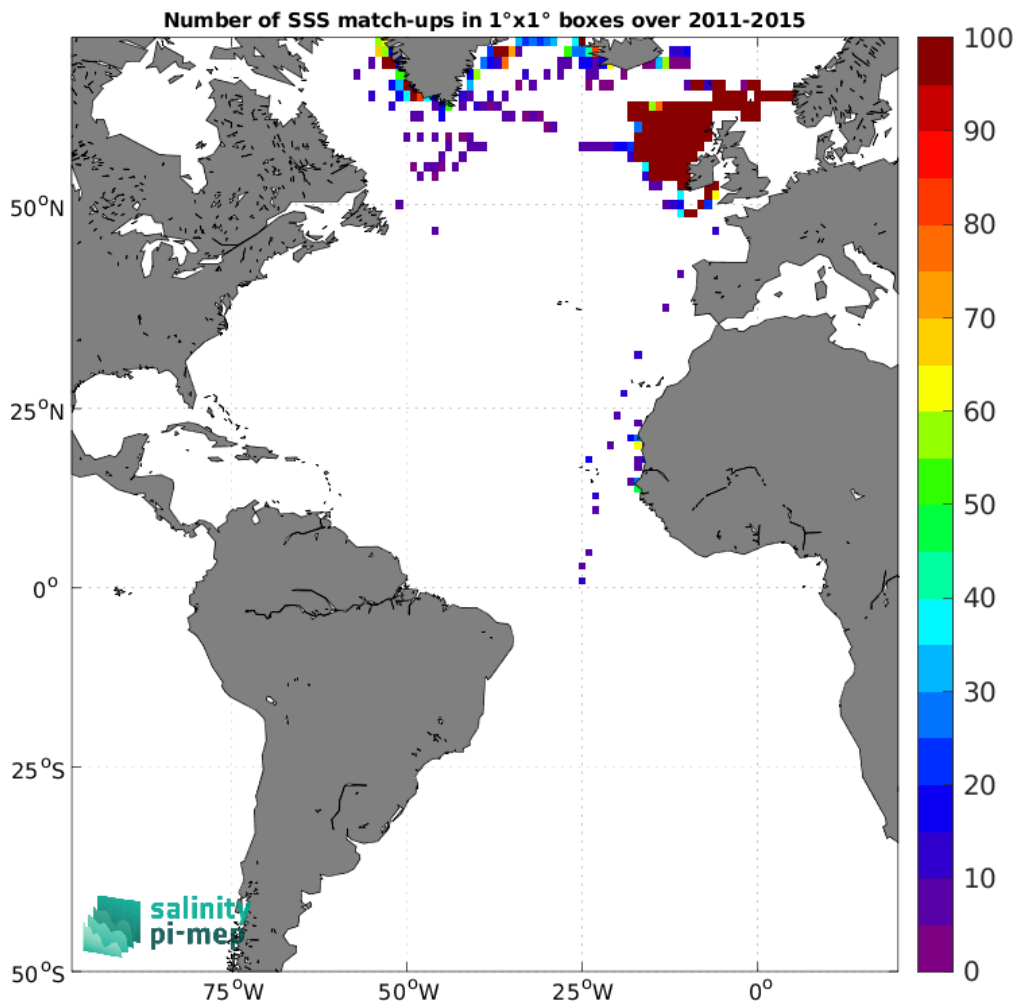
Figure 4: Number of SSS match-ups between ICES SSS and the Aquarius SSS L4 OI v5 - Weekly (IPRC) SSS product for the Atlantic Ocean Pi-MEP region over 1°×1° boxes and for the full satellite product period.
