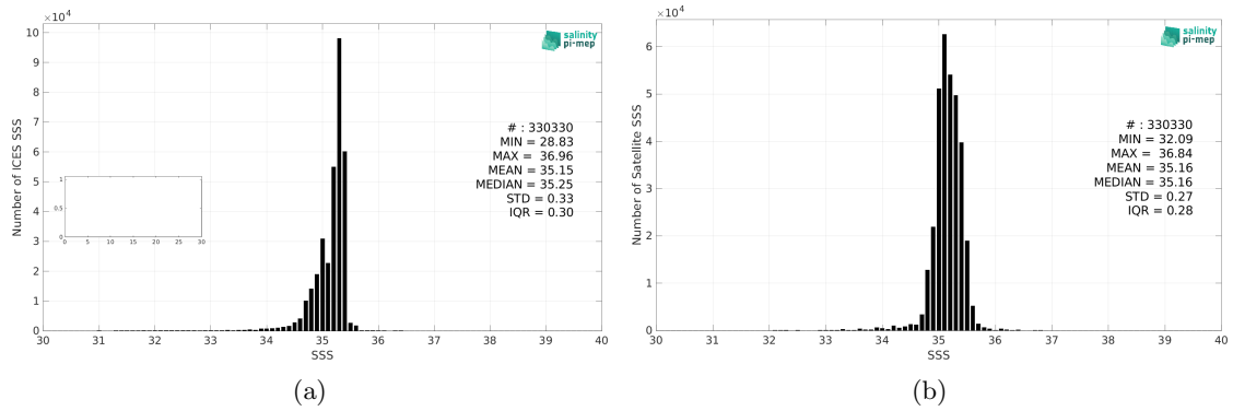
Figure 2: Histograms of SSS from ICES (a) and Aquarius SSS L4 OI v5 - Weekly (IPRC) (b) considering all match-up pairs per bins of 0.1 over the Atlantic Ocean Pi-MEP region and for the full satellite product period.
