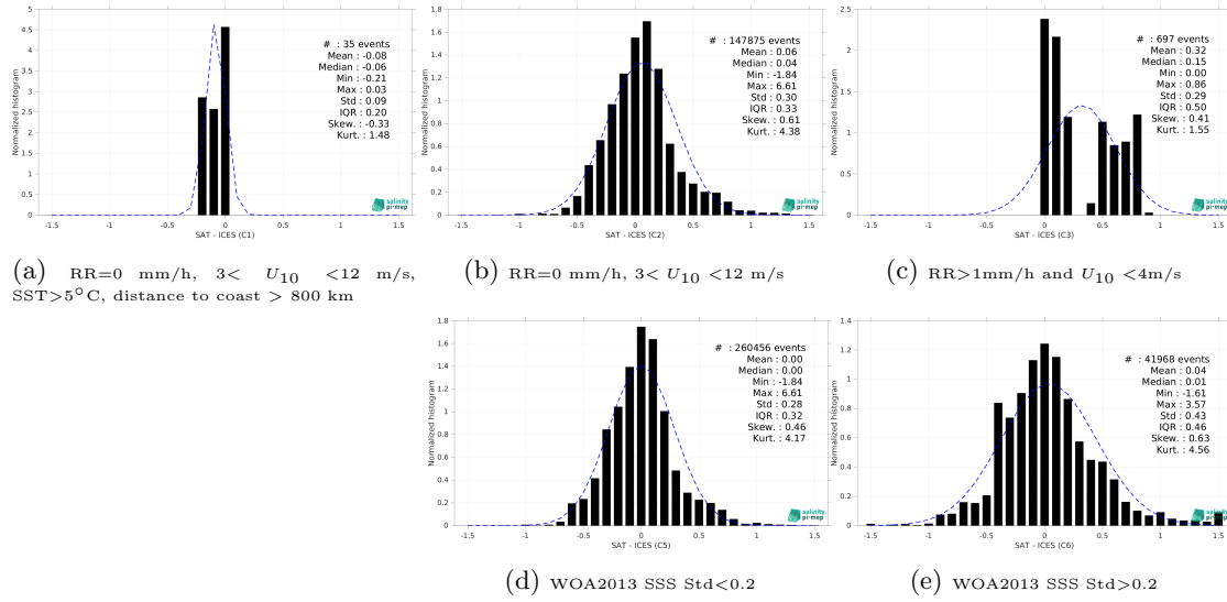
Figure 13: Normalized histogram of \Delta SSS (Aquarius SSS L4 OI v5 - Weekly (IPRC) - ICES) for 5 different subdatasets corresponding to: RR=0 mm/h, 3 < U_{10} < 12 m/s, SST>5°C, distance to coast > 800 km (a), RR=0 mm/h, 3 < U_{10} < 12 m/s (b), RR>1mm/h and U_{10} < 4 m/s (c), WOA2013 SSS Std<0.2 (d), WOA2013 SSS Std>0.2 (e).
