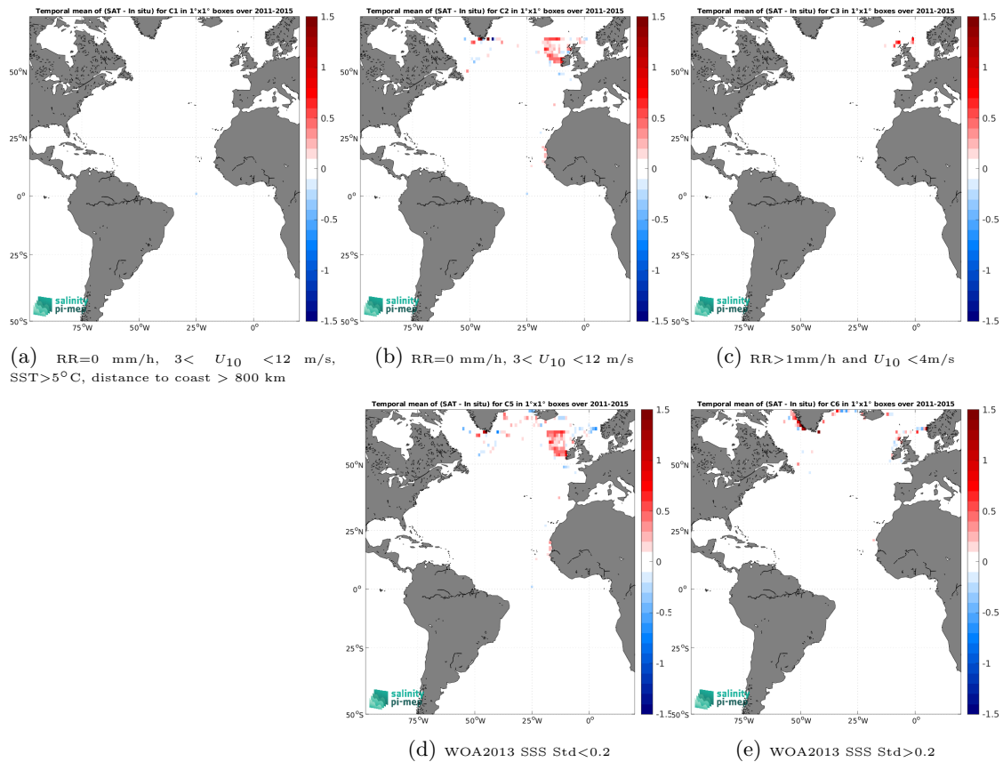
Figure 12: Temporal mean gridded over spatial boxes of size 1^\circ \times 1^\circ of \Delta SSS (Aquarius SSS L4 OI v5 - Weekly (IPRC) - ICES) for 5 different subdatasets corresponding to:RR=0 mm/h, 3 < U_{10} < 12 m/s, SST >5^\circ\text{C} , distance to coast > 800 km (a), RR=0 mm/h, 3 < U_{10} < 12 m/s (b), RR >1 mm/h and U_{10} < 4 m/s (c), WOA2013 SSS Std <0.2 (d), WOA2013 SSS Std >0.2 (e).
