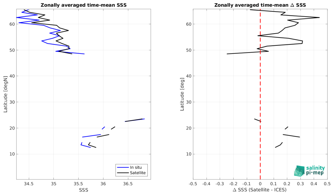
Figure 8: Left panel: Zonal mean SSS from Aquarius SSS L4 OI v5 - Weekly (IPRC) satellite product (black) and from ICES (blue). Right panel: Zonal mean of \Delta SSS (Satellite - ICES) for all the collected Pi-MEP match-up pairs estimated over the full satellite product period.
