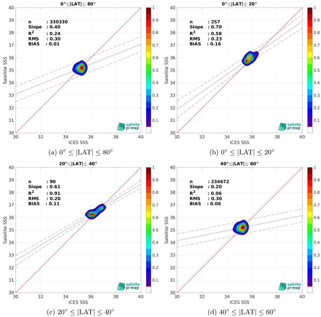
Figure 9: Contour maps of the concentration of Aquarius SSS L4 OI v5 - Weekly (IPRC) SSS (y-axis) versus ICES SSS (x-axis) at match-up pairs for different latitude bands. For each plot, the red line shows x=y . The black thin and dashed lines indicate a linear fit through the data cloud and the \pm 95\% confidence levels, respectively. The number match-up pairs n , the slope and R^2 coefficient of the linear fit, the root mean square (RMS) and the mean bias between satellite and in situ data are indicated for each latitude band in each plots.
