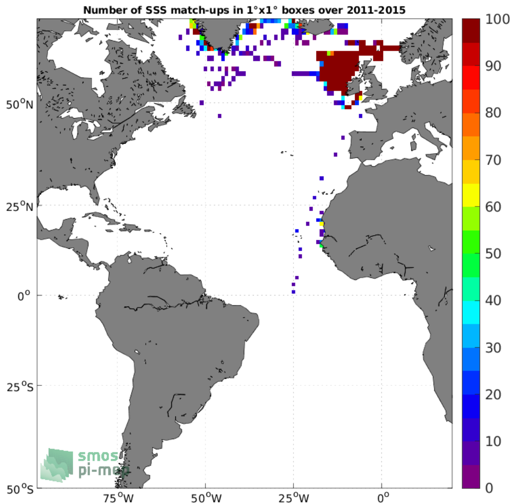
Figure 4: Number of SSS match-ups between ICES SSS and the Aquarius SSS L4 OI v5 - Weekly (IPRC) SSS product for the Atlantic Ocean Pi-MEP region over 1^\circ \times 1^\circ boxes and for the full satellite product period.
