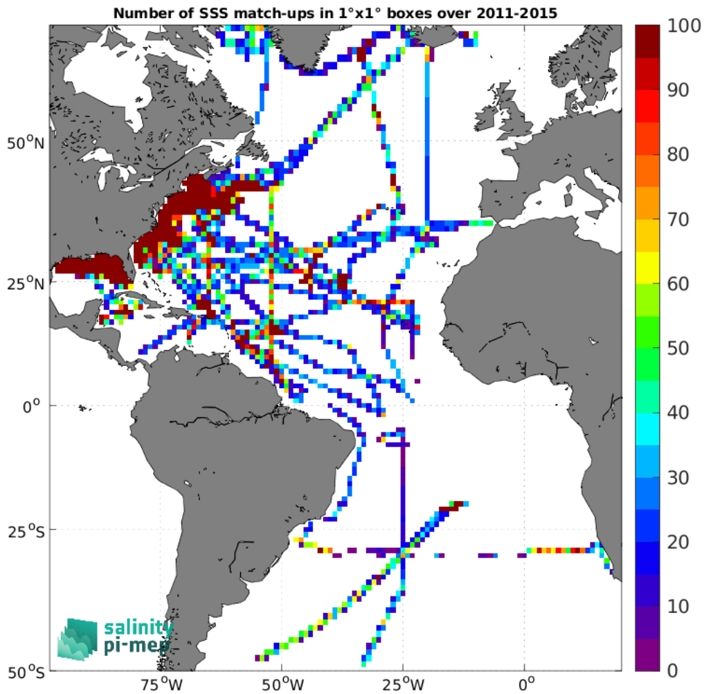
Figure 4: Number of SSS match-ups between TSG (SAMOS) SSS and the Aquarius SSS L4 OI v5 - Monthly (IPRC) SSS product for the Atlantic Ocean Pi-MEP region over 1^\circ \times 1^\circ boxes and for the full satellite product period.
