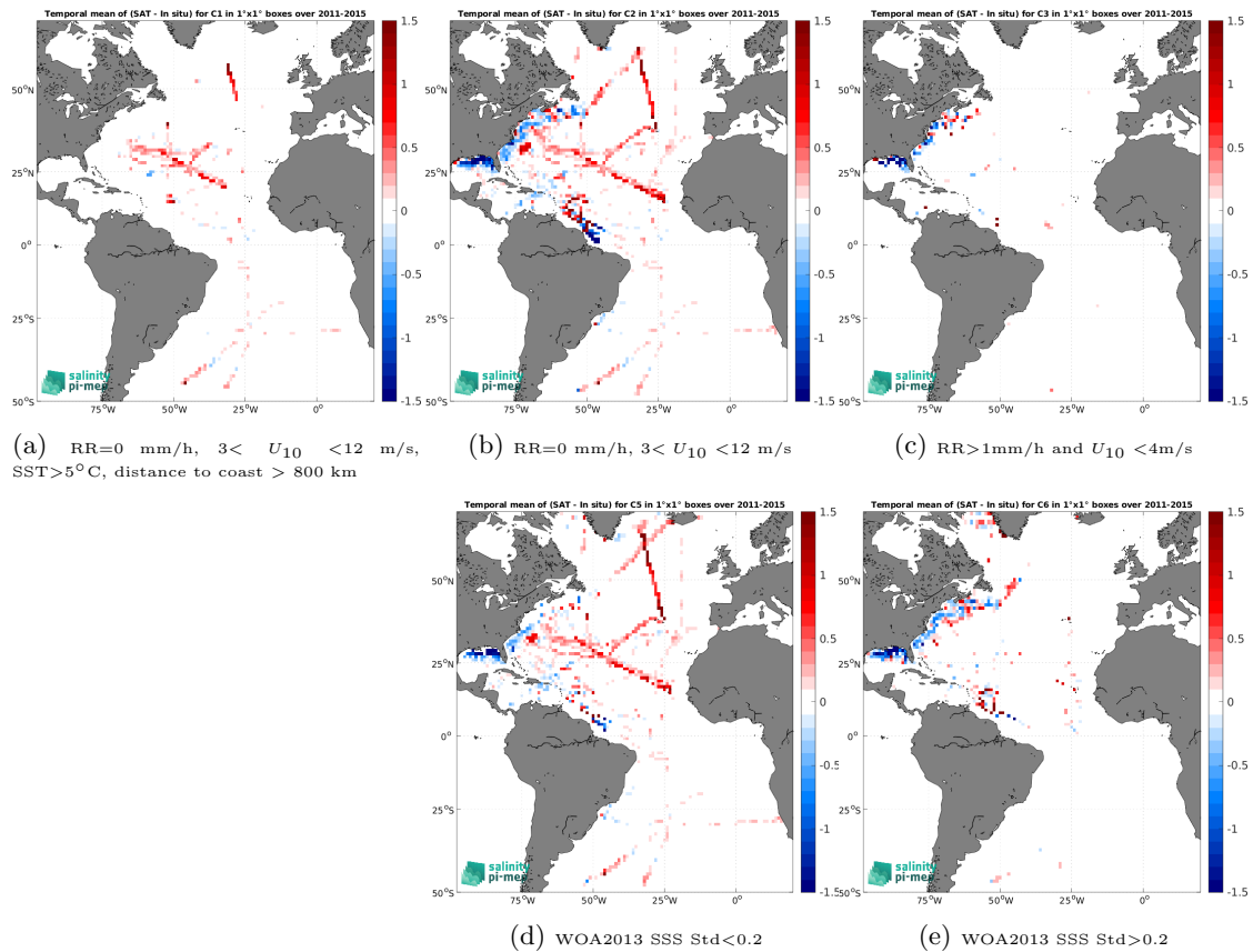
Figure 12: Temporal mean gridded over spatial boxes of size 1^\circ \times 1^\circ of \Delta SSS (Aquarius SSS L4 OI v5 - Monthly (IPRC) - TSG (SAMOS)) for 5 different subdatasets corresponding to:RR=0 mm/h, 3 < U_{10} < 12 m/s, SST >5^\circ\text{C} , distance to coast > 800 km (a), RR=0 mm/h, 3 < U_{10} < 12 m/s (b), RR >1 mm/h and U_{10} < 4 m/s (c), WOA2013 SSS Std <0.2 (d), WOA2013 SSS Std >0.2 (e).
