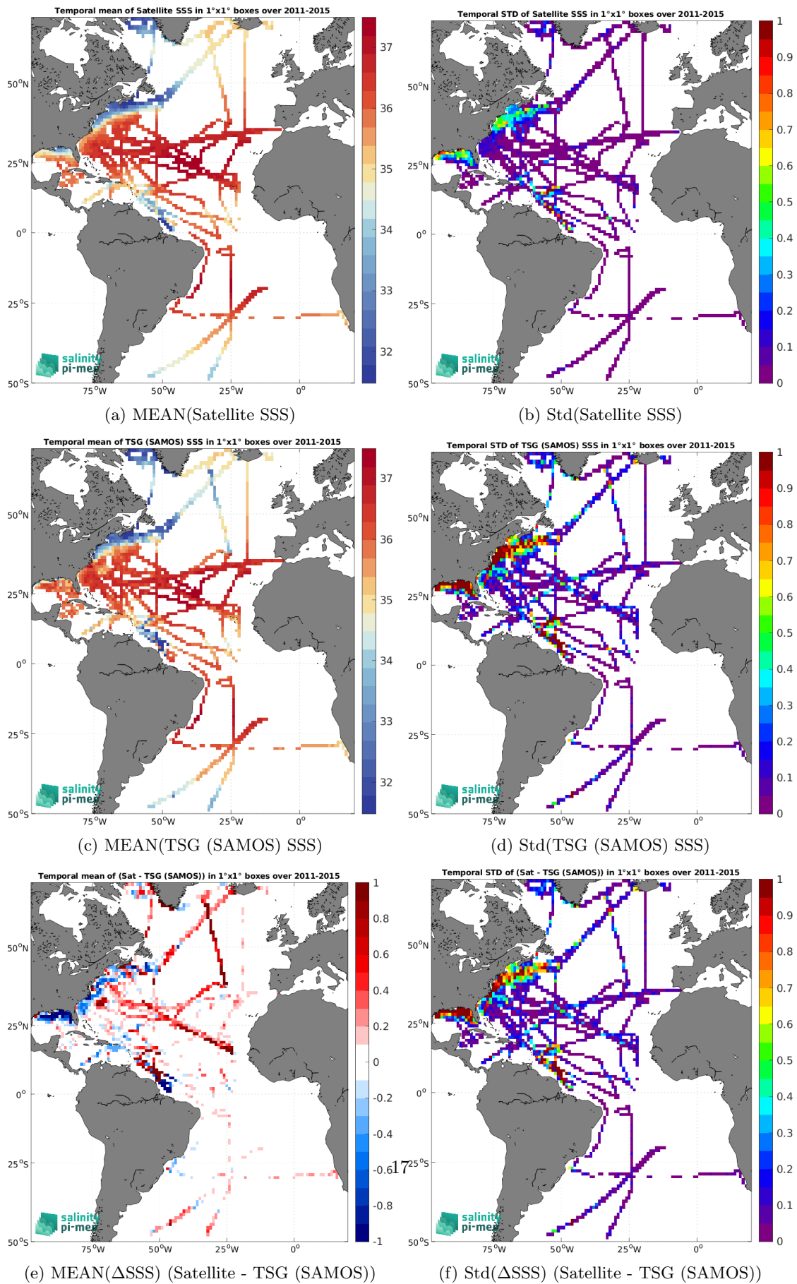
Figure 6: Temporal mean (left) and Std (right) of SSS from Aquarius SSS L4 OI v5 - Monthly (IPRC) (top), TSG (SAMOS) (middle), and of \Delta SSS (Satellite - TSG (SAMOS)). Only match-up pairs are used to generate these maps.
