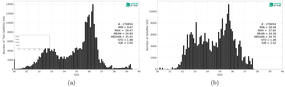
Figure 2: Histograms of SSS from TSG (SAMOS) (a) and Aquarius SSS L4 OI v5 - Monthly (IPRC) (b) considering all match-up pairs per bins of 0.1 over the Atlantic Ocean Pi-MEP region and for the full satellite product period.
