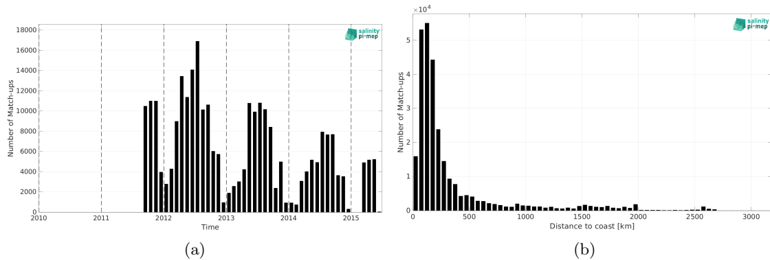
Figure 1: Number of match-ups between TSG (SAMOS) and Aquarius SSS L4 OI v5 - Monthly (IPRC) SSS as a function of time (a) and as function of the distance to coast (b) over the Atlantic Ocean Pi-MEP region and for the full satellite product period.
