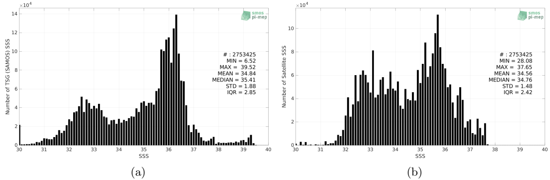
Figure 2: Histograms of SSS from TSG (SAMOS) (a) and Aquarius SSS L4 OI v5 - Monthly (IPRC) (b) considering all match-up pairs per bins of 0.1 over the Atlantic Ocean Pi-MEP region and for the full satellite product period.
