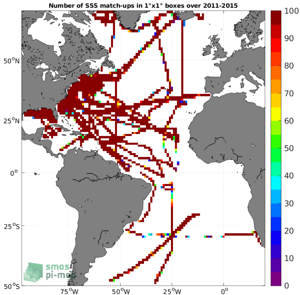
Figure 4: Number of SSS match-ups between TSG (SAMOS) SSS and the Aquarius SSS L4 OI v5 - Monthly (IPRC) SSS product for the Atlantic Ocean Pi-MEP region over 1°x1° boxes and for the full satellite product period.
