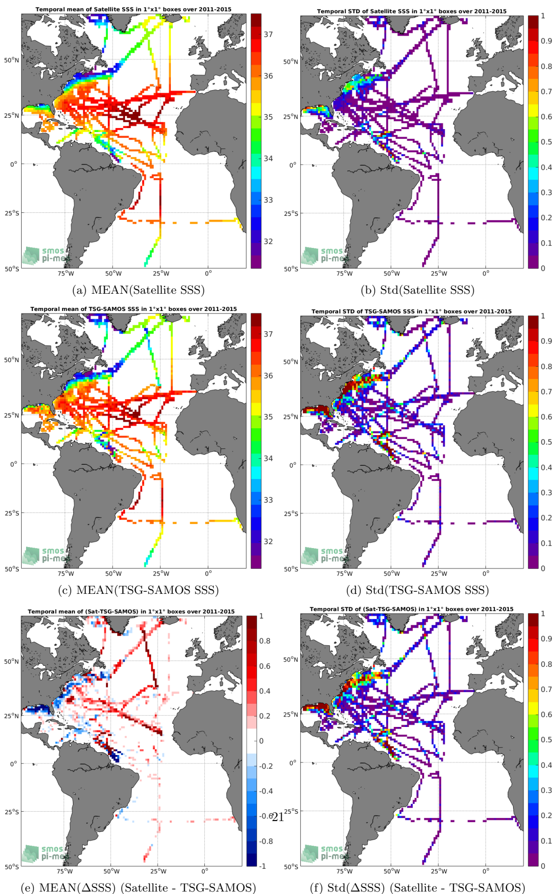
Figure 6: Temporal mean (left) and Std (right) of SSS from Aquarius-L4-IPRC-V5-MONTHLY (top), TSG-SAMOS (middle), and of \Delta SSS (Satellite - TSG-SAMOS). Only match-up pairs are used to generate these maps.
