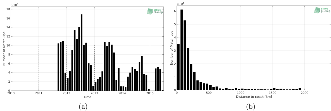
Figure 1: Number of match-ups between TSG-SAMOS and Aquarius-L4-IPRC-V5-MONTHLY SSS as a function of time (a) and as function of the distance to coast (b) over the Atlantic Ocean Pi-MEP region and for the full satellite product period.
