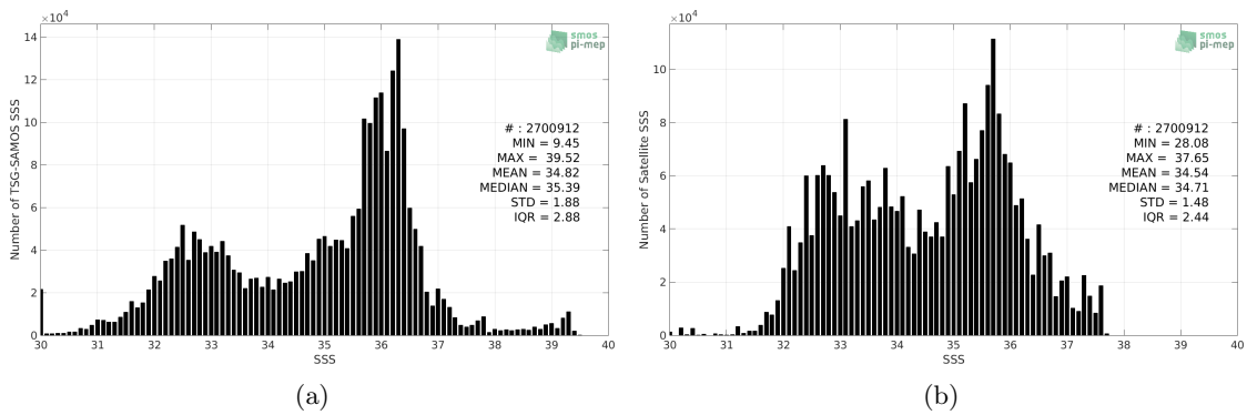
Figure 2: Histograms of SSS from TSG-SAMOS (a) and Aquarius-L4-IPRC-V5-MONTHLY (b) considering all match-up pairs per bins of 0.1 over the Atlantic Ocean Pi-MEP region and for the full satellite product period.
