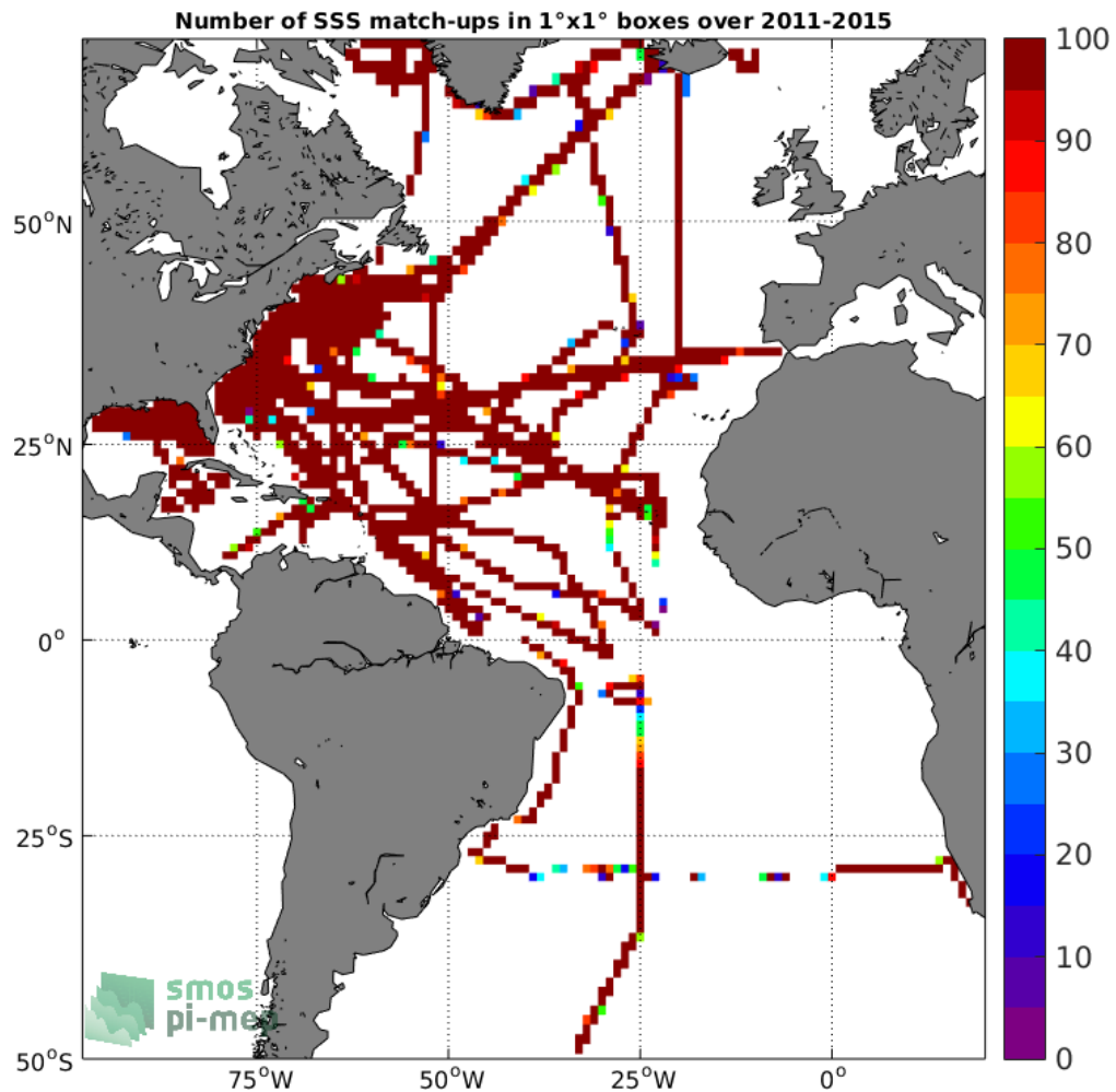
Figure 4: Number of SSS match-ups between TSG-SAMOS SSS and the Aquarius-L4-IPRC-V5-MONTHLY SSS product for the Atlantic Ocean Pi-MEP region over 1°x1° boxes and for the full satellite product period.
