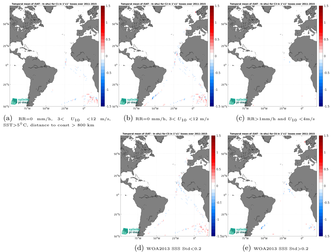
Figure 14: Temporal mean gridded over spatial boxes of size 1^\circ \times 1^\circ of \Delta\text{SSS} (Aquarius SSS L4 OI v5 - Monthly (IPRC) - TSG (Polarstern)) for 5 different subdatasets corresponding to:RR=0 mm/h, 3 < U_{10} < 12 m/s, SST>5°C, distance to coast > 800 km (a), RR=0 mm/h, 3 < U_{10} < 12 m/s (b), RR>1mm/h and U_{10} < 4 m/s (c), WOA2013 SSS Std<0.2 (d), WOA2013 SSS Std>0.2 (e).
