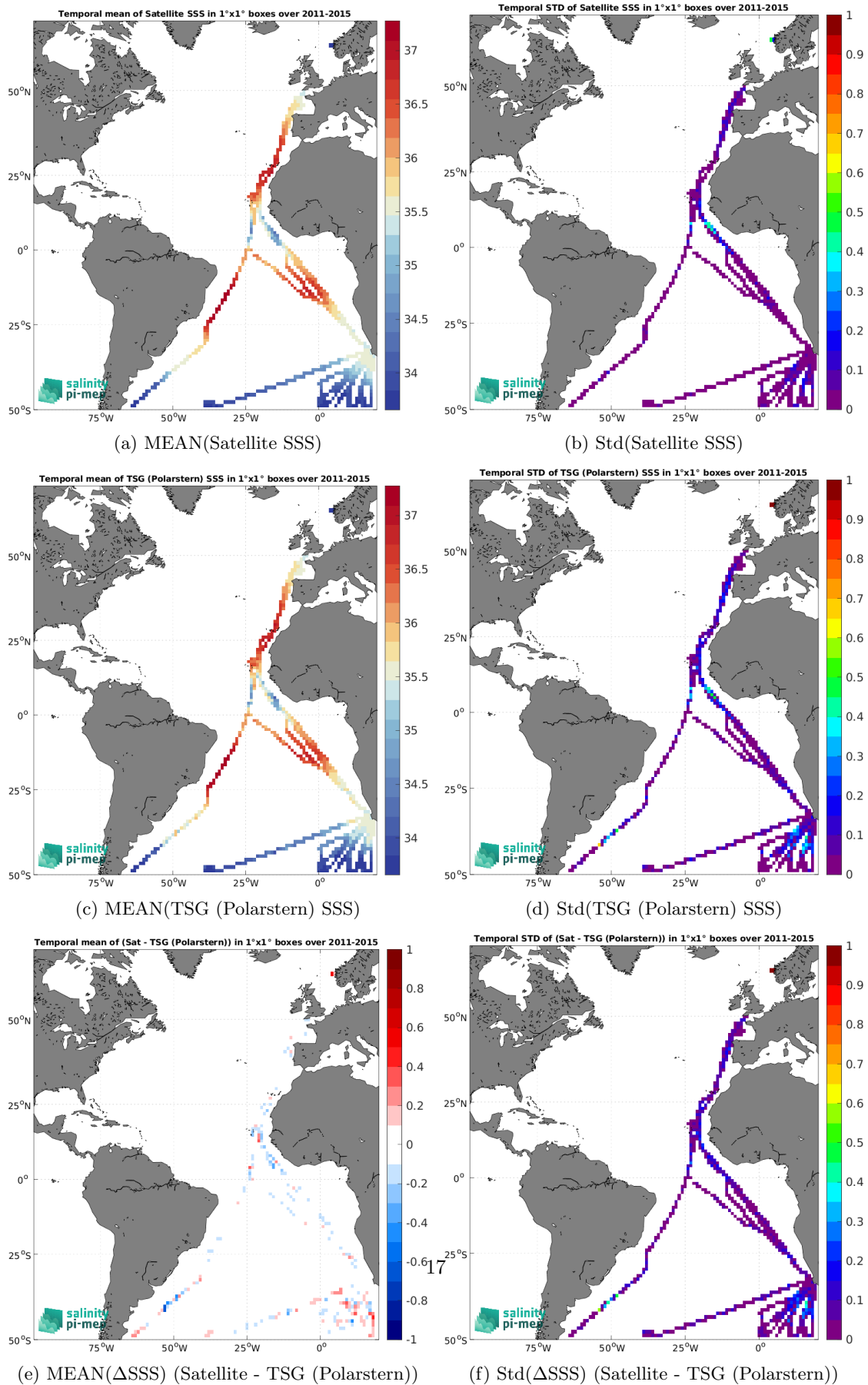
Figure 7: Temporal mean (left) and Std (right) of SSS from Aquarius SSS L4 OI v5 - Monthly (IPRC) (top), TSG (Polarstern) (middle), and of \Delta SSS (Satellite - TSG (Polarstern)). Only match-up pairs are used to generate these maps.
