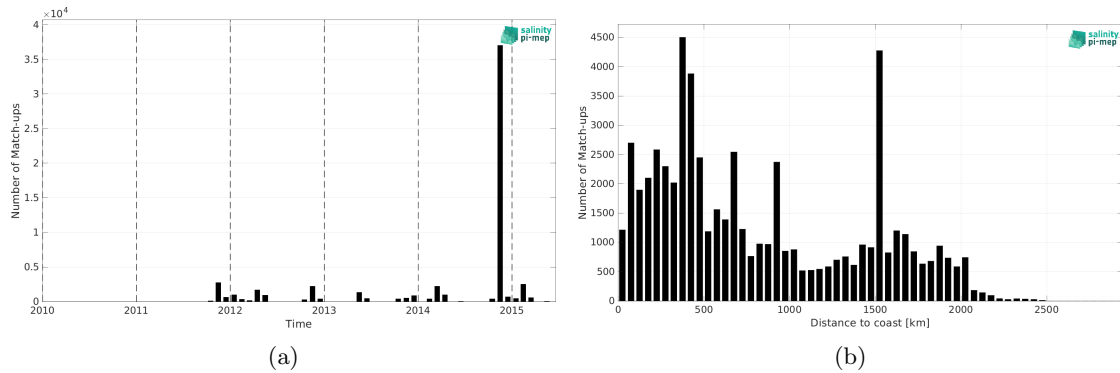
Figure 2: Number of match-ups between TSG (Polarstern) and Aquarius SSS L4 OI v5 - Monthly (IPRC) SSS as a function of time (a) and as function of the distance to coast (b) over the Atlantic Ocean Pi-MEP region and for the full satellite product period.
