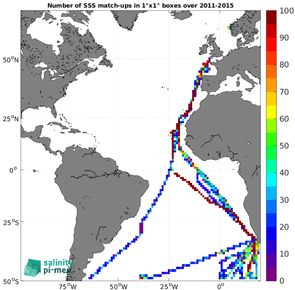
Figure 5: Number of SSS match-ups between TSG (Polarstern) SSS and the Aquarius SSS L4 OI v5 - Monthly (IPRC) SSS product for the Atlantic Ocean Pi-MEP region over 1°x1° boxes and for the full satellite product period.
