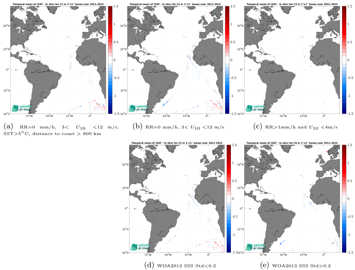
Figure 14: Temporal mean gridded over spatial boxes of size 1^\circ \times 1^\circ of \Delta SSS (Aquarius SSS L4 OI v5 - Monthly (IPRC) - TSG (Polarstern)) for 5 different subdatasets corresponding to:RR=0 mm/h, 3 < U_{10} < 12 m/s, SST >5^\circ\text{C} , distance to coast > 800 km (a), RR=0 mm/h, 3 < U_{10} < 12 m/s (b), RR >1 mm/h and U_{10} < 4 m/s (c), WOA2013 SSS Std <0.2 (d), WOA2013 SSS Std >0.2 (e).
