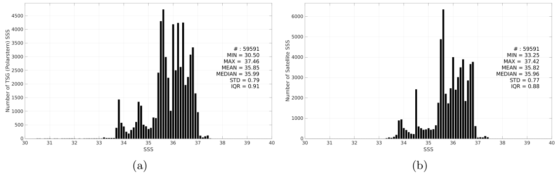
Figure 3: Histograms of SSS from TSG (Polarstern) (a) and Aquarius SSS L4 OI v5 - Monthly (IPRC) (b) considering all match-up pairs per bins of 0.1 over the Atlantic Ocean Pi-MEP region and for the full satellite product period.
