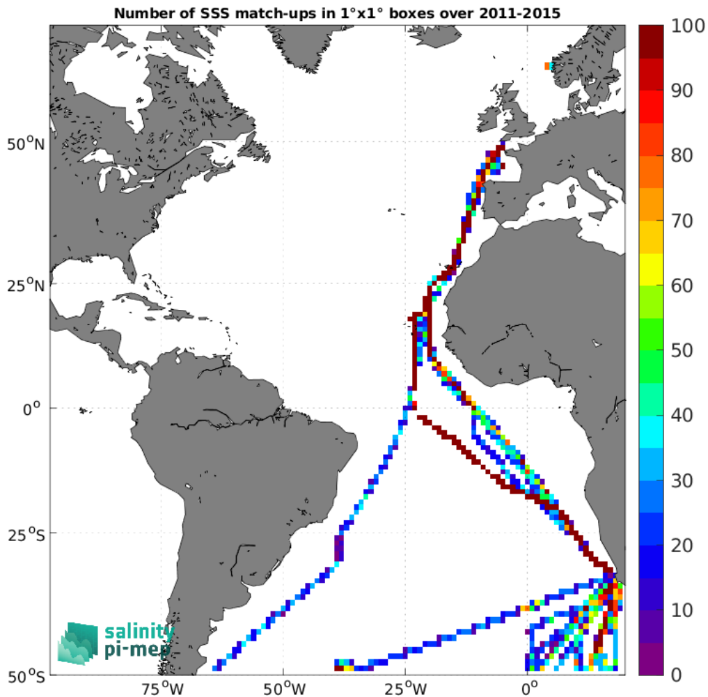
Figure 4: Number of SSS match-ups between TSG (Polarstern) SSS and the Aquarius SSS L4 OI v5 - Monthly (IPRC) SSS product for the Atlantic Ocean Pi-MEP region over 1^\circ \times 1^\circ boxes and for the full satellite product period.
