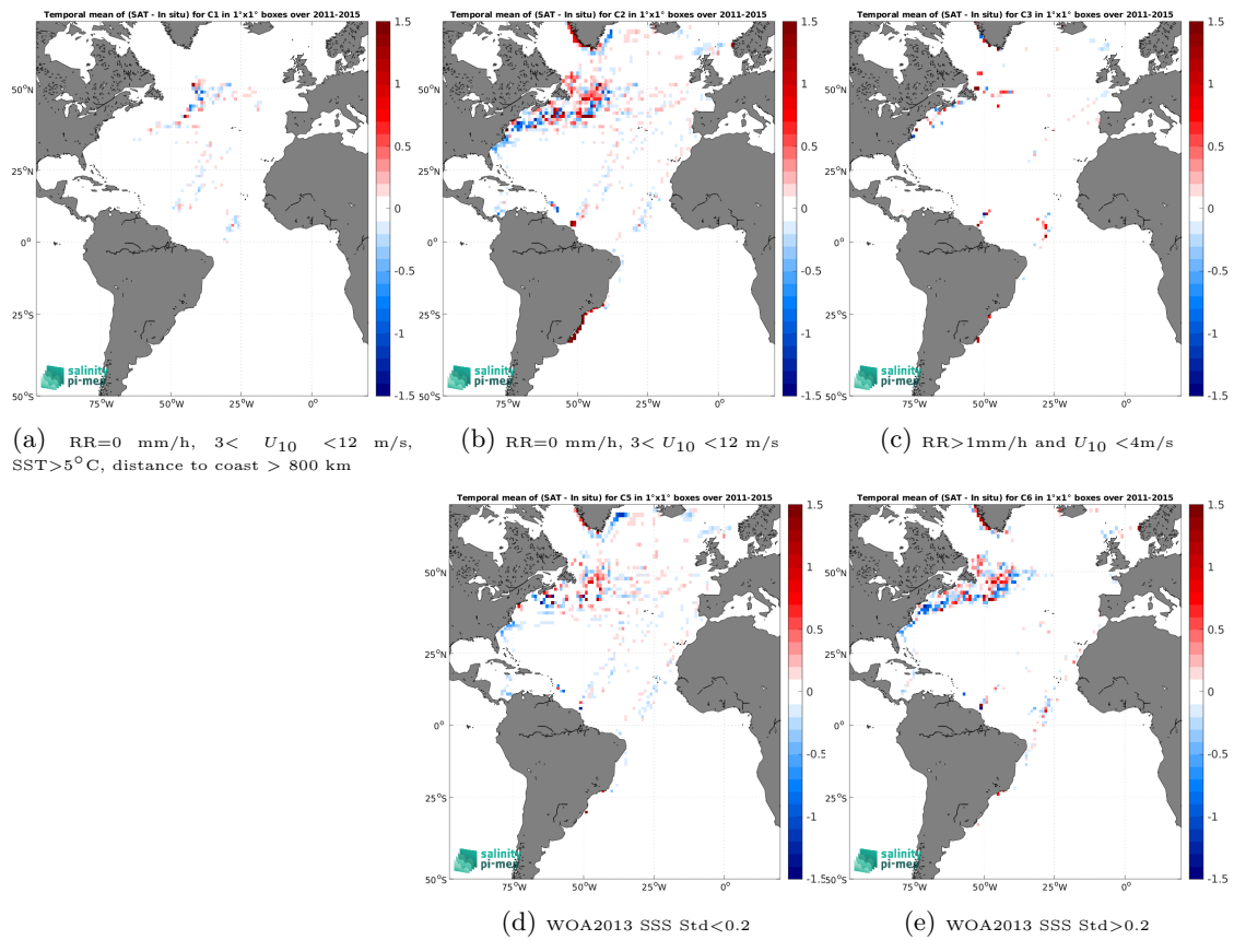
Figure 14: Temporal mean gridded over spatial boxes of size 1^\circ \times 1^\circ of \Delta\text{SSS} (Aquarius SSS L4 OI v5 - Monthly (IPRC) - TSG (LEGOS-DM)) for 5 different subdatasets corresponding to:RR=0 mm/h, 3 < U_{10} < 12 m/s, SST >5^\circ\text{C} , distance to coast > 800 km (a), RR=0 mm/h, 3 < U_{10} < 12 m/s (b), RR >1 mm/h and U_{10} < 4 m/s (c), WOA2013 SSS Std <0.2 (d), WOA2013 SSS Std >0.2 (e).
