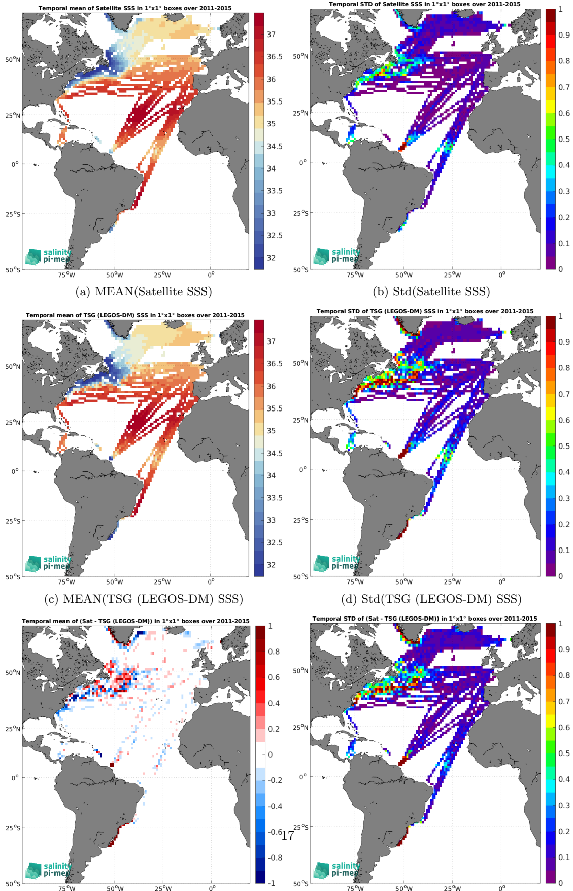
(e) MEAN( \Delta SSS) (Satellite - TSG (LEGOS-DM)) (f) Std( \Delta SSS) (Satellite - TSG (LEGOS-DM)) Figure 7: Temporal mean (left) and Std (right) of SSS from Aquarius SSS L4 OI v5 - Monthly (IPRC) (top), TSG (LEGOS-DM) (middle), and of \Delta SSS (Satellite - TSG (LEGOS-DM)). Only match-up pairs are used to generate these maps.
