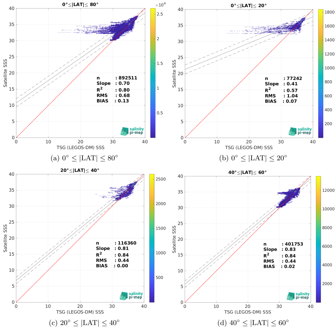
Figure 10: Contour maps of the concentration of Aquarius SSS L4 OI v5 - Monthly (IPRC) SSS (y-axis) versus TSG (LEGOS-DM) SSS (x-axis) at match-up pairs for different latitude bands. For each plot, the red line shows x=y . The black thin and dashed lines indicate a linear fit through the data cloud and the \pm 95\% confidence levels, respectively. The number match-up pairs n , the slope and R^2 coefficient of the linear fit, the root mean square (RMS) and the mean bias between satellite and in situ data are indicated for each latitude band in each plots.
