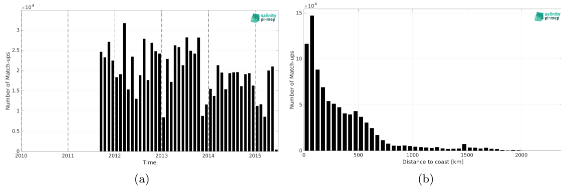
Figure 2: Number of match-ups between TSG (LEGOS-DM) and Aquarius SSS L4 OI v5 - Monthly (IPRC) SSS as a function of time (a) and as function of the distance to coast (b) over the Atlantic Ocean Pi-MEP region and for the full satellite product period.
