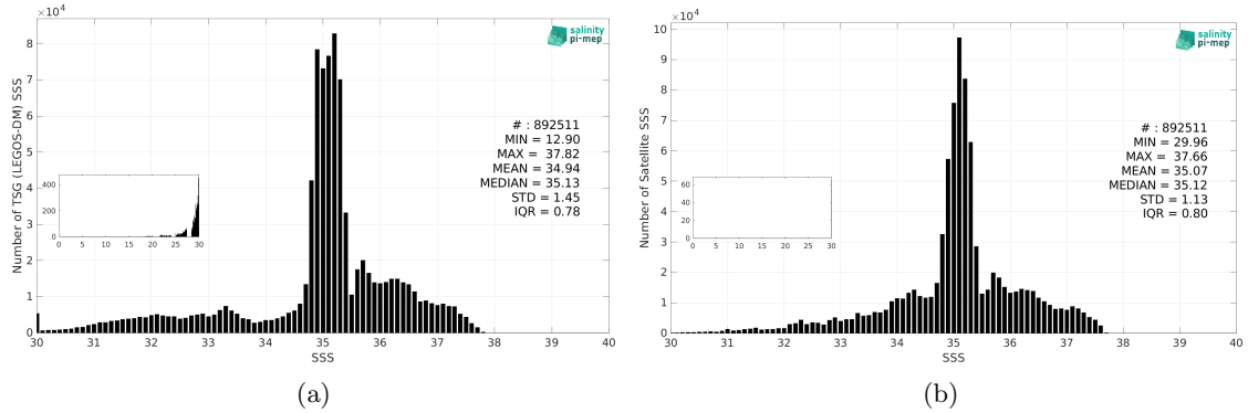
Figure 3: Histograms of SSS from TSG (LEGOS-DM) (a) and Aquarius SSS L4 OI v5 - Monthly (IPRC) (b) considering all match-up pairs per bins of 0.1 over the Atlantic Ocean Pi-MEP region and for the full satellite product period.
