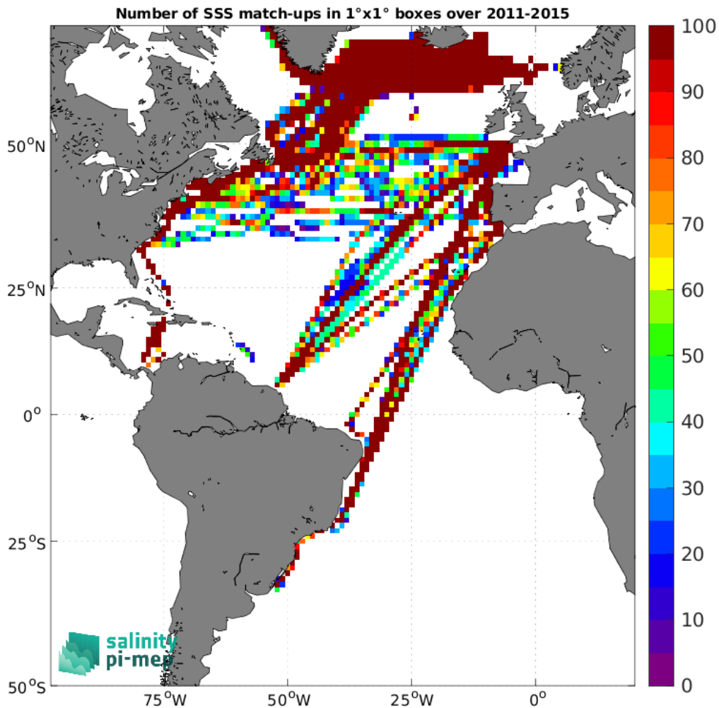
Figure 5: Number of SSS match-ups between TSG (LEGOS-DM) SSS and the Aquarius SSS L4 OI v5 - Monthly (IPRC) SSS product for the Atlantic Ocean Pi-MEP region over 1^\circ \times 1^\circ boxes and for the full satellite product period.
