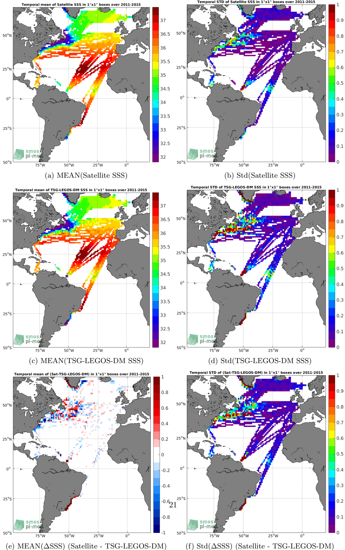
(e) MEAN( \Delta SSS) (Satellite - TSG-LEGOS-DM) (f) Std( \Delta SSS) (Satellite - TSG-LEGOS-DM) Figure 6: Temporal mean (left) and Std (right) of SSS from Aquarius-L4-IPRC-V5-MONTHLY (top), TSG-LEGOS-DM (middle), and of \Delta SSS (Satellite - TSG-LEGOS-DM). Only match-up pairs are used to generate these maps.
