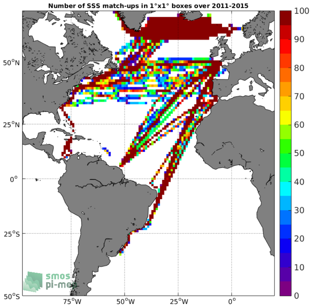
Figure 4: Number of SSS match-ups between TSG-LEGOS-DM SSS and the Aquarius-L4-IPRC-V5-MONTHLY SSS product for the Atlantic Ocean Pi-MEP region over 1°x1° boxes and for the full satellite product period.
