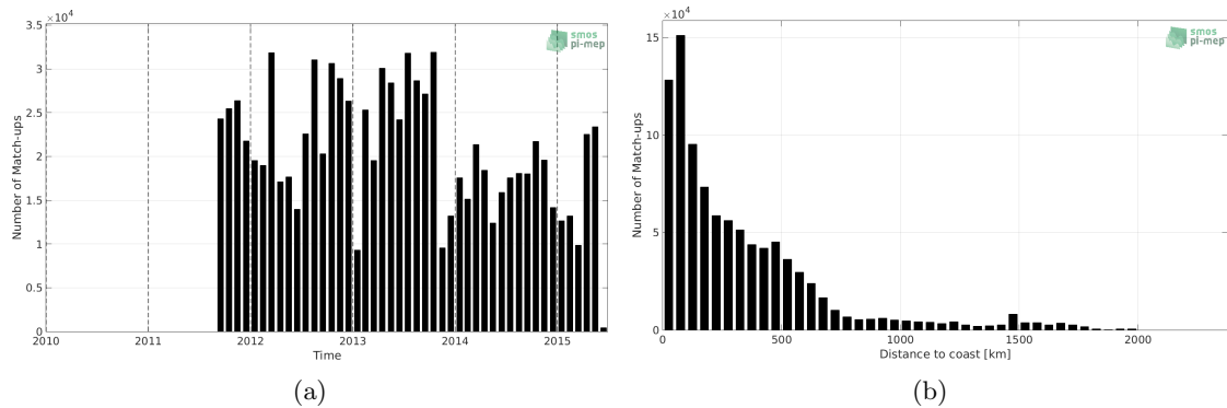
Figure 1: Number of match-ups between TSG-LEGOS-DM and Aquarius-L4-IPRC-V5-MONTHLY SSS as a function of time (a) and as function of the distance to coast (b) over the Atlantic Ocean Pi-MEP region and for the full satellite product period.
