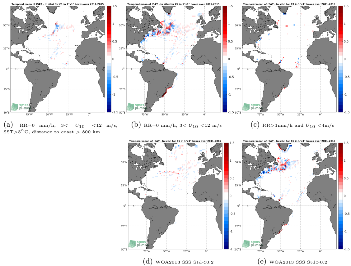
Figure 12: Temporal mean gridded over spatial boxes of size 1^\circ \times 1^\circ of \Delta SSS (Aquarius-L4-IPRC-V5-MONTHLY - TSG-LEGOS-DM) for 5 different subdatasets corresponding to:RR=0 mm/h, 3 < U_{10} < 12 m/s, SST >5^\circ C, distance to coast > 800 km (a), RR=0 mm/h, 3 < U_{10} < 12 m/s (b), RR >1 mm/h and U_{10} < 4 m/s (c), WOA2013 SSS Std <0.2 (d), WOA2013 SSS Std >0.2 (e).
