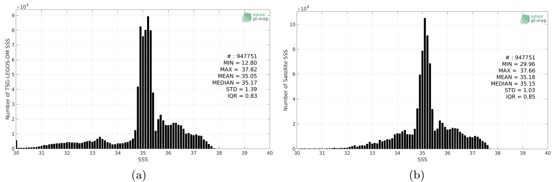
Figure 2: Histograms of SSS from TSG-LEGOS-DM (a) and Aquarius-L4-IPRC-V5-MONTHLY (b) considering all match-up pairs per bins of 0.1 over the Atlantic Ocean Pi-MEP region and for the full satellite product period.
