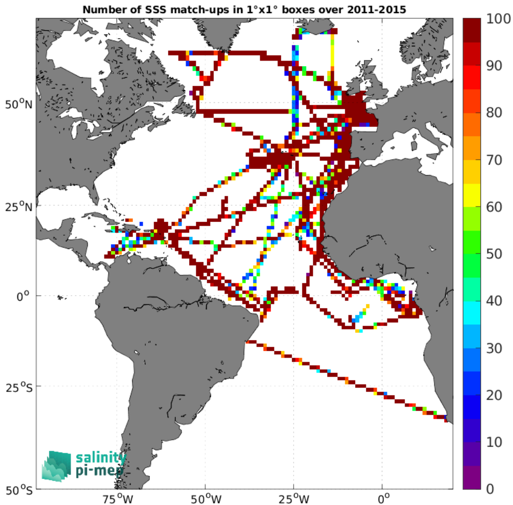
Figure 5: Number of SSS match-ups between TSG (GOSUD-Research-vessel) SSS and the Aquarius SSS L4 OI v5 - Monthly (IPRC) SSS product for the Atlantic Ocean Pi-MEP region over 1^\circ \times 1^\circ boxes and for the full satellite product period.
