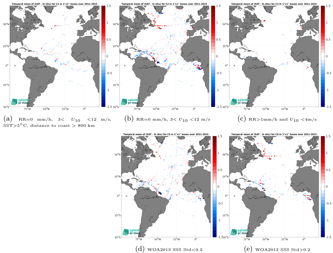
Figure 14: Temporal mean gridded over spatial boxes of size 1^\circ \times 1^\circ of \Delta\text{SSS} (Aquarius SSS L4 OI v5 - Monthly (IPRC) - TSG (GOSUD-Research-vessel)) for 5 different subdatasets corresponding to:RR=0 mm/h, 3 < U_{10} < 12 m/s, SST >5^\circ\text{C} , distance to coast > 800 km (a), RR=0 mm/h, 3 < U_{10} < 12 m/s (b), RR >1 mm/h and U_{10} < 4 m/s (c), WOA2013 SSS Std <0.2 (d), WOA2013 SSS Std >0.2 (e).
