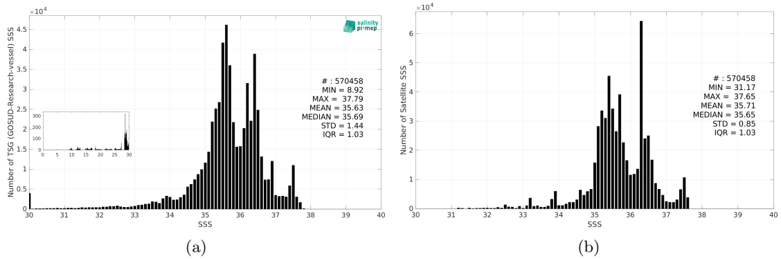
Figure 3: Histograms of SSS from TSG (GOSUD-Research-vessel) (a) and Aquarius SSS L4 OI v5 - Monthly (IPRC) (b) considering all match-up pairs per bins of 0.1 over the Atlantic Ocean Pi-MEP region and for the full satellite product period.
