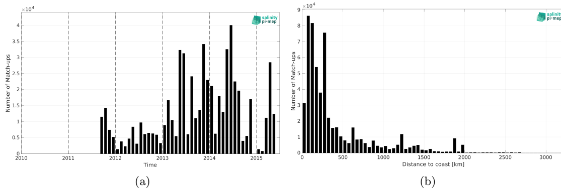
Figure 2: Number of match-ups between TSG (GOSUD-Research-vessel) and Aquarius SSS L4 OI v5 - Monthly (IPRC) SSS as a function of time (a) and as function of the distance to coast (b) over the Atlantic Ocean Pi-MEP region and for the full satellite product period.
