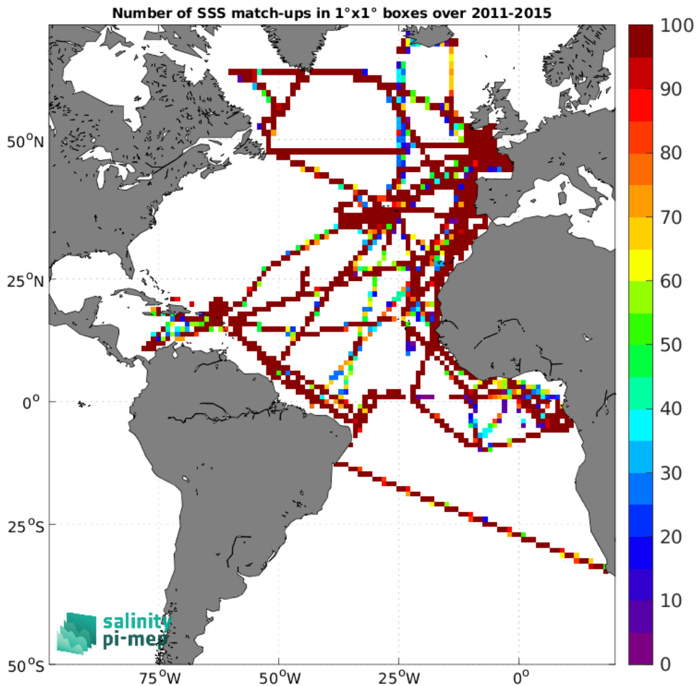
Figure 4: Number of SSS match-ups between TSG (GOSUD-Research-vessel) SSS and the Aquarius SSS L4 OI v5 - Monthly (IPRC) SSS product for the Atlantic Ocean Pi-MEP region over 1^{\circ} \times 1^{\circ} boxes and for the full satellite product period.
