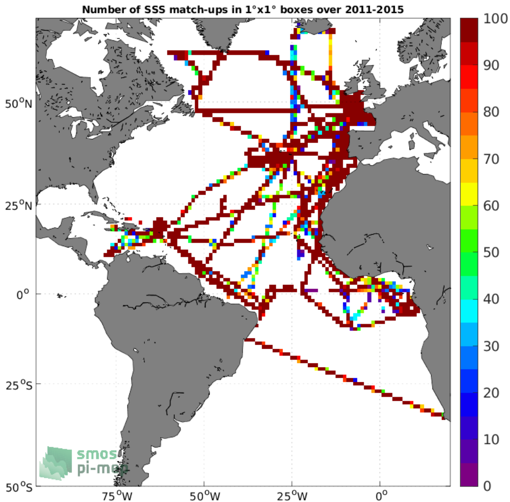
Figure 4: Number of SSS match-ups between TSG (GOSUD-Research-vessel) SSS and the Aquarius SSS L4 OI v5 - Monthly (IPRC) SSS product for the Atlantic Ocean Pi-MEP region over 1°×1° boxes and for the full satellite product period.
