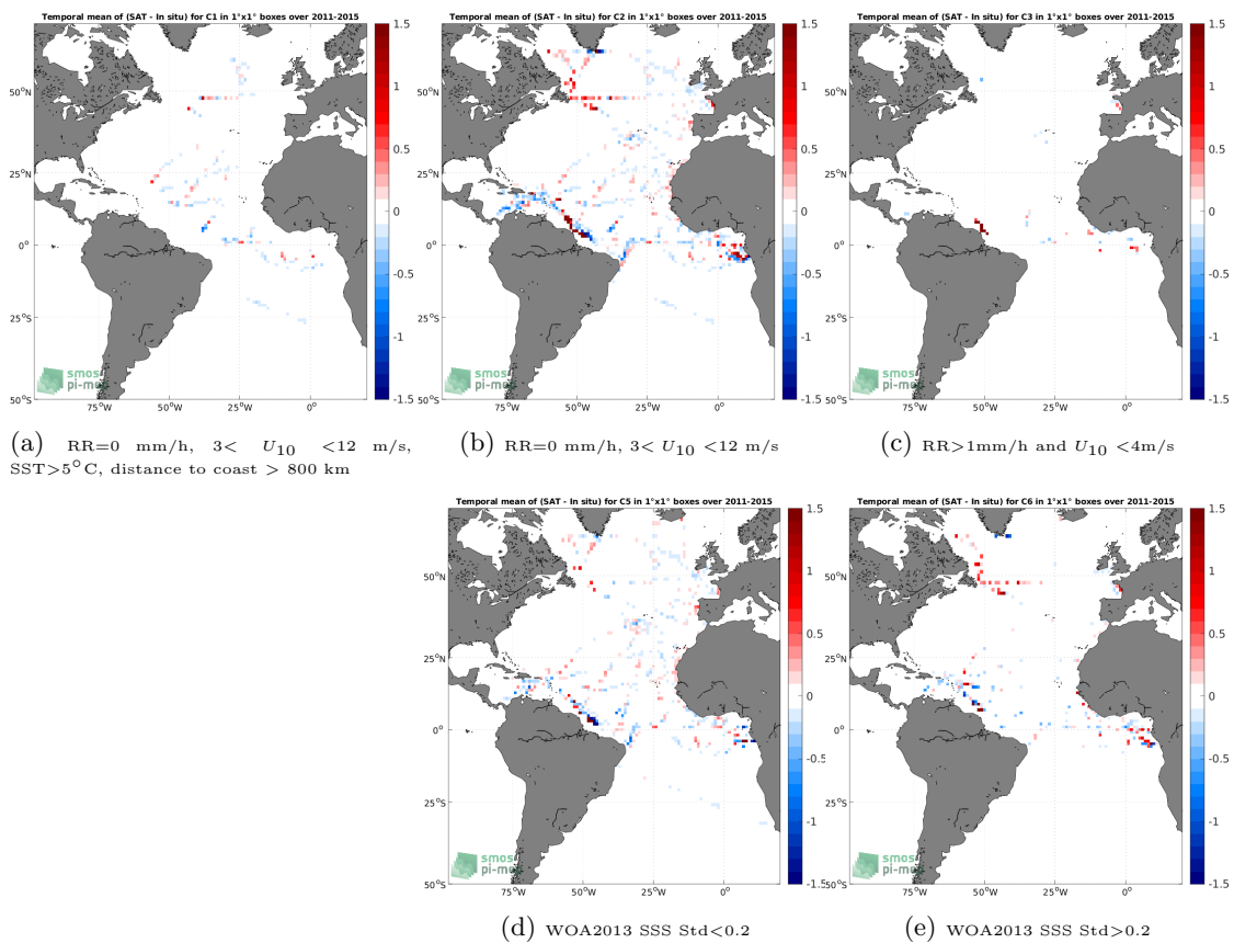
Figure 12: Temporal mean gridded over spatial boxes of size 1^\circ \times 1^\circ of \Delta\text{SSS} (Aquarius SSS L4 OI v5 - Monthly (IPRC) - TSG (GOSUD-Research-vessel)) for 5 different subdatasets corresponding to:RR=0 mm/h, 3 < U_{10} < 12 m/s, SST>5°C, distance to coast > 800 km (a), RR=0 mm/h, 3 < U_{10} < 12 m/s (b), RR>1mm/h and U_{10} < 4 m/s (c), WOA2013 SSS Std<0.2 (d), WOA2013 SSS Std>0.2 (e).
