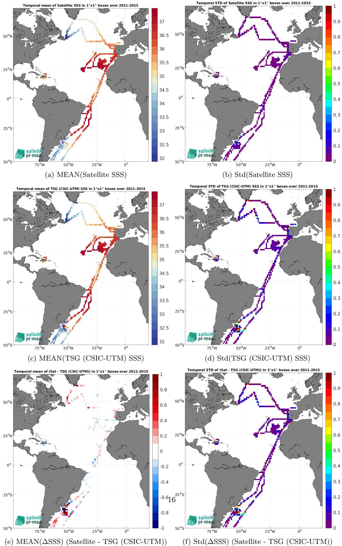
Figure 7: Temporal mean (left) and Std (right) of SSS from Aquarius SSS L4 OI v5 - Monthly (IPRC) (top), TSG (CSIC-UTM) (middle), and of \Delta SSS (Satellite - TSG (CSIC-UTM)). Only match-up pairs are used to generate these maps.
