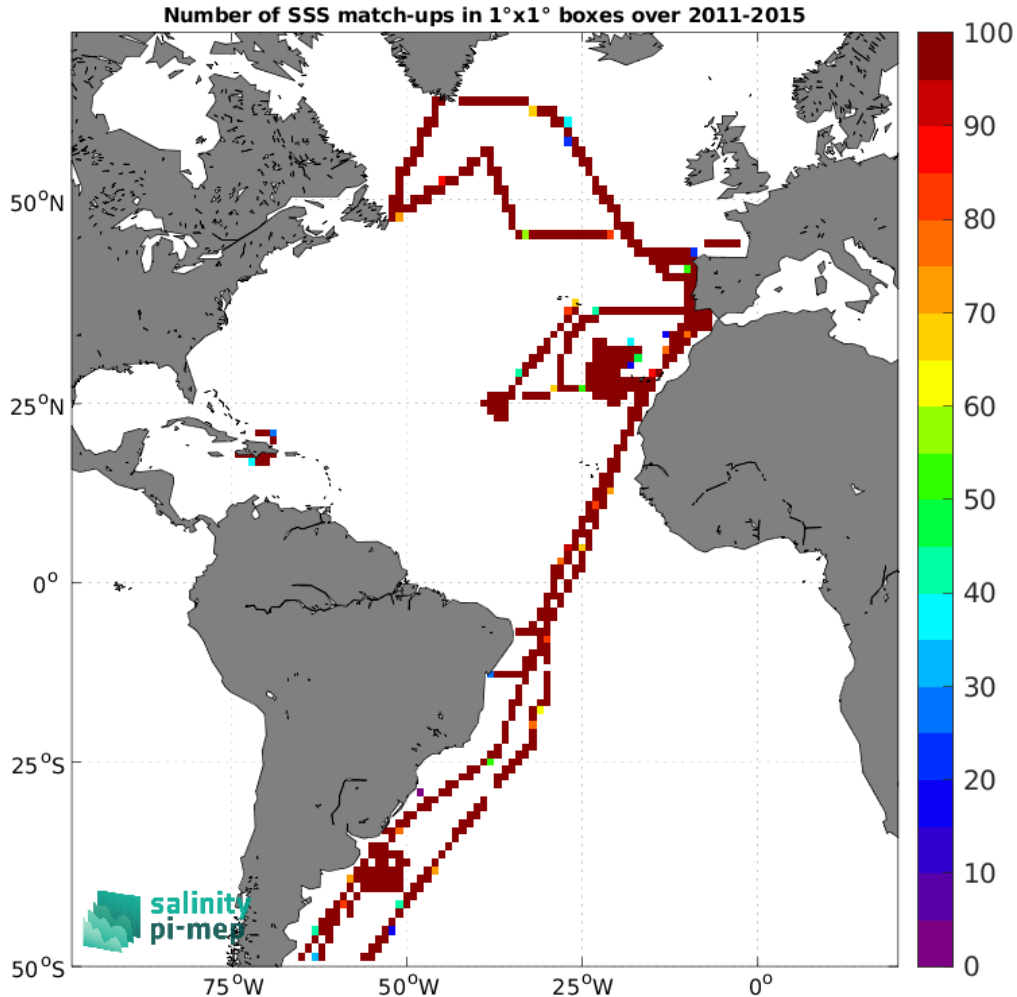
Figure 5: Number of SSS match-ups between TSG (CSIC-UTM) SSS and the Aquarius SSS L4 OI v5 - Monthly (IPRC) SSS product for the Atlantic Ocean Pi-MEP region over 1^\circ \times 1^\circ boxes and for the full satellite product period.
