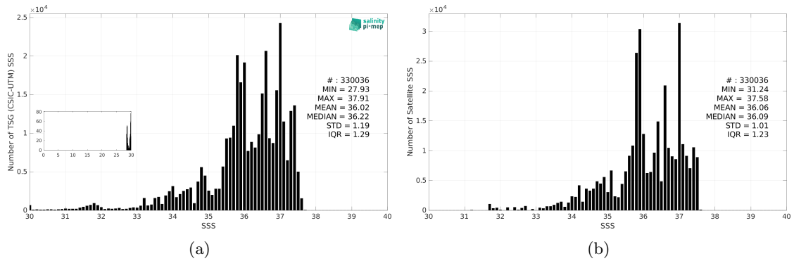
Figure 3: Histograms of SSS from TSG (CSIC-UTM) (a) and Aquarius SSS L4 OI v5 - Monthly (IPRC) (b) considering all match-up pairs per bins of 0.1 over the Atlantic Ocean Pi-MEP region and for the full satellite product period.
