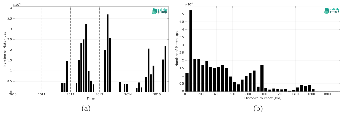
Figure 2: Number of match-ups between TSG (CSIC-UTM) and Aquarius SSS L4 OI v5 - Monthly (IPRC) SSS as a function of time (a) and as function of the distance to coast (b) over the Atlantic Ocean Pi-MEP region and for the full satellite product period.
