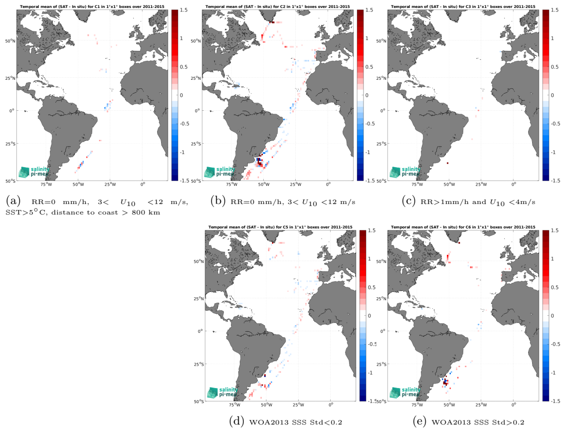
Figure 14: Temporal mean gridded over spatial boxes of size 1^\circ \times 1^\circ of \Delta\text{SSS} (Aquarius SSS L4 OI v5 - Monthly (IPRC) - TSG (CSIC-UTM)) for 5 different subdatasets corresponding to:RR=0 mm/h, 3 < U_{10} < 12 m/s, SST>5°C, distance to coast > 800 km (a), RR=0 mm/h, 3 < U_{10} < 12 m/s (b), RR>1mm/h and U_{10} < 4 m/s (c), WOA2013 SSS Std<0.2 (d), WOA2013 SSS Std>0.2 (e).
