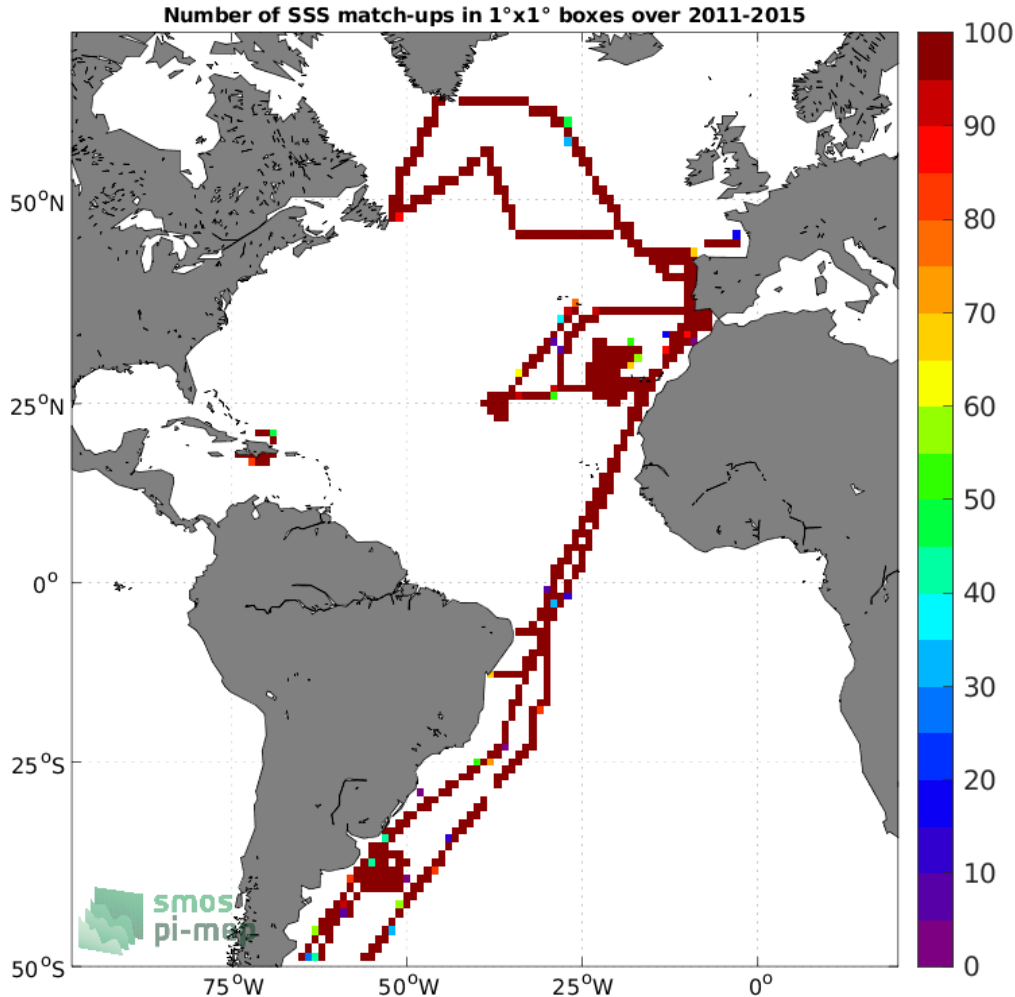
Figure 4: Number of SSS match-ups between TSG (CSIC-UTM) SSS and the Aquarius SSS L4 OI v5 - Monthly (IPRC) SSS product for the Atlantic Ocean Pi-MEP region over 1^\circ \times 1^\circ boxes and for the full satellite product period.
