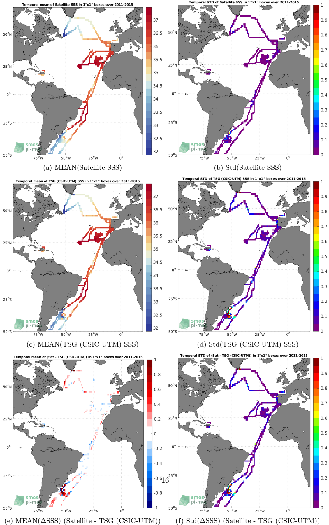
Figure 6: Temporal mean (left) and Std (right) of SSS from Aquarius SSS L4 OI v5 - Monthly (IPRC) (top), TSG (CSIC-UTM) (middle), and of \Delta SSS (Satellite - TSG (CSIC-UTM)). Only match-up pairs are used to generate these maps.
