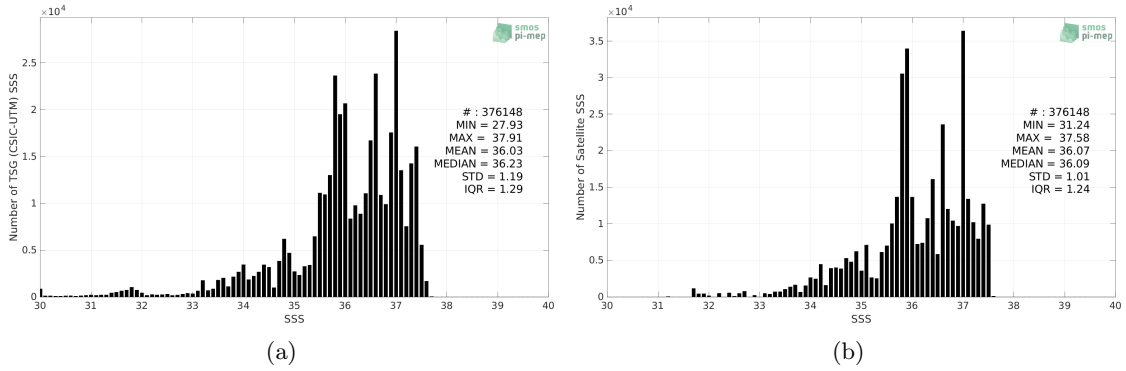
Figure 2: Histograms of SSS from TSG (CSIC-UTM) (a) and Aquarius SSS L4 OI v5 - Monthly (IPRC) (b) considering all match-up pairs per bins of 0.1 over the Atlantic Ocean Pi-MEP region and for the full satellite product period.
