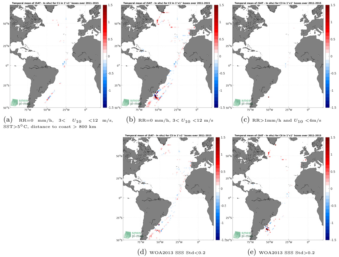
Figure 12: Temporal mean gridded over spatial boxes of size 1^\circ \times 1^\circ of \Delta SSS (Aquarius SSS L4 OI v5 - Monthly (IPRC) - TSG (CSIC-UTM)) for 5 different subdatasets corresponding to:RR=0 mm/h, 3 < U_{10} < 12 m/s, SST >5^\circ\text{C} , distance to coast > 800 km (a), RR=0 mm/h, 3 < U_{10} < 12 m/s (b), RR >1 mm/h and U_{10} < 4 m/s (c), WOA2013 SSS Std <0.2 (d), WOA2013 SSS Std >0.2 (e).
