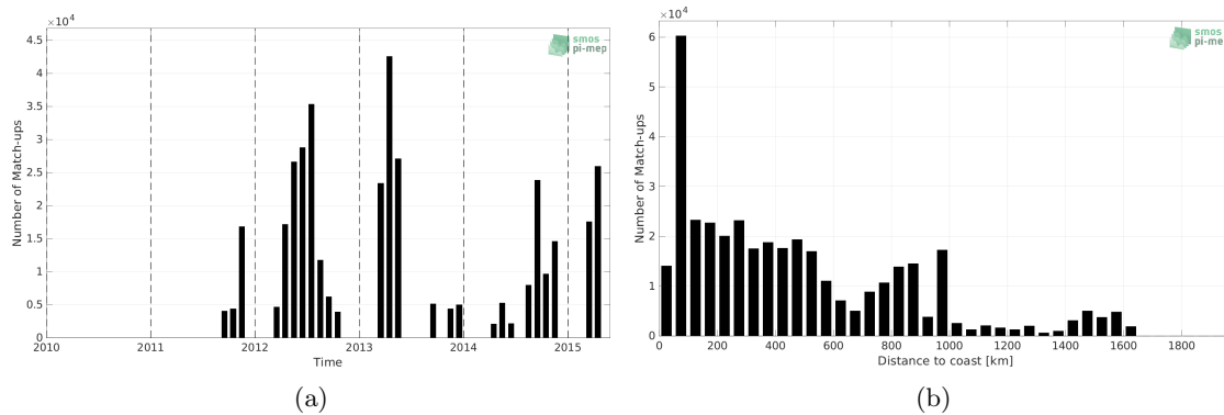
Figure 1: Number of match-ups between TSG (CSIC-UTM) and Aquarius SSS L4 OI v5 - Monthly (IPRC) SSS as a function of time (a) and as function of the distance to coast (b) over the Atlantic Ocean Pi-MEP region and for the full satellite product period.
