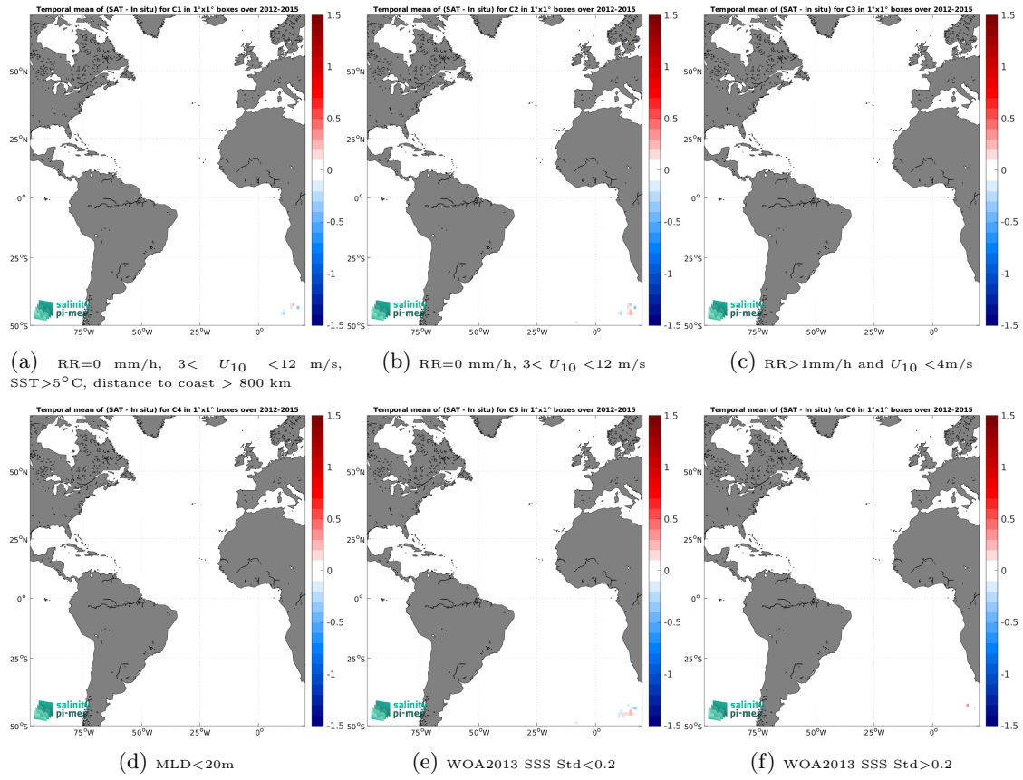
Figure 12: Temporal mean gridded over spatial boxes of size 1^{\circ} \times 1^{\circ} of \Delta SSS (Aquarius SSS L4 OI v5 - Monthly (IPRC) - Marine mammals) for 6 different subdatasets corresponding to: RR=0 mm/h, 3 < U_{10} < 12 m/s, SST > 5^{\circ}C , distance to coast > 800 km (a), RR=0 mm/h, 3 < U_{10} < 12 m/s (b), RR > 1 mm/h and U_{10} < 4 m/s (c), MLD < 20 m (d), WOA2013 SSS Std < 0.2 (e), WOA2013 SSS Std > 0.2 (f).
