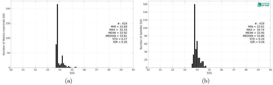
Figure 2: Histograms of SSS from Marine mammals (a) and Aquarius SSS L4 OI v5 - Monthly (IPRC) (b) considering all match-up pairs per bins of 0.1 over the Atlantic Ocean Pi-MEP region and for the full satellite product period.
