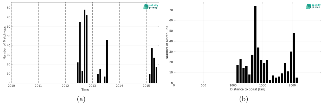
Figure 1: Number of match-ups between Marine mammals and Aquarius SSS L4 OI v5 - Monthly (IPRC) SSS as a function of time (a) and as function of the distance to coast (b) over the Atlantic Ocean Pi-MEP region and for the full satellite product period.
