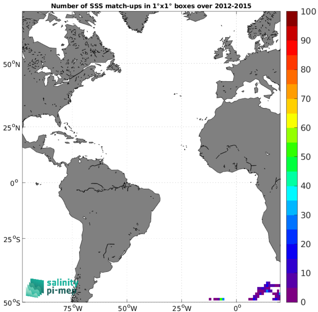
Figure 4: Number of SSS match-ups between Marine mammals SSS and the Aquarius SSS L4 OI v5 - Monthly (IPRC) SSS product for the Atlantic Ocean Pi-MEP region over 1^\circ \times 1^\circ boxes and for the full satellite product period.
