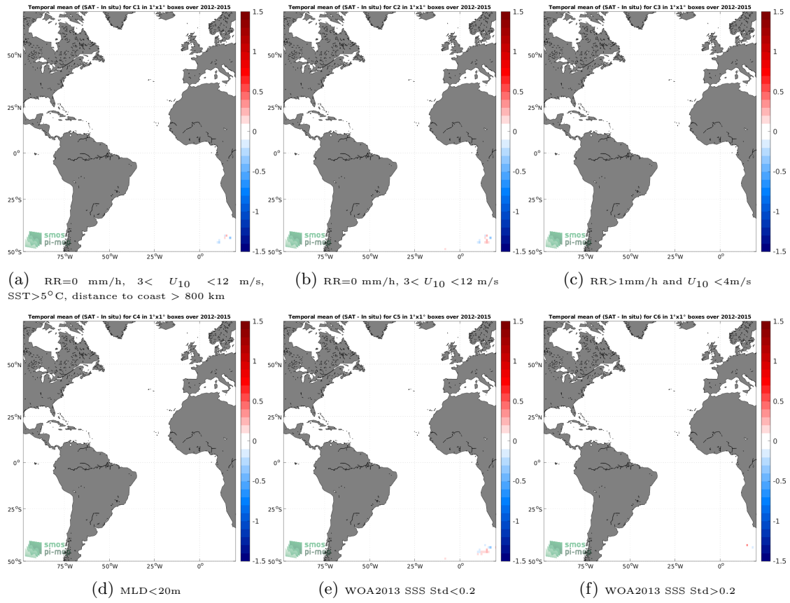
Figure 12: Temporal mean gridded over spatial boxes of size 1^\circ \times 1^\circ of \Delta\text{SSS} (Aquarius SSS L4 OI v5 - Monthly (IPRC) - Marine mammals) for 6 different subdatasets corresponding to: RR=0 mm/h, 3 < U_{10} < 12 m/s, SST > 5^\circ\text{C} , distance to coast > 800 km (a), RR=0 mm/h, 3 < U_{10} < 12 m/s (b), RR > 1 mm/h and U_{10} < 4 m/s (c), MLD < 20 m (d), WOA2013 SSS Std < 0.2 (e), WOA2013 SSS Std > 0.2 (f).
