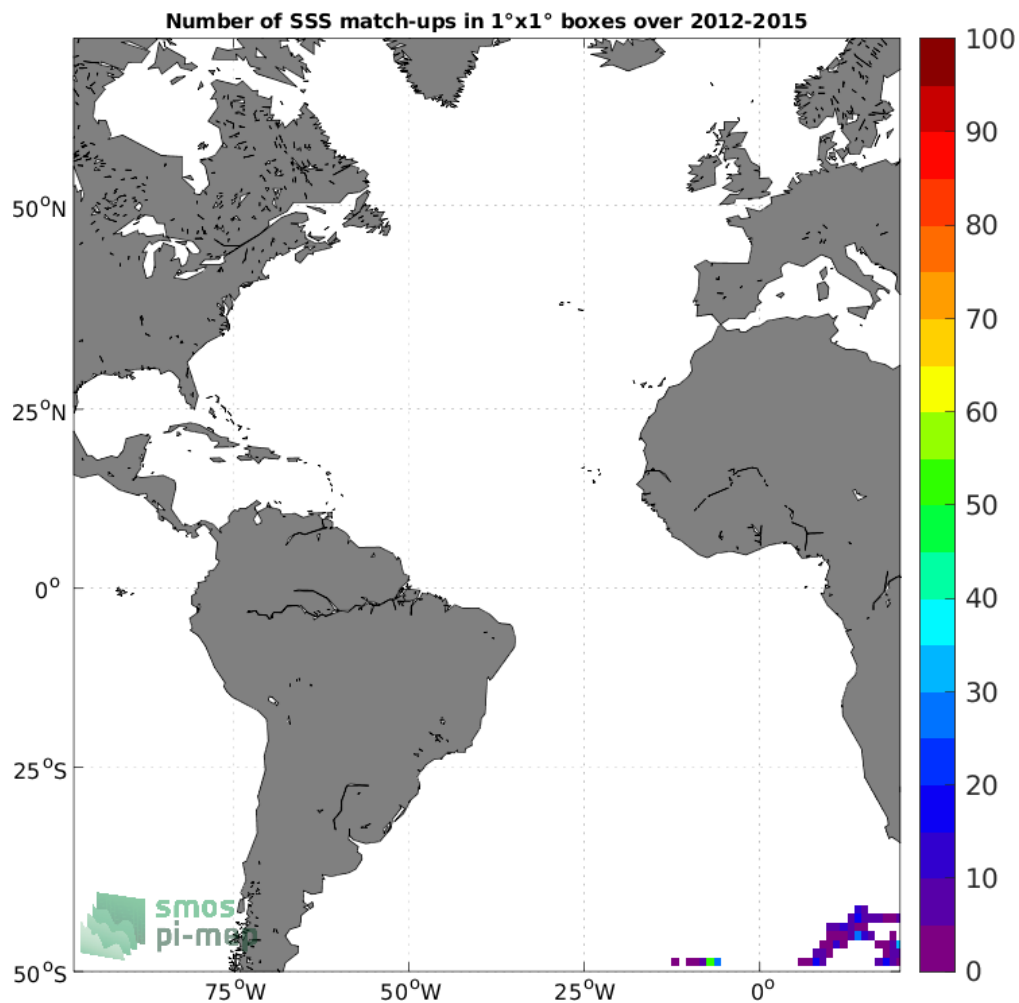
Figure 4: Number of SSS match-ups between Marine mammals SSS and the Aquarius SSS L4 OI v5 - Monthly (IPRC) SSS product for the Atlantic Ocean Pi-MEP region over 1°x1° boxes and for the full satellite product period.
